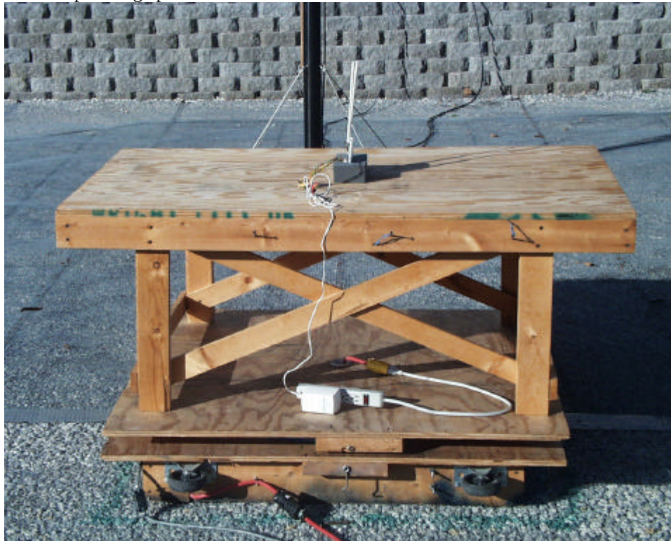
Test Setup Photographs for 1100 Wireless.
