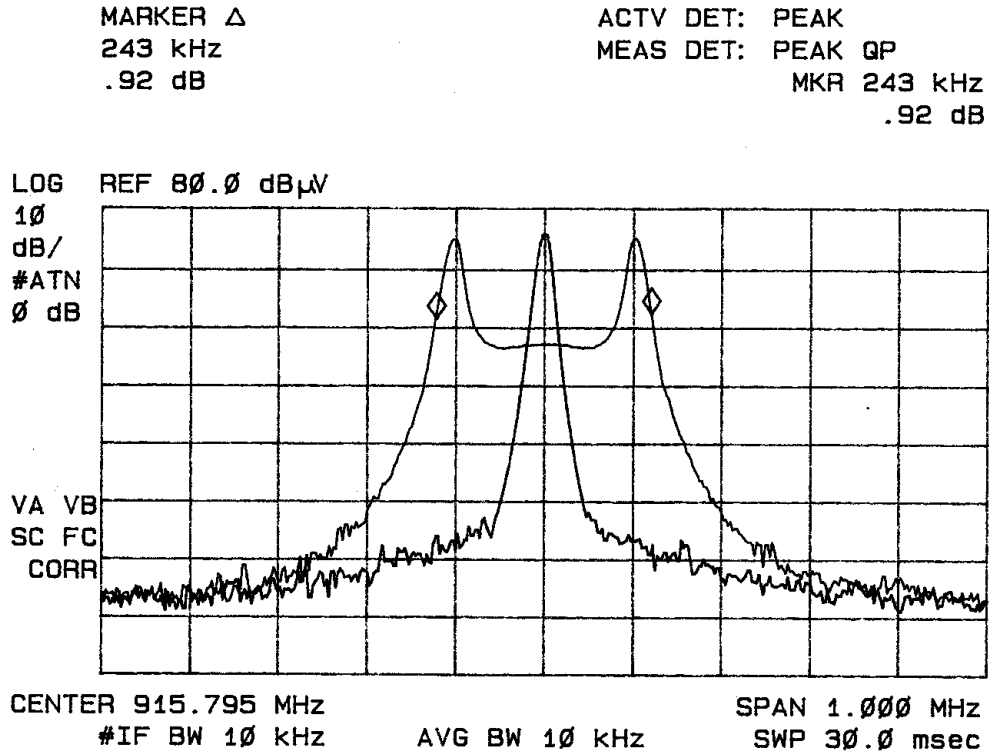
Figure nine 20-dB bandwidth.
