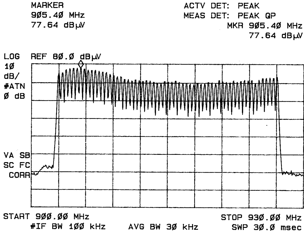
Figure eleven plot showing 61 hopping channels, (at least 50 hopping channels required).
