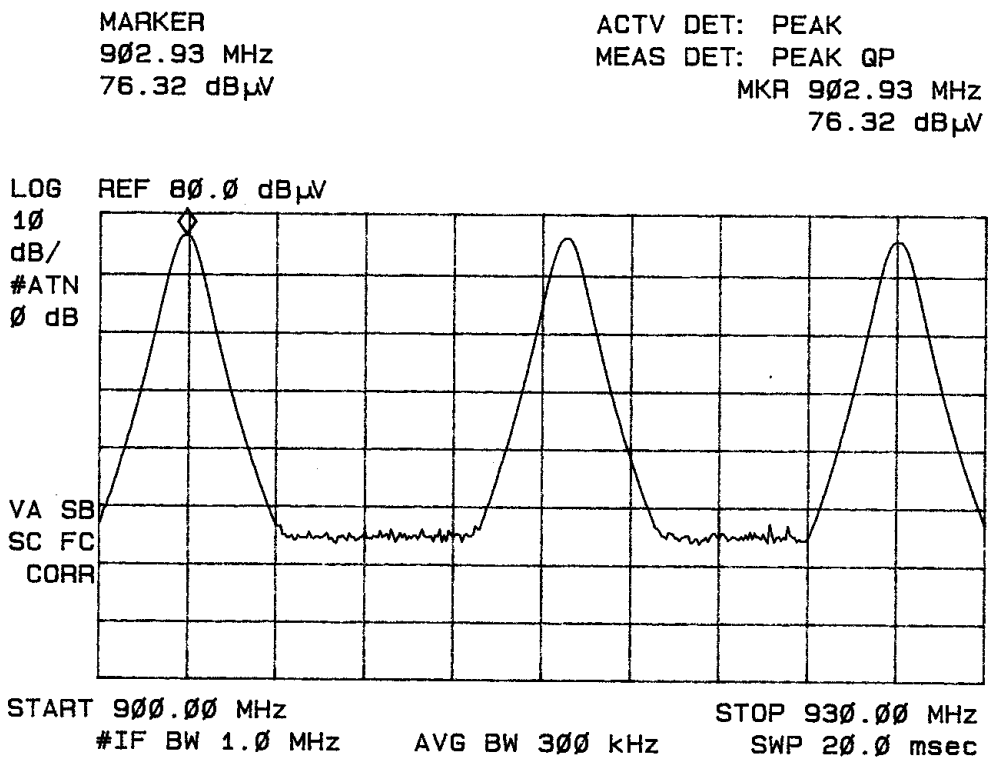
Figure eight Maximum Power output across band (taken in screen room at 1 meter).
