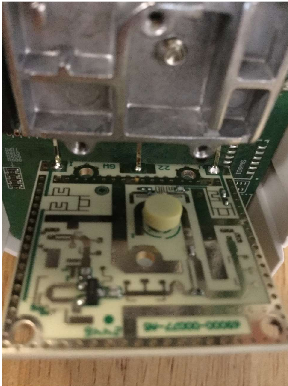
Microwave Detector Internal Components
