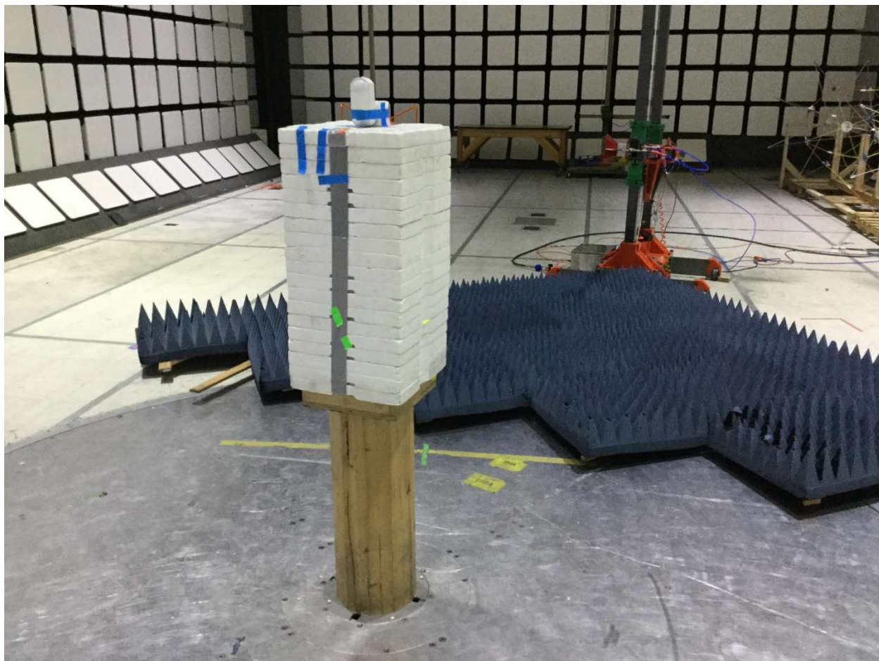
Setup, 1GHz – 18GHz
