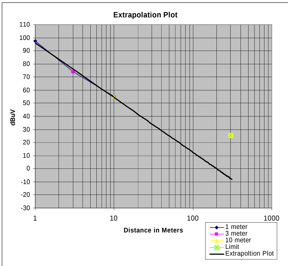
Figure ten Extrapolated Radiated Emissions data.
