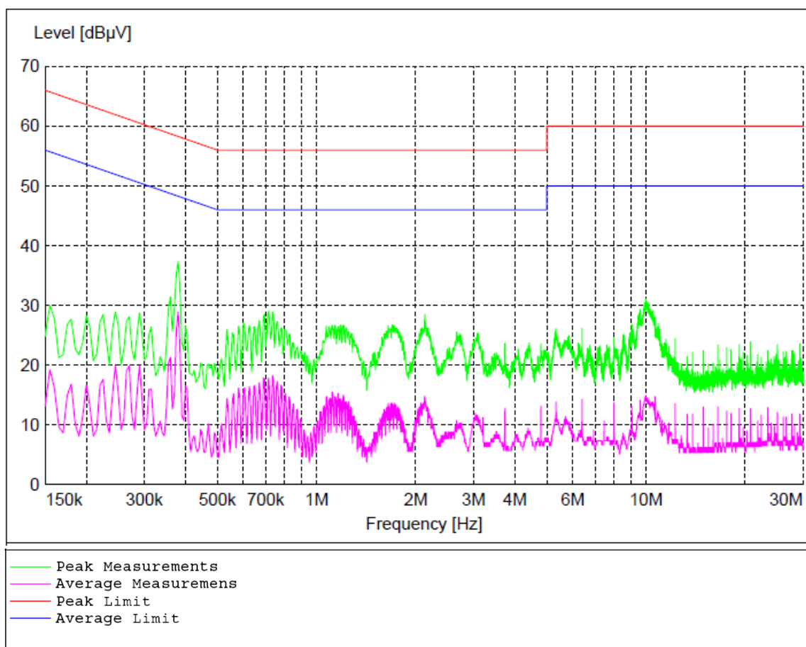
Figure 20 - Conducted Emissions Plot
