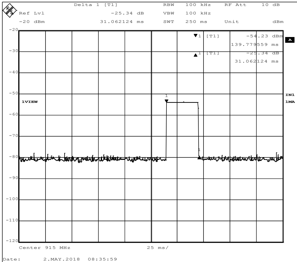
Figure 2 – Duty Cycle
