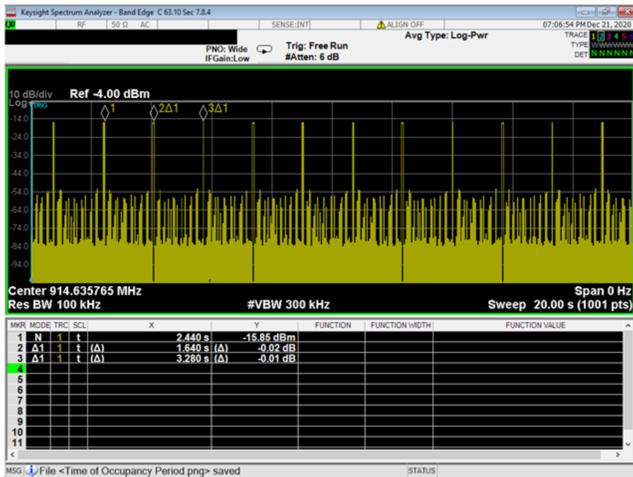
Figure 22 – Period, 1.6 sec.
