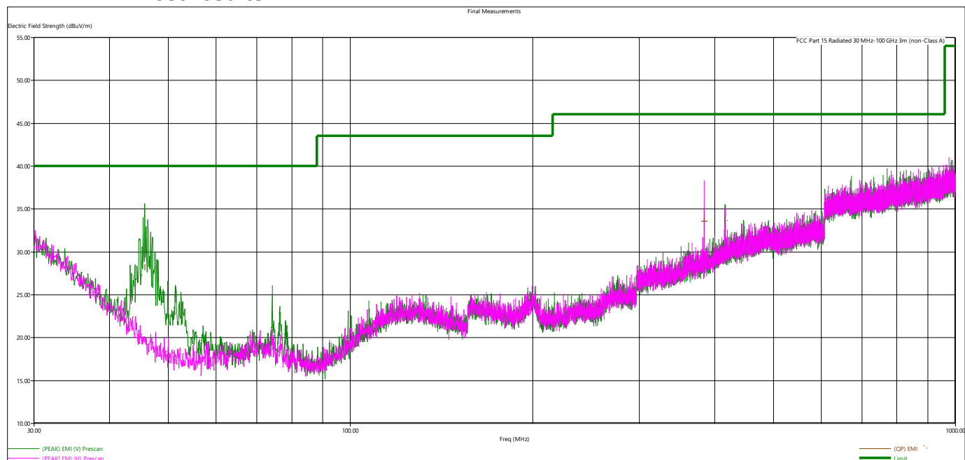
Figure 2 - Radiated Emissions Plot, 30 MHz-1 GHz, Receive Mode
