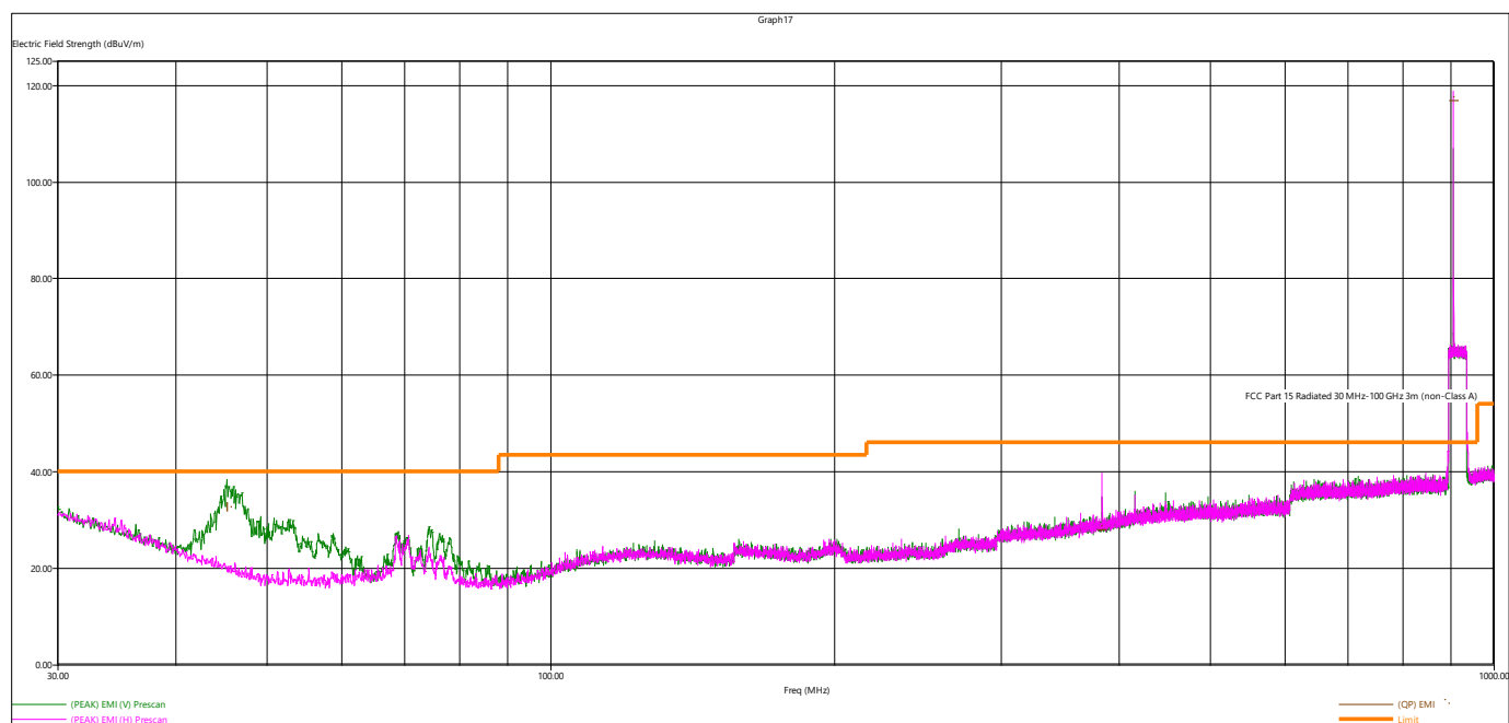
Figure 3 - Radiated Emissions Plot, 30 MHz-1 GHz Low Channel
