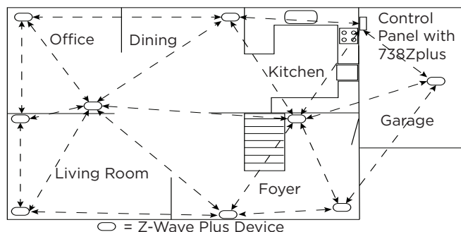
Figure 2: Example Z-Wave Plus Transmission Routes
