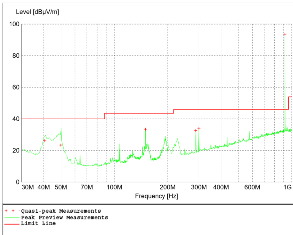
Figure 6 - Radiated Emissions Plot, 916 MHz
