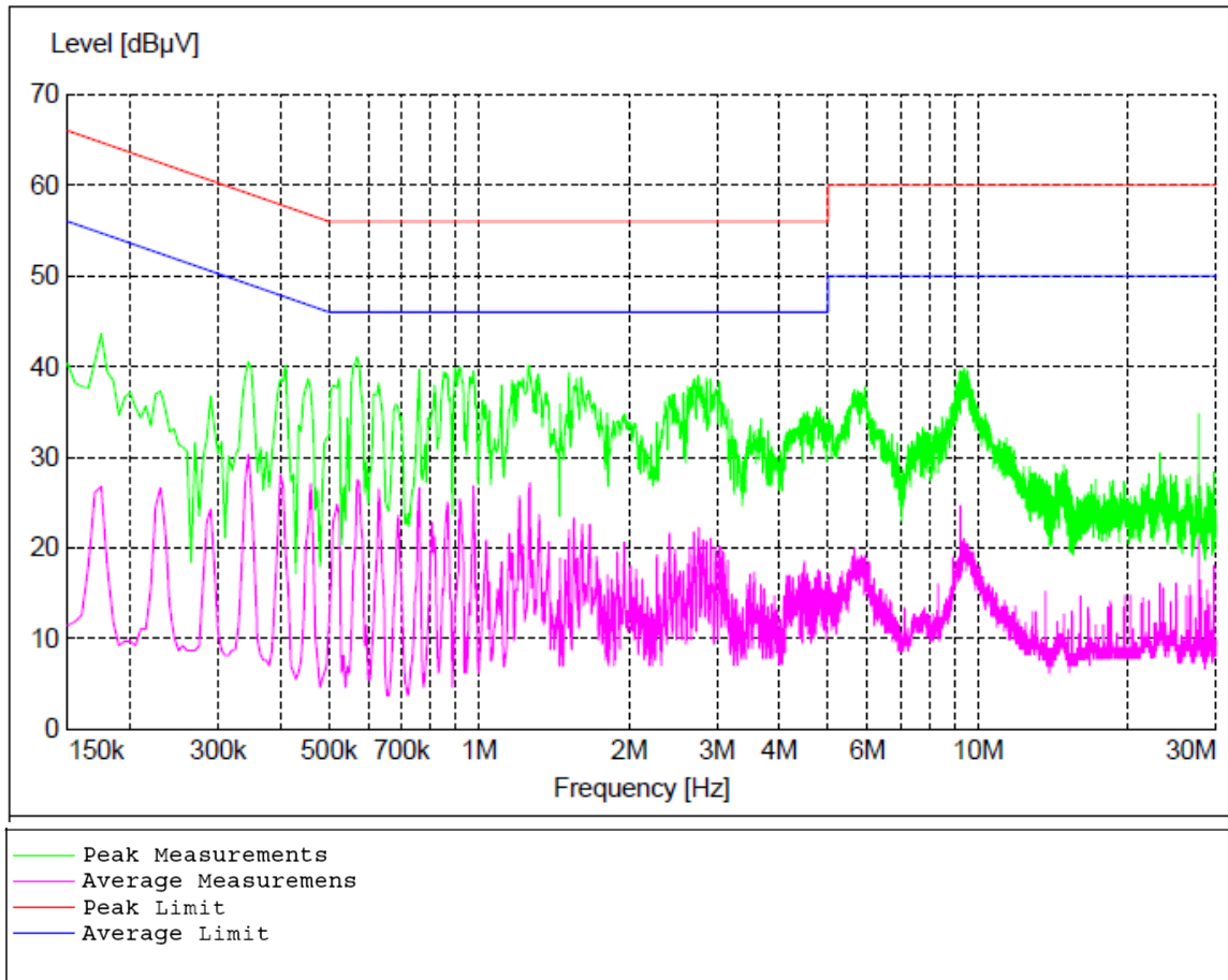
Figure 14 - Conducted Emissions Plot
