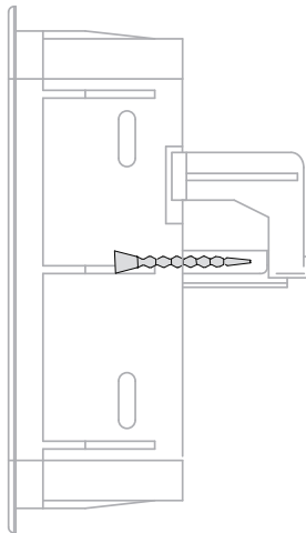
Figure 8: Screw Locations
