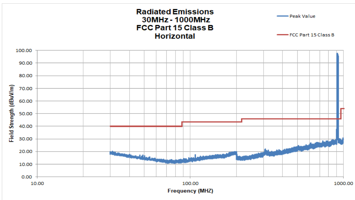
Figure 2. Intentional Radiator, Radiated Emissions Horizontal, 30 MHz – 1000 MHz
