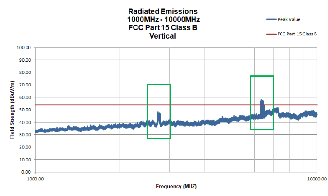
Figure 5. Intentional Radiator, Radiated Emissions Vertical, 1 GHz – 10 GHz
