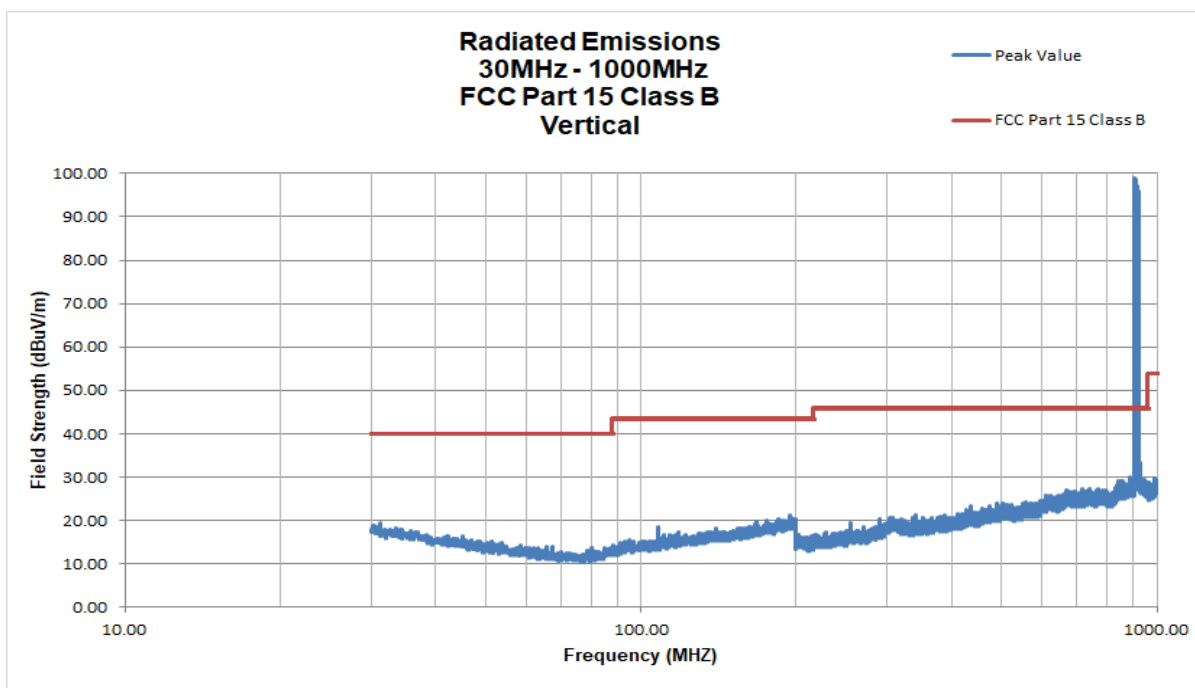
Figure 3. Intentional Radiator, Radiated Emissions Vertical, 30 MHz – 1000 MHz
