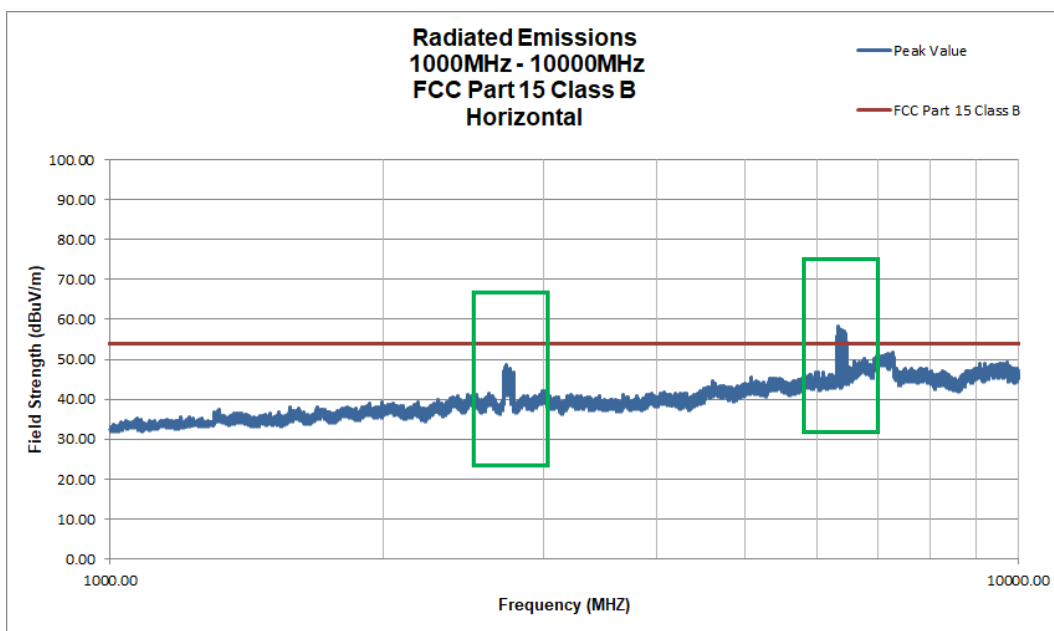
Figure 4. Intentional Radiator, Radiated Emissions Horizontal, 1 GHz – 10 GHz
