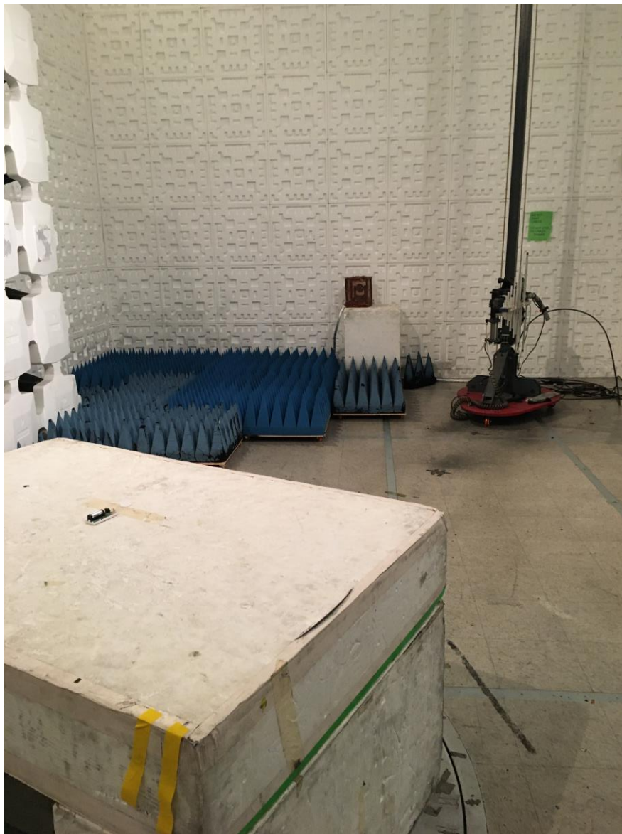
Figure 2. Radiated Emissions Test Setup 200 - 1000 MHz
