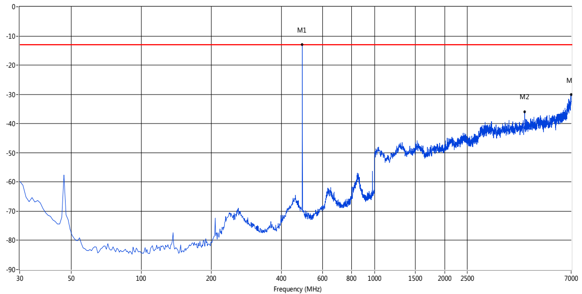
Figure 5: TX Spurious Radiation, 30 – 7000 MHz, Horizontal (Middle CH)
