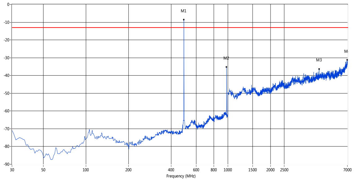
Figure 4: TX Spurious Radiation, 30 – 7000 MHz, Vertical (Middle CH)
