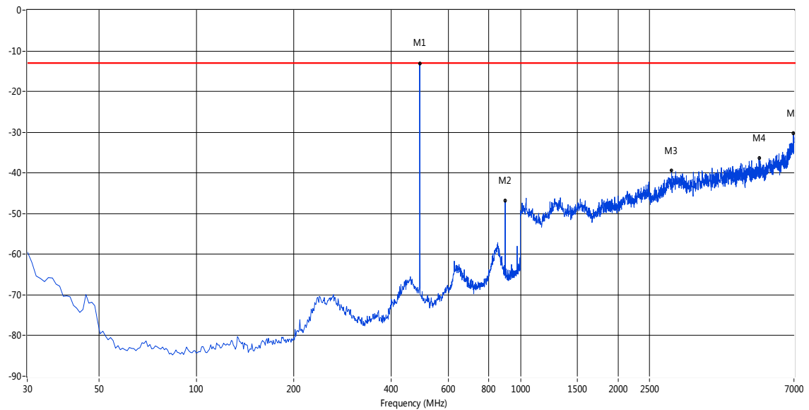
Figure 3: TX Spurious Radiation, 30 – 7000 MHz, Horizontal (Low CH)
