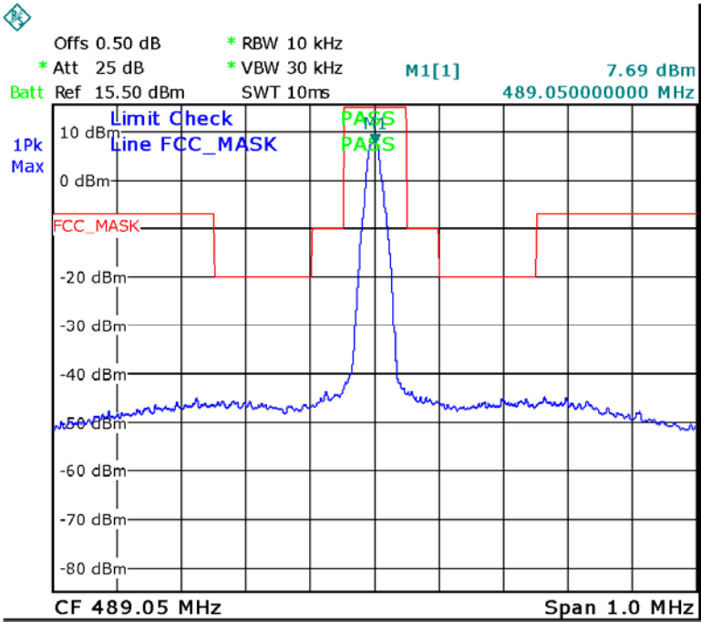
Emission Mask Middle Channel
