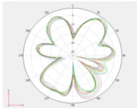
Radiation Pattern @1950mhZ
