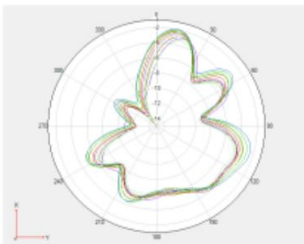
Radiation Pattern @1950mhZ
