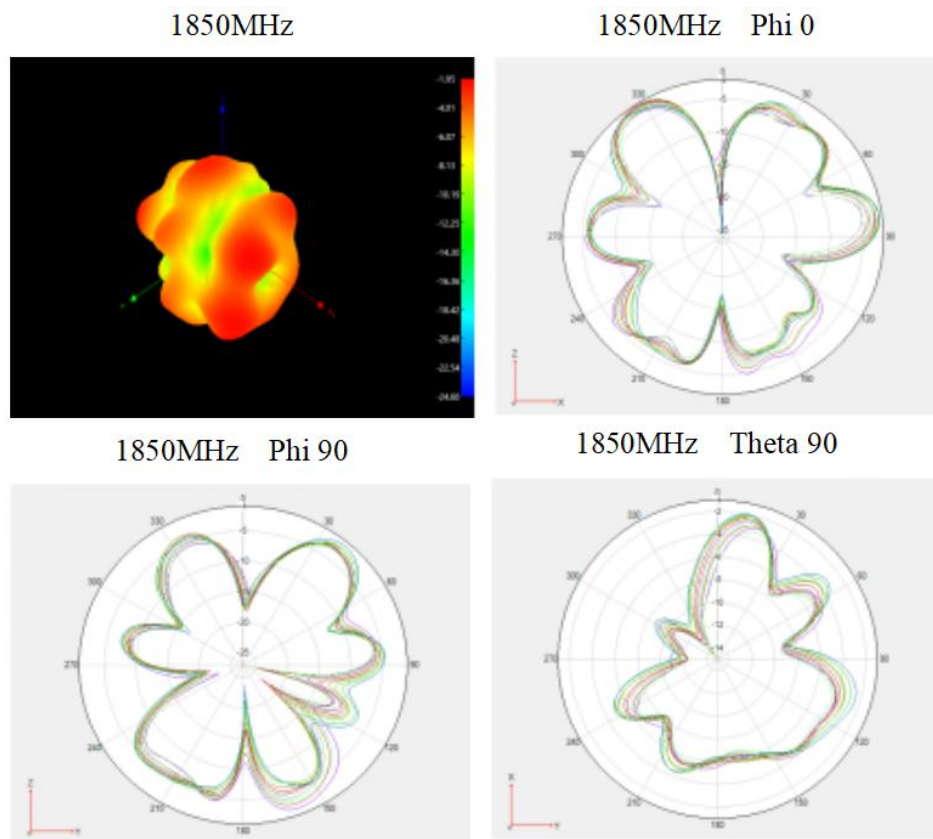
Radiation Pattern @1850mhZ
