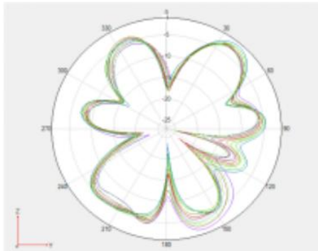
Radiation Pattern @1900mhZ
