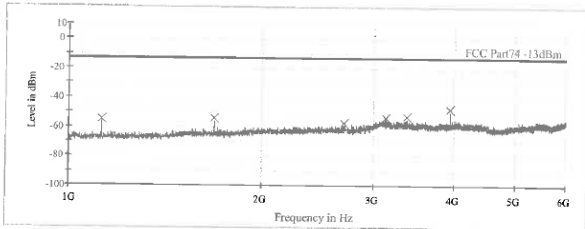
Figure 13: TX Spurious Radiation, Above 1GHz, Vertical (CH288, High CH)
