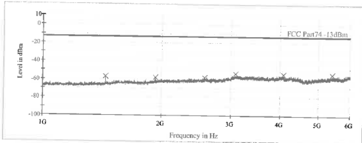
Figure 9: TX Spurious Radiation, Above 1GHz, Vertical (CH288, Low CH)
