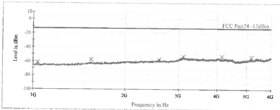
Figure 10: TX Spurious Radiation, Above 1GHz, Horizontal (CH288, Middle CH)
