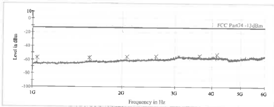
Figure 11: TX Spurious Radiation, Above 1GHz, Vertical (CH288, Middle CH)
