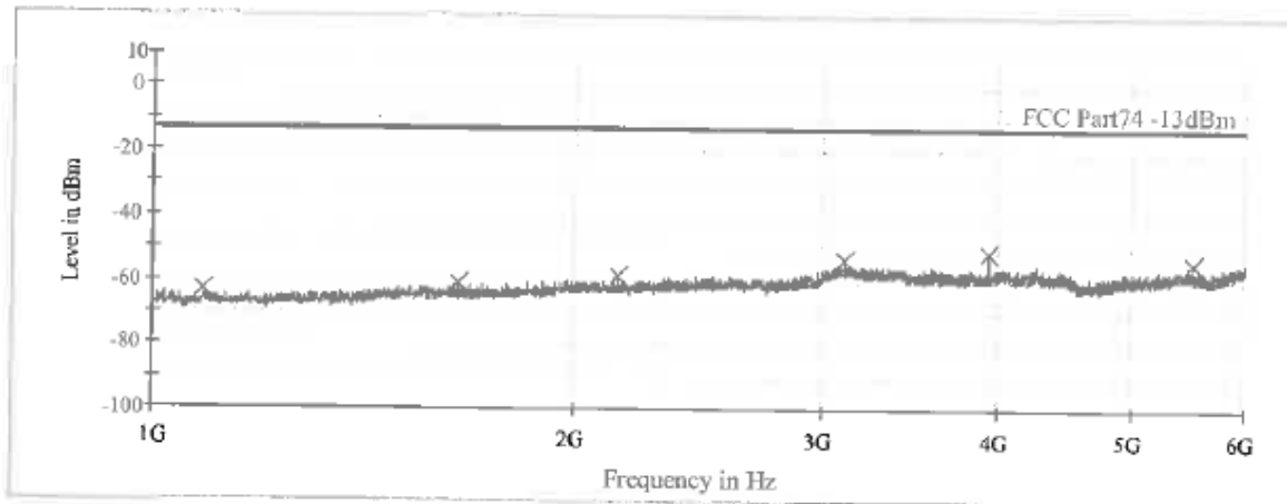
Figure 12: TX Spurious Radiation, Above 1GHz, Horizontal (CH288, High CH)
