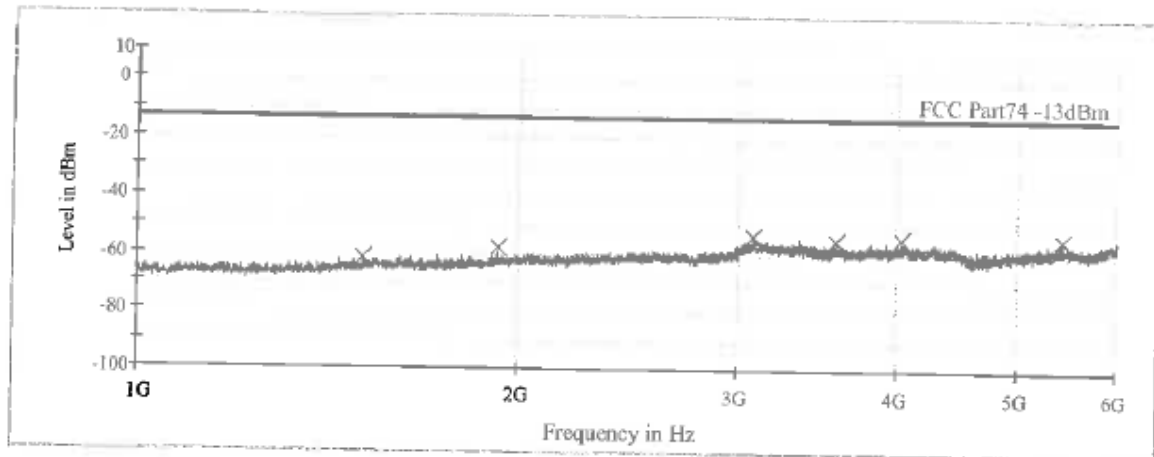
Figure 8: TX Spurious Radiation, Above 1GHz, Horizontal (CH288, Low CH)
