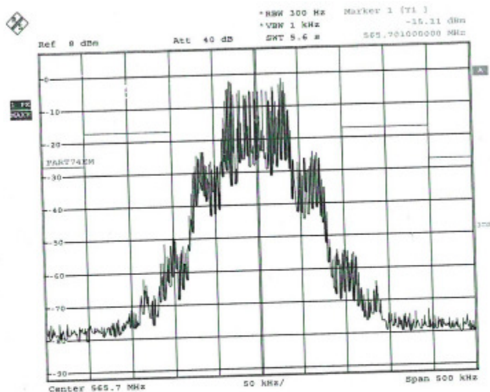
Figure 19: Emission Mask (CH99, High CH)
