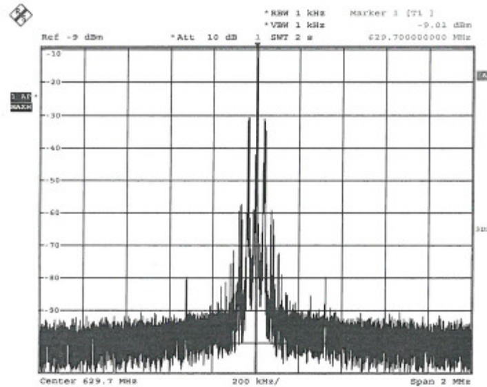
Figure 22: Emission Mask in ETSI EN300 422-1 V1.4.2 (CH99, High CH)
