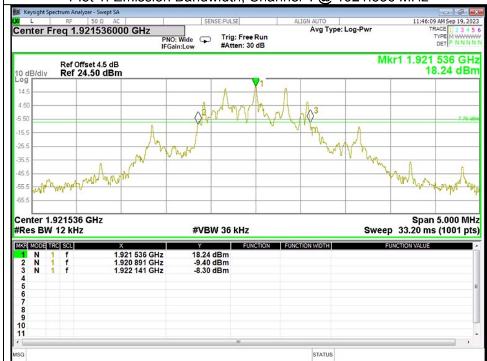
Plot 1. Emission Bandwidth, Channel 4 @ 1921.536 MHz
