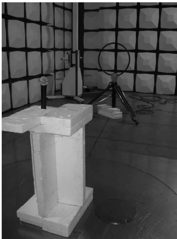
Photograph 1: Set-up for Radiation Measurement below 1GHz
