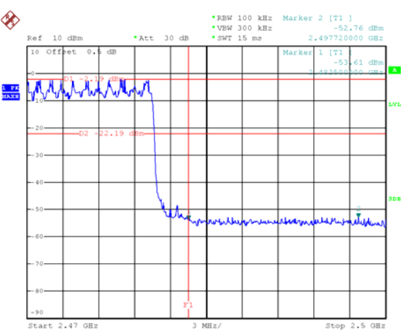
Hopping Band edge-right side
