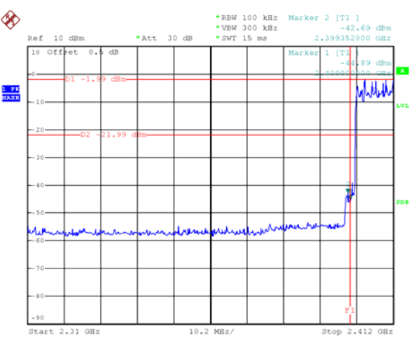
Hopping Band edge-left side
