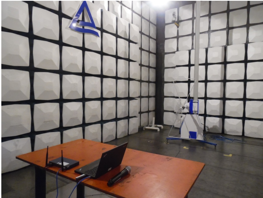
Photograph 2: Set-up for Radiated Emission (30MHz-6GHz)
