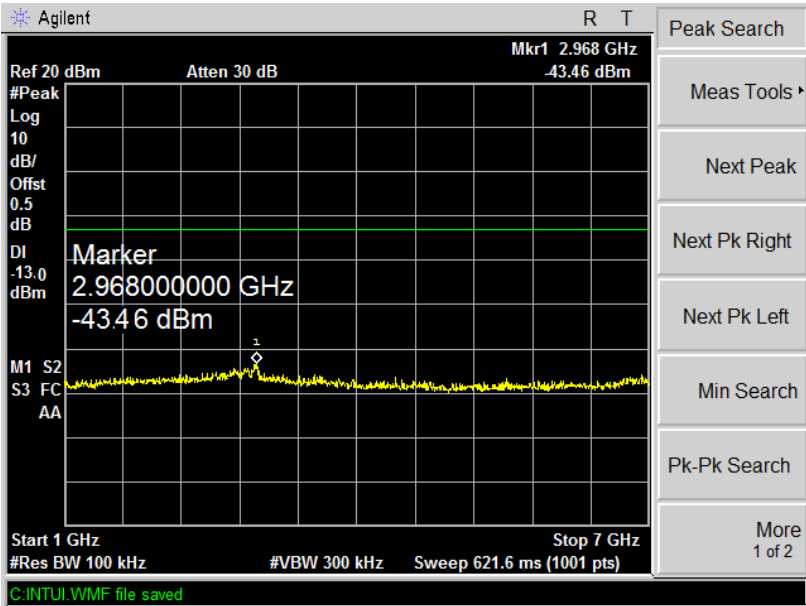
Middle channel 1GHz-7GHz
