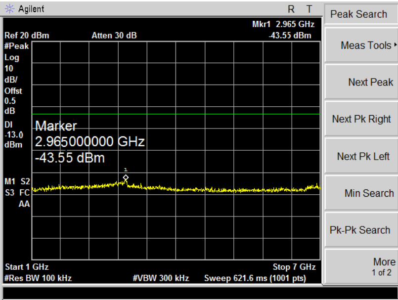
Low channel 1GHz-7GHz
