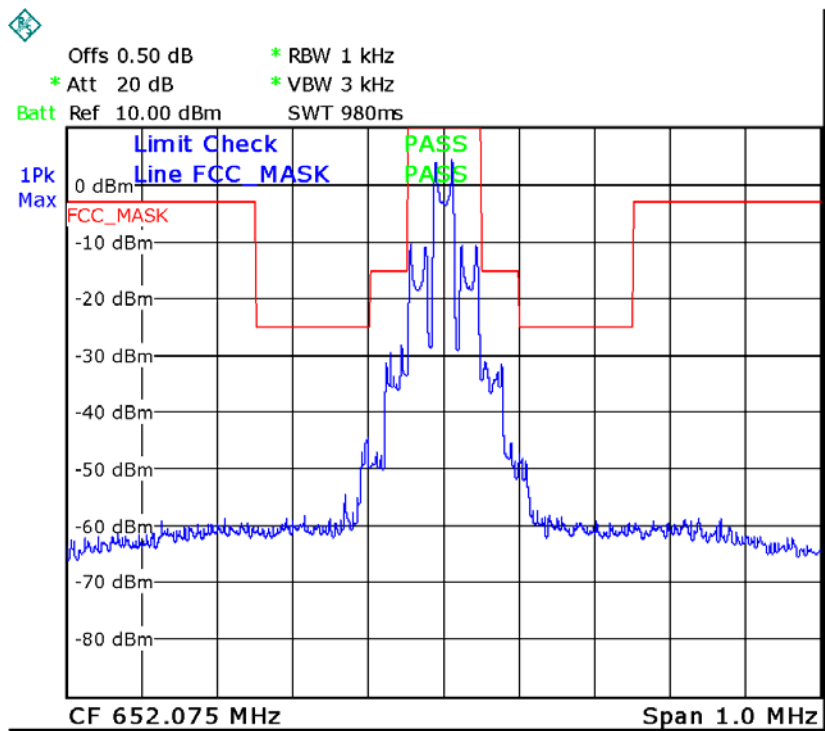
Emission Mask Middle Channel
