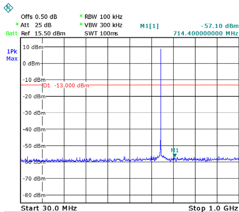
Middle channel 30MHz-1GHz
