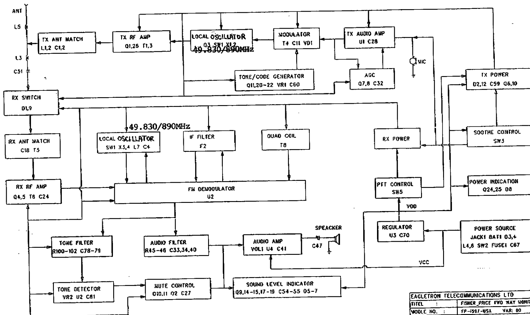
BLOCK DIAGRAM FOR FP-1597-USA
