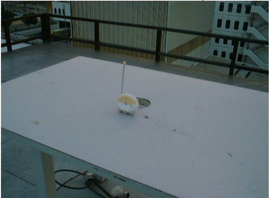
Measurement of Radiated Emission Test Set Up
