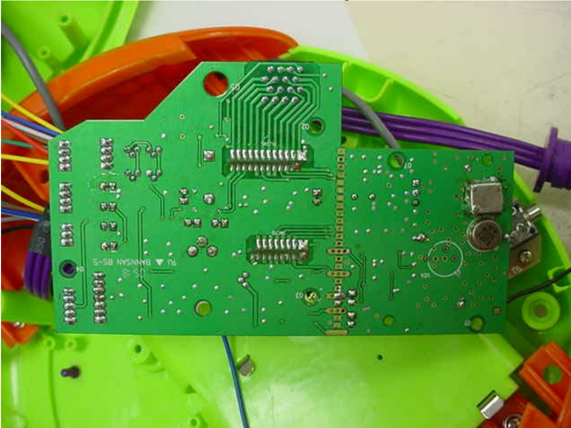
Fisher-Price H6723 Receiver with Small Shielding Can removed– Bottom View
