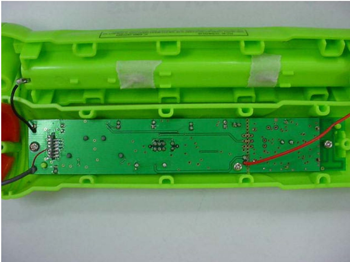
Fisher-Price H6723 Transmitter – Bottom View
