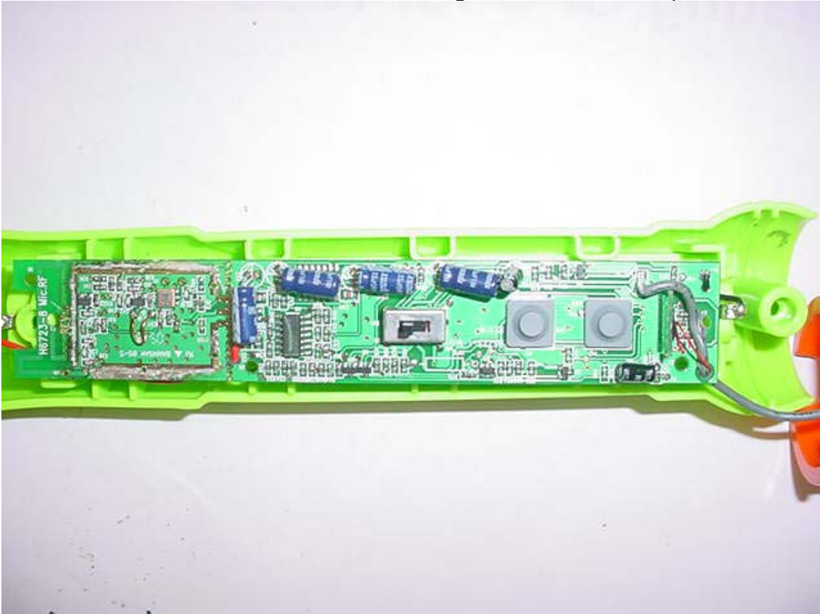
Fisher-Price H6723 Transmitter with Shielding Can Removed – Top View
