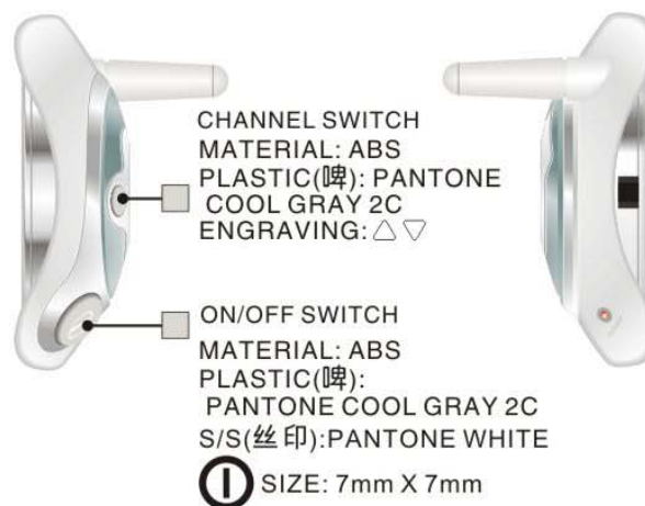
LEFT VIEW
