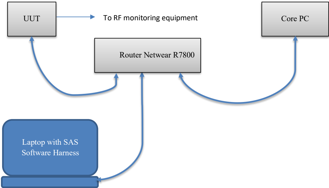
Figure 3.6-1: Setup diagram
