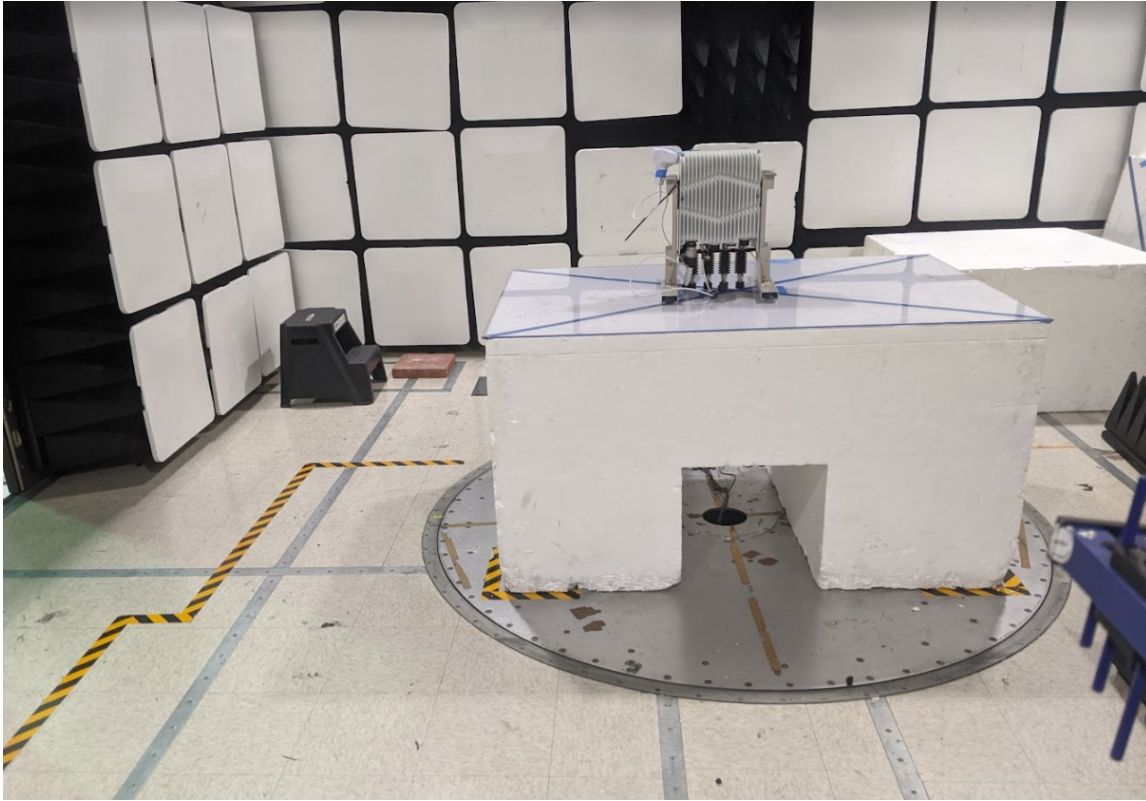
Figure 2 - Radiated emissions below 1 GHz (0.03 – 1 GHz), front view.
