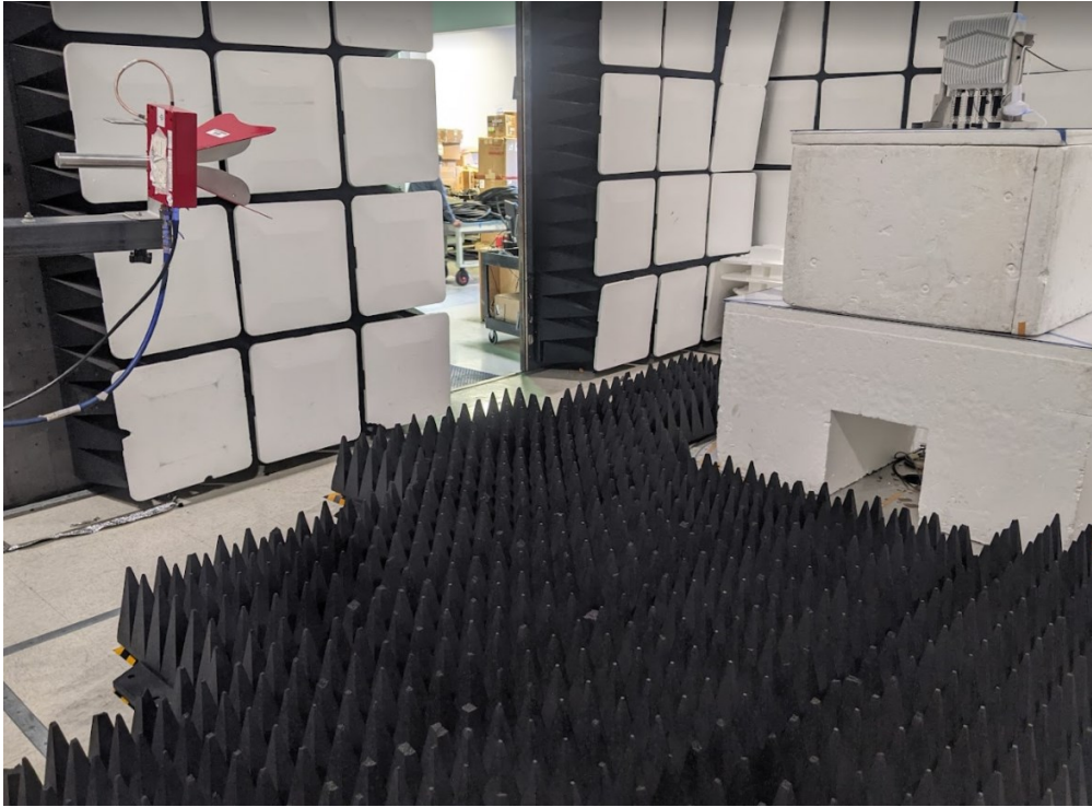
Figure 4 - Radiated emissions above 1 GHz, front view.
