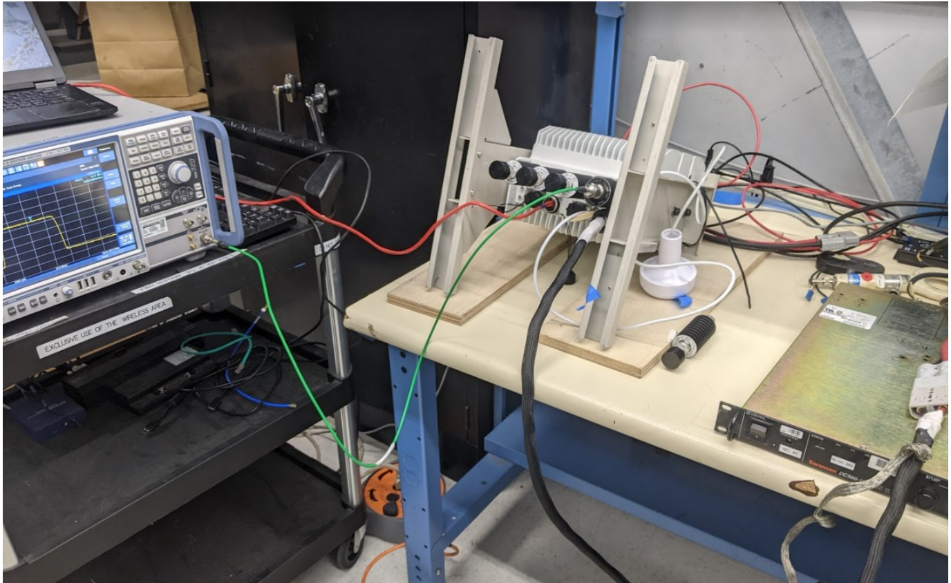
Figure 1 –Test setup – conducted antenna port tests
