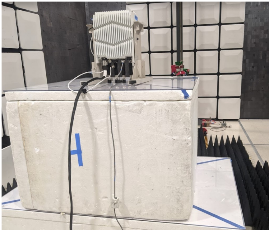
Figure 5 - Radiated emissions above 1 GHz, rear view.
