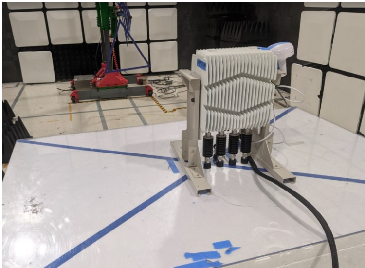
Figure 3 - Radiated emissions below 1 GHz (0.03 – 1 GHz), rear view.
