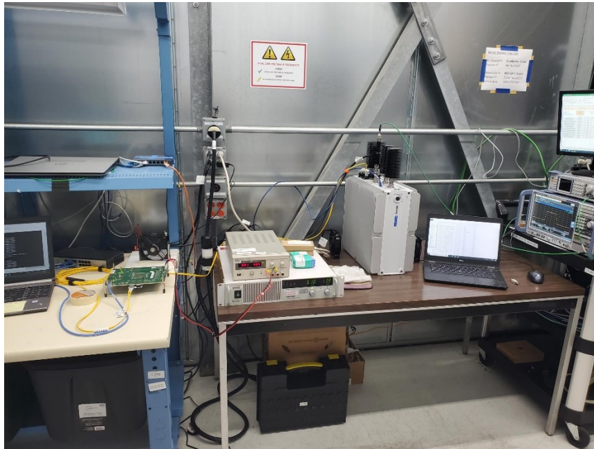
Figure 7 – Test setup – conducted antenna port measurements
