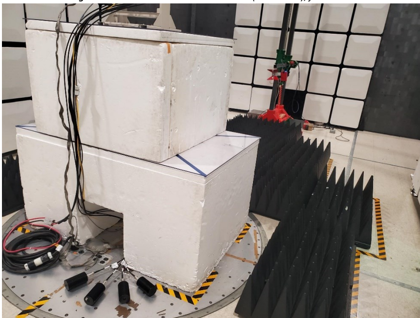
Figure 4 - Radiated emissions above 1 GHz (1 – 10 GHz), rear view.
