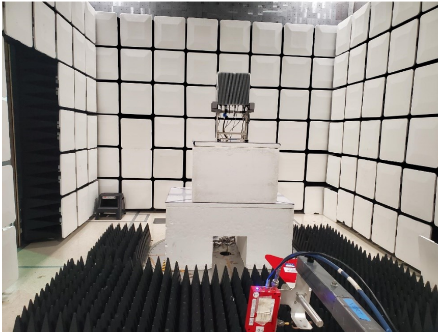
Figure 3 - Radiated emissions above 1 GHz (1 – 10 GHz), front view.
