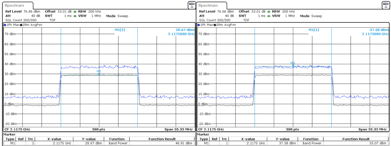
PAPR TX 2117.5 MHz, BW: 15MHz, MOD: 64QAM
