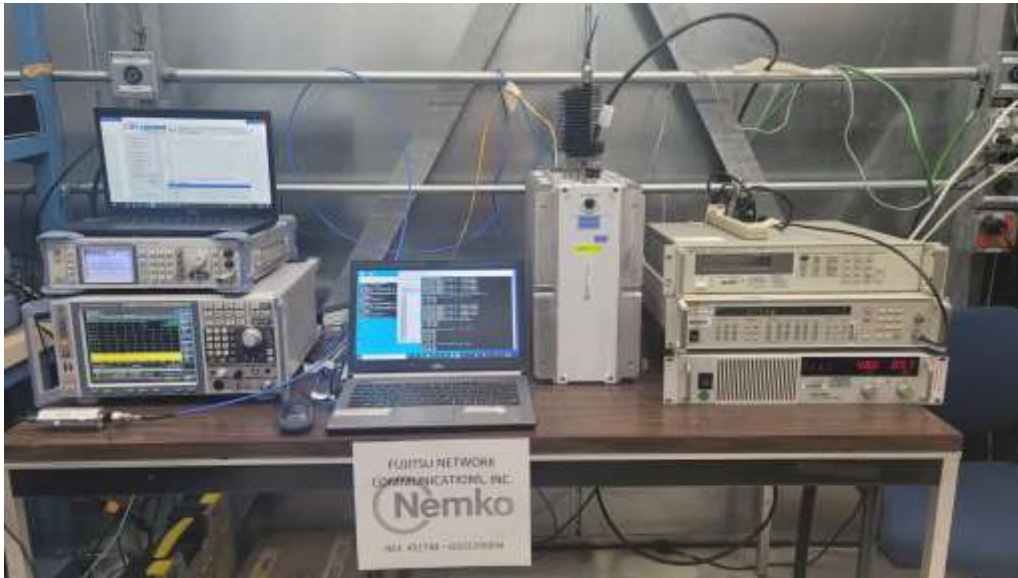
Figure 7 – Test setup (power meter measurements)
