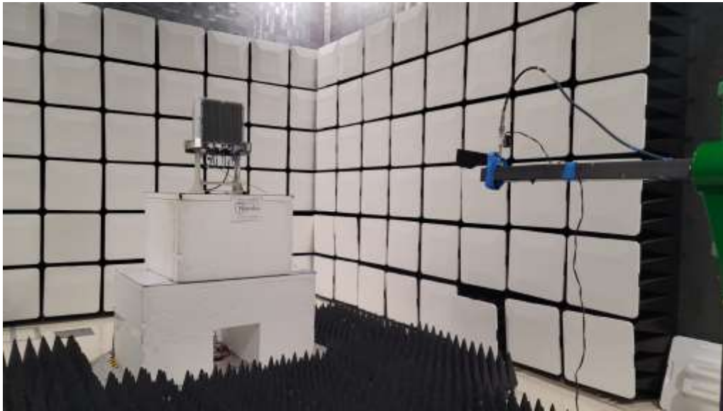
Figure 5 - Radiated emissions above 1 GHz (18 – 26 GHz), front view.
