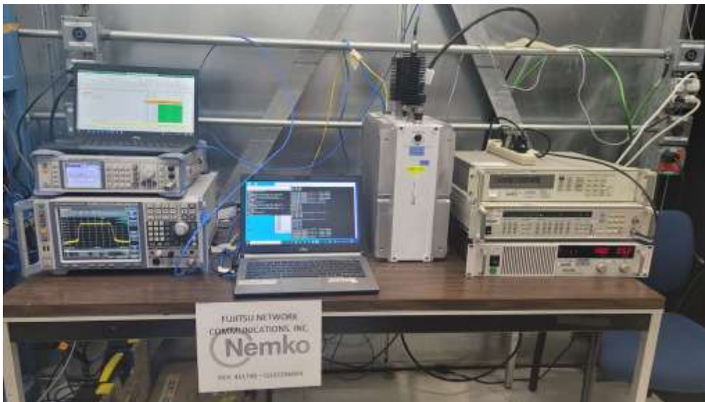
Figure 8 – Test setup (spectrum analyzer measurements)
