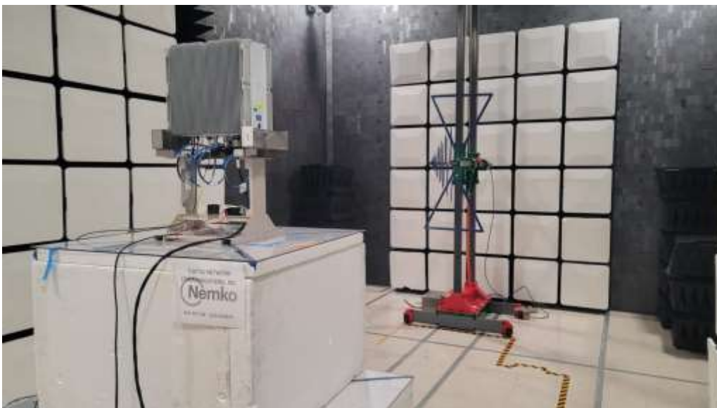
Figure 2 - Radiated emissions below 1 GHz (0.03 – 1 GHz), rear view.
