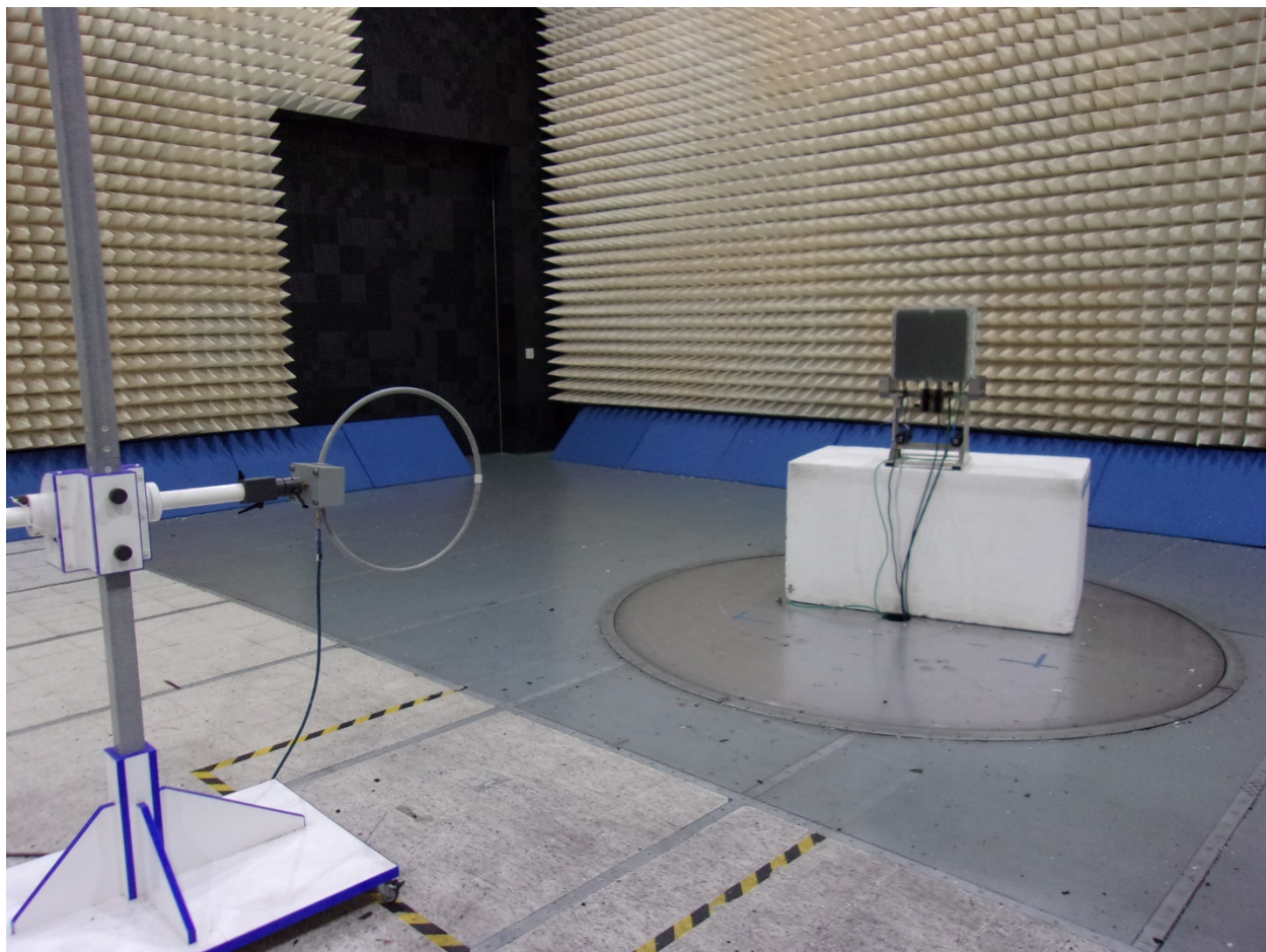
Radiated Spurious Emissions <30MHz
