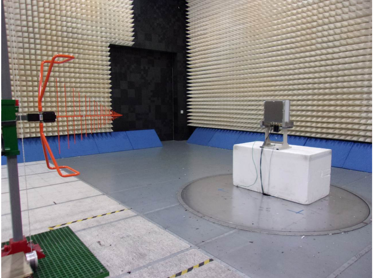
Radiated Spurious Emissions Below 1GHz
