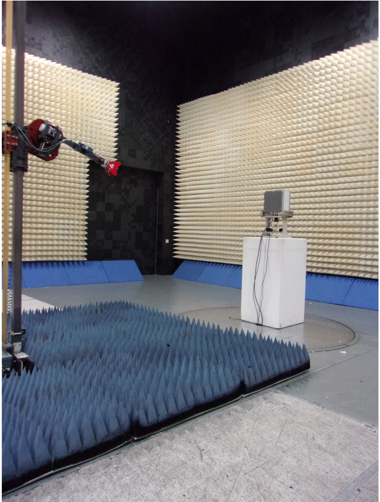
Radiated Spurious Emissions >1GHz
