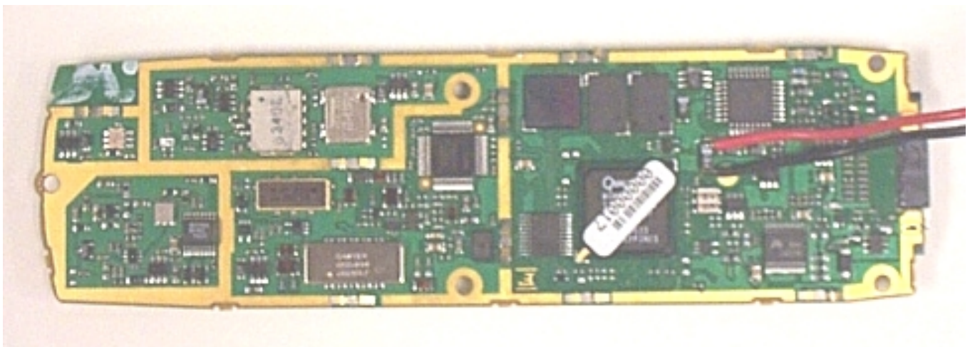
Photo 2 - PCB RX Side
