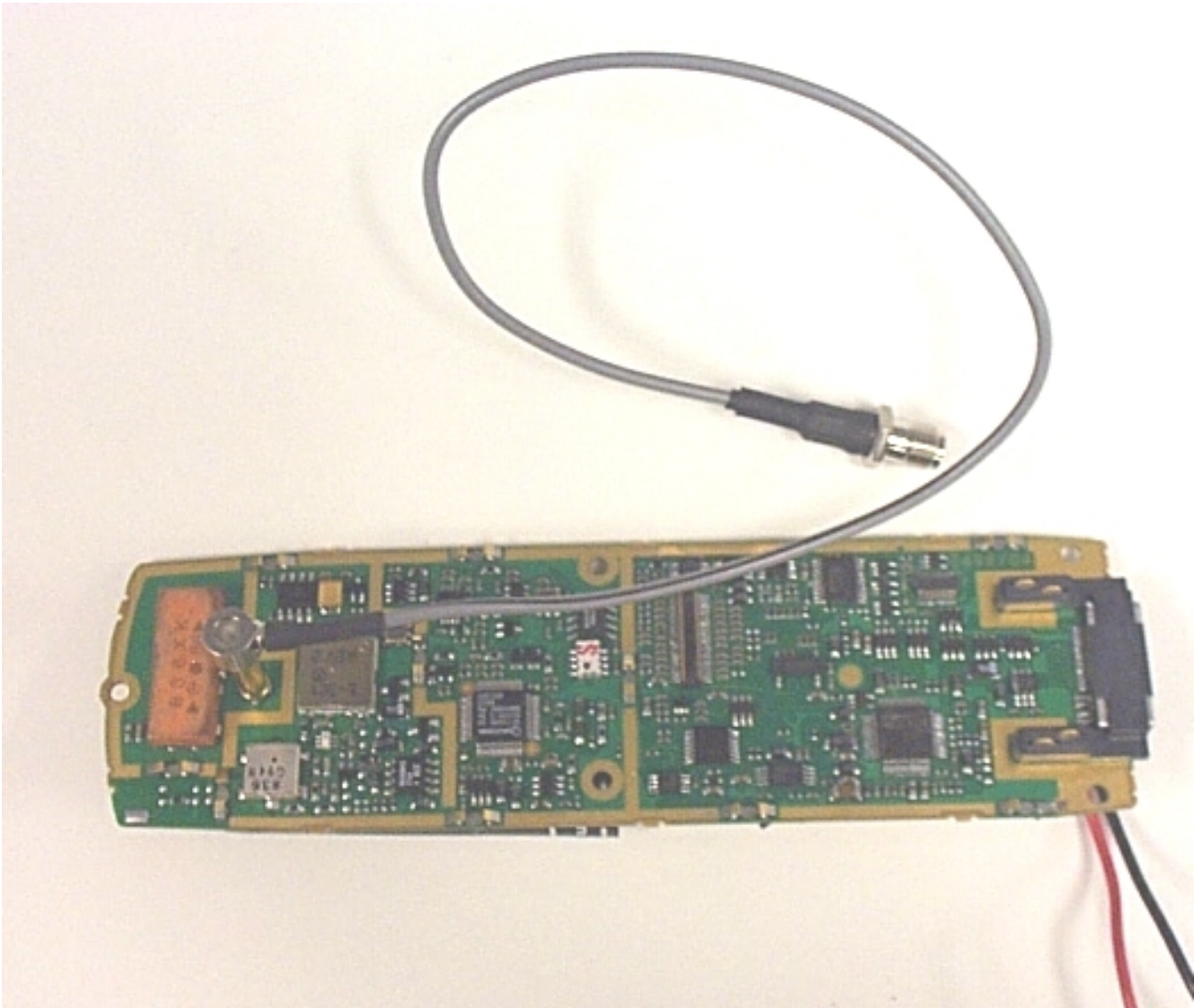
Photo 3 - Antenna Connection for testing
