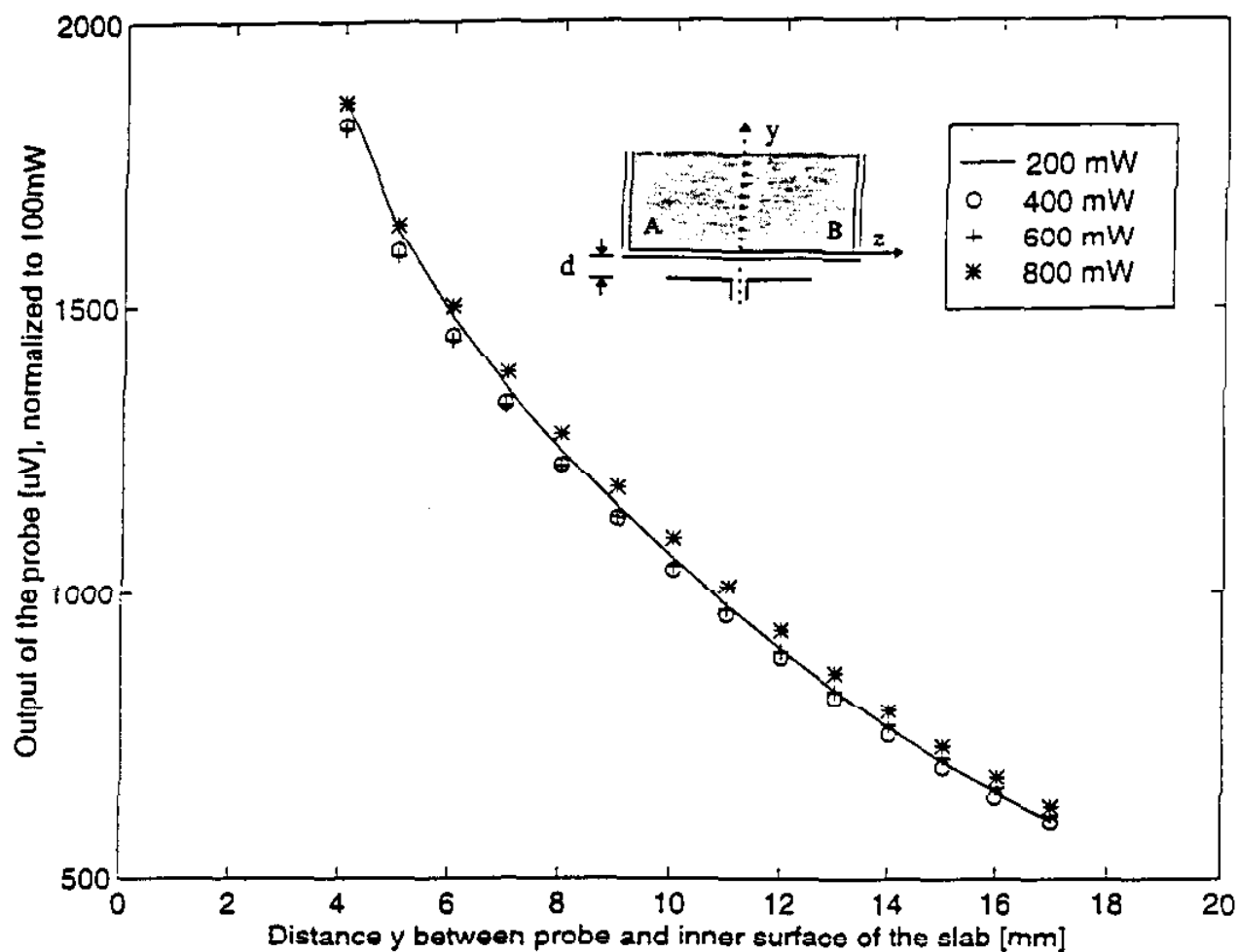
Fig. 3a. Test for square-law behavior at 840 MHz: Variation of the output voltage (proportional to |E_i|^2 ) for different radiated powers normalized to 0.1 W.
