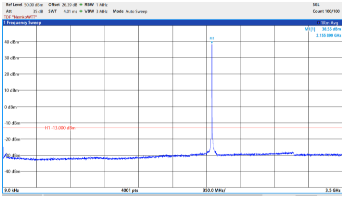
16QAM operation: MID channel
