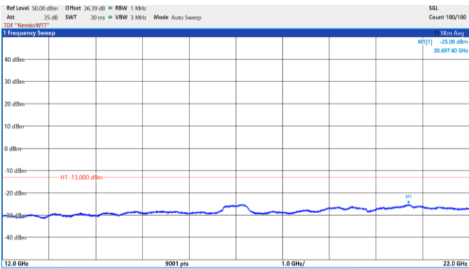
16QAM operation: HIGH channel
