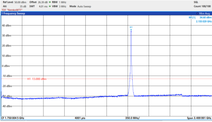
16QAM operation: MID channel
