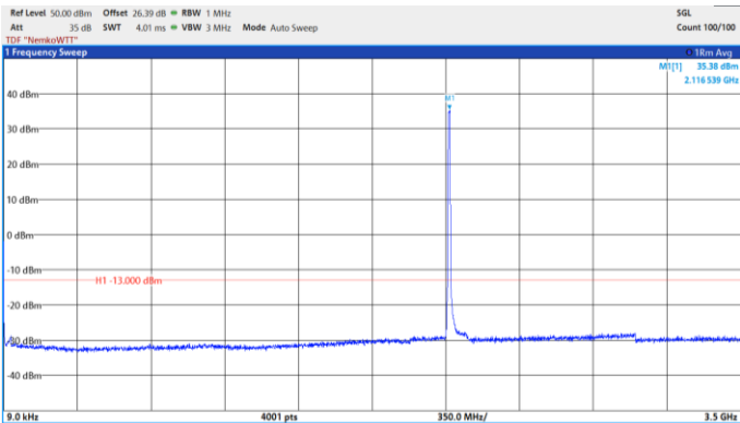
QPSK operation: LOW channel
