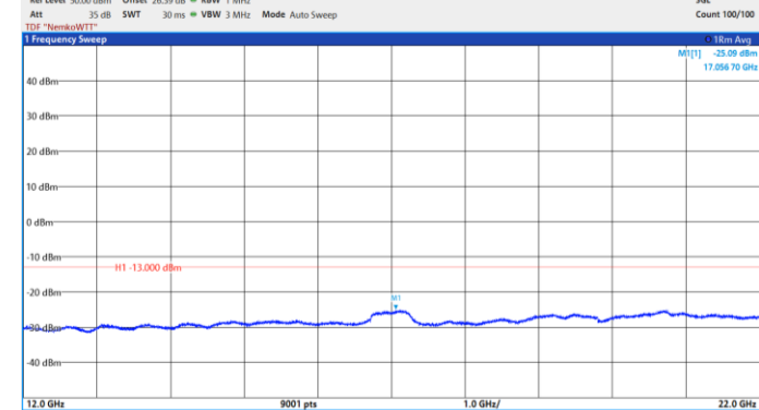
64QAM operation: MID channel
