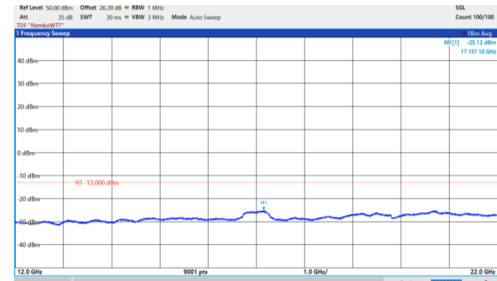
64QAM operation: LOW channel
