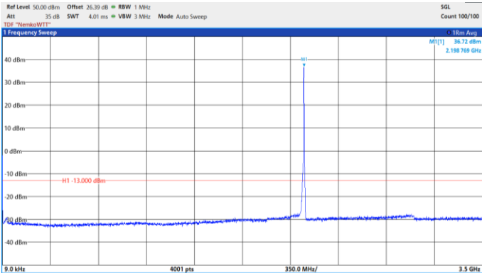
64QAM operation: HIGH channel
