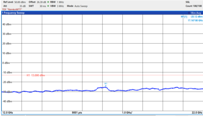
16QAM operation: HIGH channel
