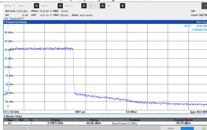
Figure 8.6-156: Conducted Spurious Emissions, Low CH 2117.5 MHz, 15 MHz, 1024QAM, Low band edge.
