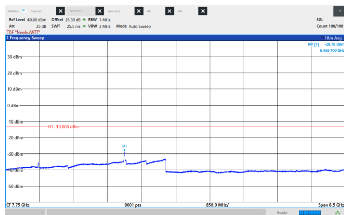
Figure 8.6-148: Conducted Spurious Emissions, Mid CH 2155 MHz, 15 MHz, 256QAM, Frequency range: 3.5 – 12.0 GHz.
