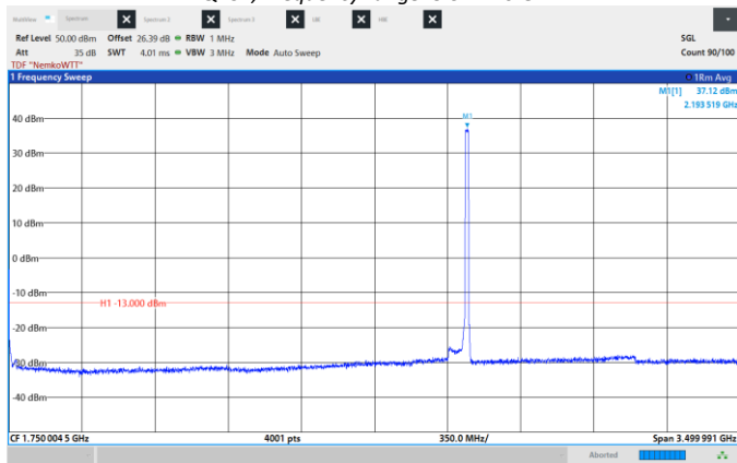
Figure 8.6-118: Conducted Spurious Emissions, High CH 2192.5 MHz, 15 MHz, QPSK, Frequency range: 0.009 – 3500 MHz.
