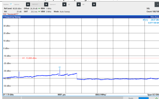
Figure 8.6-141: Conducted Spurious Emissions, High CH 2155 MHz, 15 MHz, 64QAM, Frequency range: 3.5 – 12.0 GHz.
