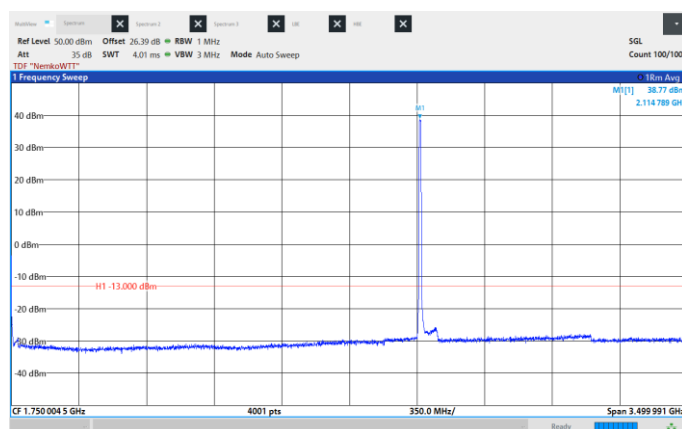
Figure 8.6-78: Conducted Spurious Emissions, Low CH 2115 MHz, 10 MHz, 64QAM, Frequency range: 0.009 -3500 MHz.
