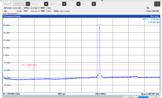
Figure 8.6-147: Conducted Spurious Emissions, Mid CH 2155 MHz, 15 MHz, 256QAM, Frequency range: 0.009 - 3500 MHz.
