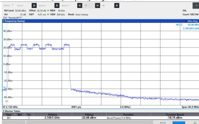
Figure 8.6-124: Conducted Spurious Emissions, Low CH 2117.5 MHz, 15 MHz, 16QAM, Low band edge.
