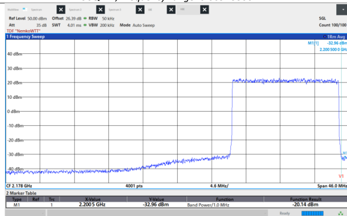
Figure 8.6-152: Conducted Spurious Emissions, High CH 2192.5 MHz, 15 MHz, 256QAM, High band edge.
