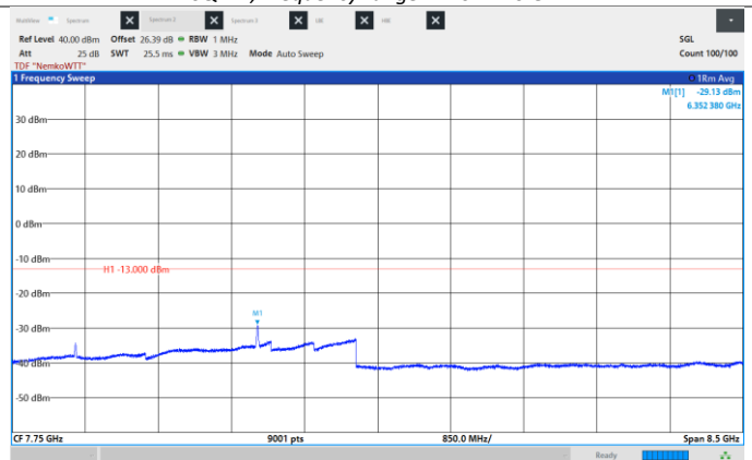
Figure 8.6-134: Conducted Spurious Emissions, Low CH 2117.5 MHz, 15 MHz, 64QAM, Frequency range: 3.5 - 12.0 GHz.
