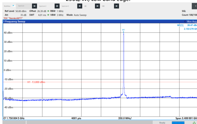
Figure 8.6-93: Conducted Spurious Emissions, Mid CH 2155 MHz, 10 MHz, 256QAM, Frequency range: 0.009 – 3500 MHz.
