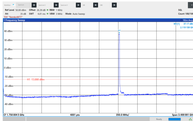
Figure 8.6-154: Conducted Spurious Emissions, Low CH 2117.5 MHz, 15 MHz, 1024QAM, Frequency range: 0.009 -3500 MHz.
