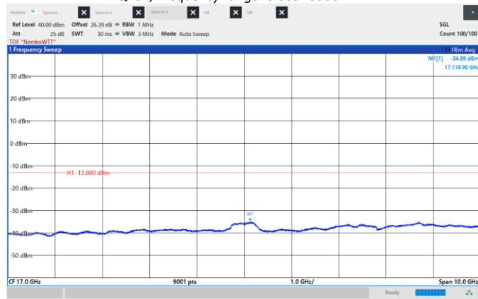
Figure 8.6-117: Conducted Spurious Emissions, Mid CH 2155 MHz, 15 MHz, QPSK, Frequency range: 12.0 – 22.0 GHz.
