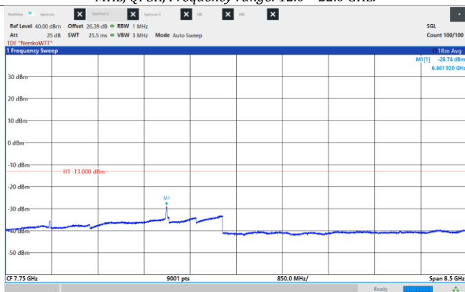
Figure 8.6-116: Conducted Spurious Emissions, Mid CH 2155 MHz, 15 MHz, QPSK, Frequency range: 3.5 - 12.0 GHz.
