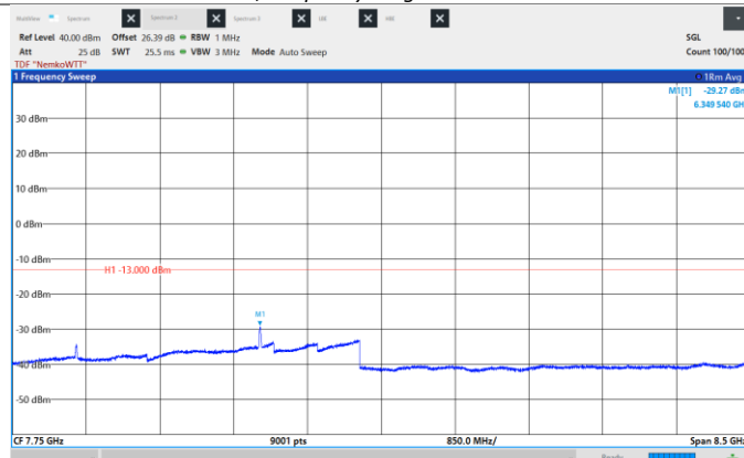
Figure 8.6-144: Conducted Spurious Emissions, Low CH 2117.5 MHz, 15 MHz, 256QAM, Frequency range: 3.5 - 12.0 GHz.
