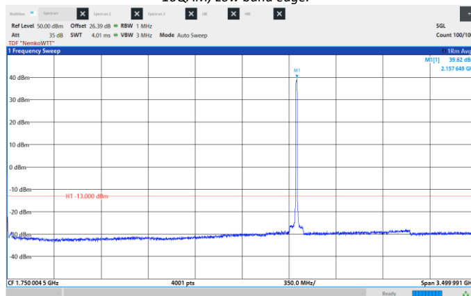
Figure 8.6-71: Conducted Spurious Emissions, Mid CH 2155 MHz, 10 MHz, 16QAM, Frequency range: 0.009 -3500 MHz
