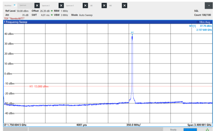
Figure 8.6-126: Conducted Spurious Emissions, Mid CH 2155 MHz, 15 MHz, 16QAM, Frequency range: 0.009 -3500 MHz
