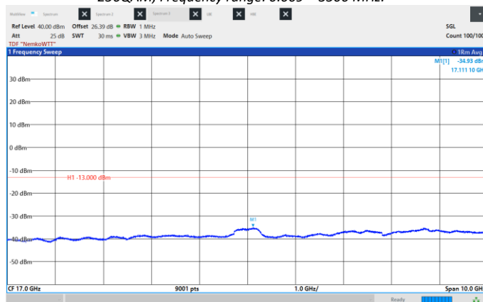
Figure 8.6-95: Conducted Spurious Emissions, Mid CH 2155 MHz, 10 MHz, 256QAM, Frequency range: 12.0 - 22.0 GHz.
