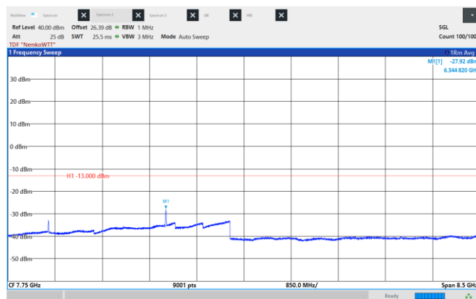
Figure 8.6-90: Conducted Spurious Emissions, Low CH 2115 MHz, 10 MHz, 256QAM, Frequency range: 3.5 – 12.0 GHz.
