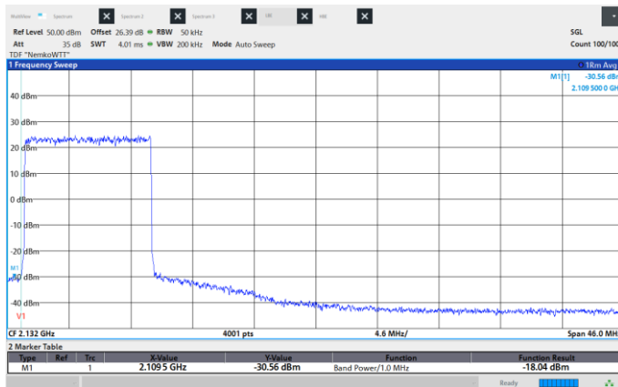
Figure 8.6-102: Conducted Spurious Emissions, Low CH 2115 MHz, 10 MHz, 1024QAM, Low band edge.
