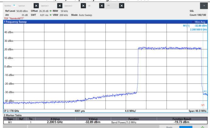
Figure 8.6-142: Conducted Spurious Emissions, High CH 2192.5 MHz, 15 MHz, 64QAM, High band edge.
