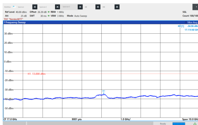
Figure 8.6-84: Conducted Spurious Emissions, Mid CH 2155 MHz, 10 MHz, 64QAM, Frequency range: 12.0 – 22.0 GHz.
