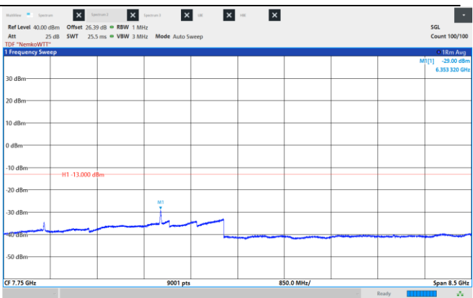
Figure 8.6-112: Conducted Spurious Emissions, Low CH 2117.5 MHz, 15 MHz, QPSK, Frequency range: 3.5 -12.0 GHz.
