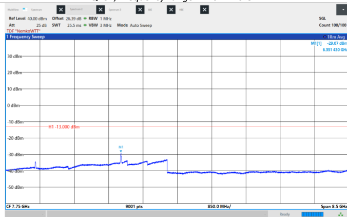
Figure 8.6-123: Conducted Spurious Emissions, Low CH 2117.5 MHz, 15 MHz, 16QAM, Frequency range: 3.5 - 12.0 GHz.
