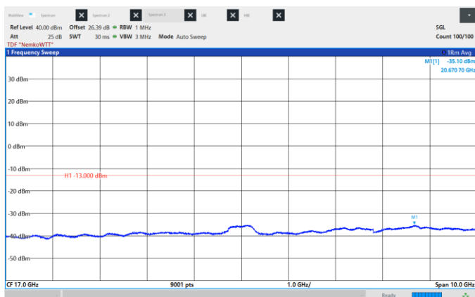
Figure 8.6-114: Conducted Spurious Emissions, Low CH 2117.5 MHz, 15 MHz, QPSK, Frequency range: 12.0 – 22.0 GHz.
