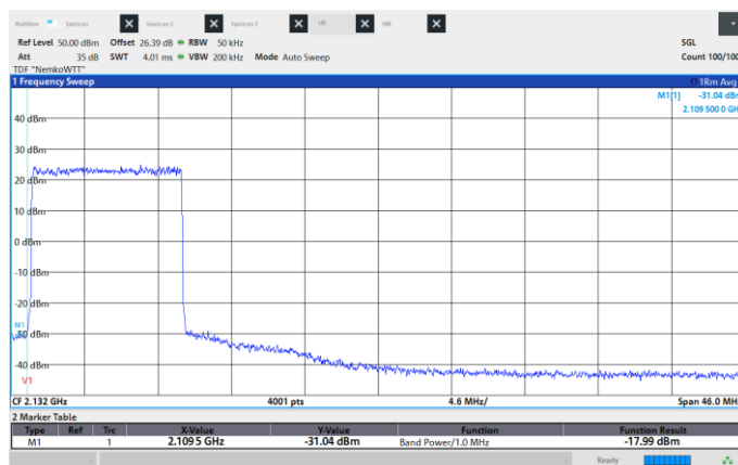
Figure 8.6-91: Conducted Spurious Emissions, Low CH 2115 MHz, 10 MHz, 256QAM, Low band edge.
