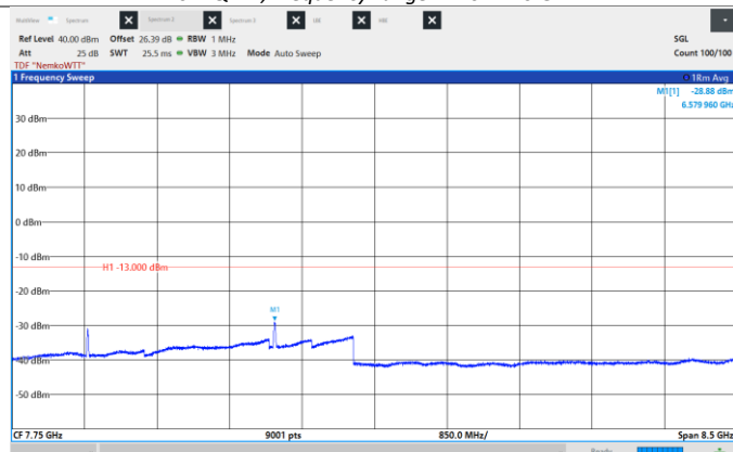
Figure 8.6-160: Conducted Spurious Emissions, High CH 2192.5 MHz, 15 MHz, 1024QAM, Frequency range: 3.5 -12.0 GHz.
