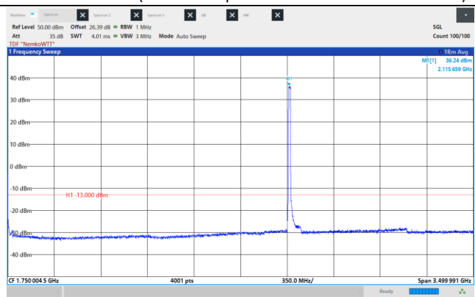
Figure 8.6-111: Conducted Spurious Emissions, Low CH 2117.5 MHz, 15 MHz, QPSK, Frequency range: 0.009 – 3500 MHz.
