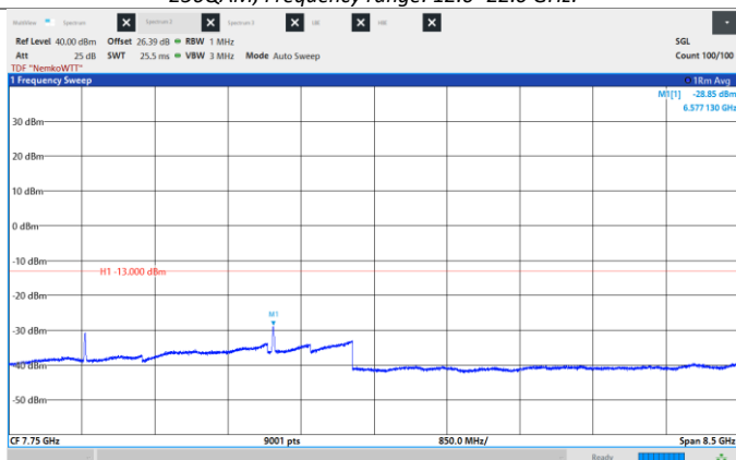
Figure 8.6-151: Conducted Spurious Emissions, High CH 2192.5 MHz, 15 MHz, 256QAM, Frequency range: 3.5 – 12.0 GHz
