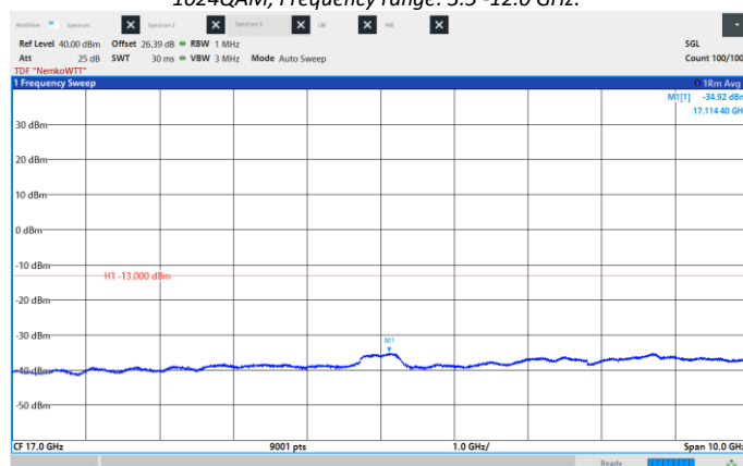
Figure 8.6-110: Conducted Spurious Emissions High CH 2195 MHz, 10 MHz, 1024QAM, Frequency range: 12.0 -22.0 GHz.
