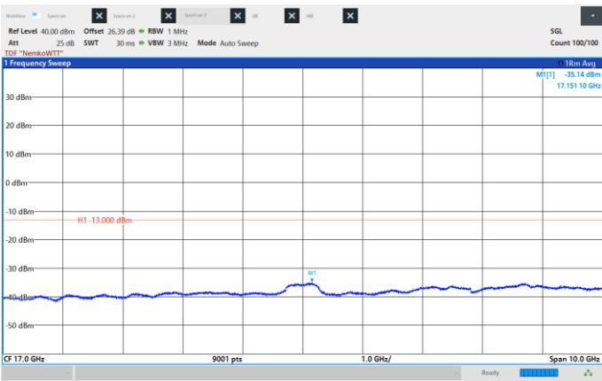
Figure 8.6-73: Conducted Spurious Emissions, Mid CH 2155 MHz, 10 MHz, 16QAM, Frequency range: 12.0 – 22.0 GHz.
