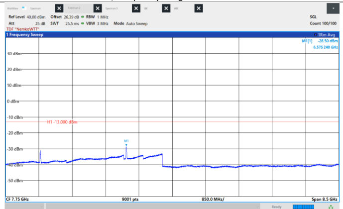
Figure 8.6-130: Conducted Spurious Emissions, High CH 2192.5 MHz, 15 MHz, 16QAM, Frequency range: 3.5 - 12.0 GHz
