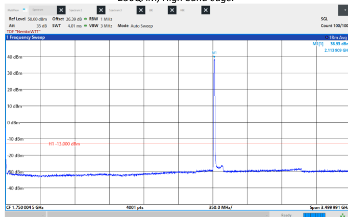
Figure 8.6-100: Conducted Spurious Emissions, Low CH 2115 MHz, 10 MHz, 1024QAM, Frequency range: 0.009 -3500 MHz.
