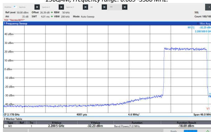
Figure 8.6-98: Conducted Spurious Emissions, High CH 2195 MHz, 10 MHz, 256QAM, High band edge.
