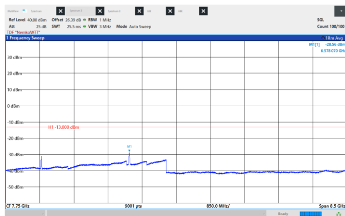
Figure 8.6-119: Conducted Spurious Emissions, High CH 2192.5 MHz, 15 MHz, QPSK, Frequency range: 3.5 -12.0 GHz.
