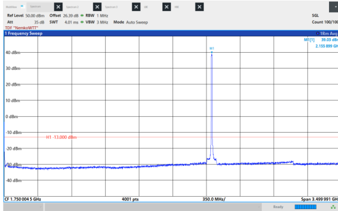
Figure 8.6-104: Conducted Spurious Emissions, Mid CH 2155 MHz, 10 MHz, 1024QAM, Frequency range: 0.009 – 3500 MHz.
