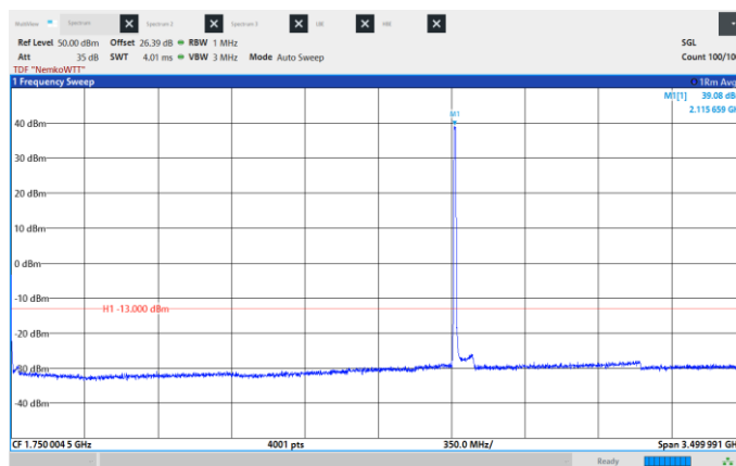
Figure 8.6-67: Conducted Spurious Emissions, Low CH 2115 MHz, 10 MHz, 16QAM, Frequency range: 0.009 - 3500 MHz.
