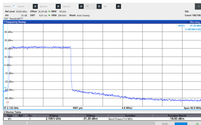
Figure 8.6-113: Conducted Spurious Emissions, Low CH 2117.5 MHz, 15 MHz, QPSK, Low band edge.
