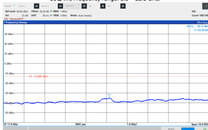
Figure 8.6-70: Conducted Spurious Emissions, Low CH 2115 MHz, 10 MHz, 16QAM, Frequency range: 12.0 -22.0 GHz
