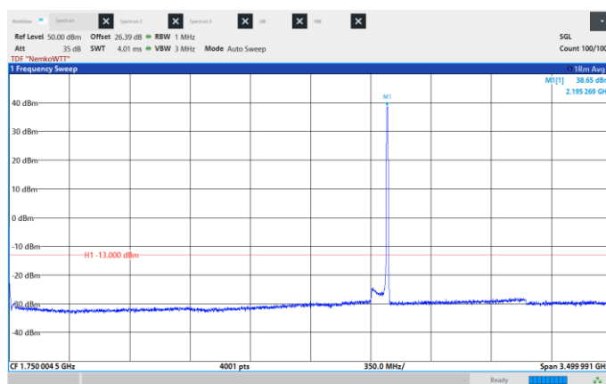
Figure 8.6-85: Conducted Spurious Emissions, High CH 2195 MHz, 10 MHz, 64QAM, Frequency range: 0.009 – 3500 MHz.
