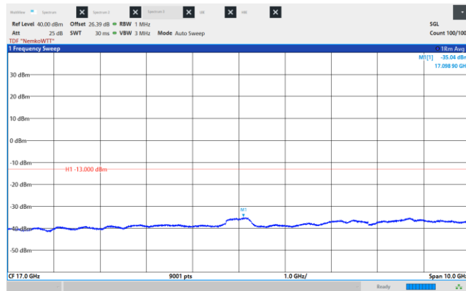
Figure 8.6-125: Conducted Spurious Emissions, Low CH 2117.5 MHz, 15 MHz, 16QAM, Frequency range: 12.0 -22.0 GHz
