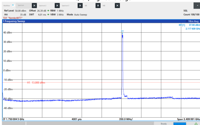
Figure 8.6-122: Conducted Spurious Emissions, Low CH 2117.5 MHz, 15 MHz, 16QAM, Frequency range: 0.009 - 3500 MHz.
