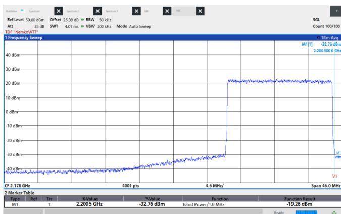
Figure 8.6-120: Conducted Spurious Emissions, High CH 2192.5 MHz, 15 MHz, QPSK, High band edge.
