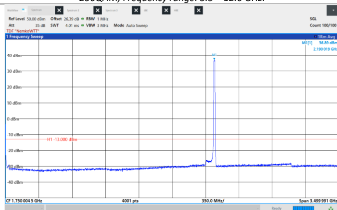
Figure 8.6-150: Conducted Spurious Emissions, High CH 2192.5 MHz, 15 MHz, 256QAM, Frequency range: 0.009 -3500 MHz.
