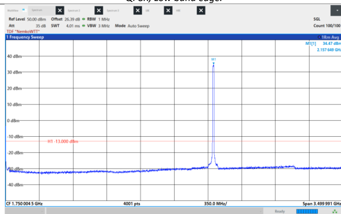
Figure 8.6-115: Conducted Spurious Emissions, Mid CH 2155 MHz, 15 MHz, QPSK, Frequency range: 0.009 - 3500 MHz.
