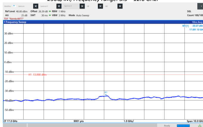
Figure 8.6-92: Conducted Spurious Emissions, Low CH 2115 MHz, 10 MHz, 256QAM, Frequency range: 12.0 – 22.0 GHz.
