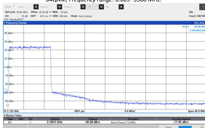
Figure 8.6-80: Conducted Spurious Emissions, Low CH 2115 MHz, 10 MHz, 64QAM, Low band edge
