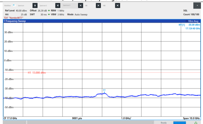
Figure 8.6-157: Conducted Spurious Emissions, Low CH 2117.5 MHz, 15 MHz, 1024QAM, Frequency range: 12.0 - 22.0 GHz.
