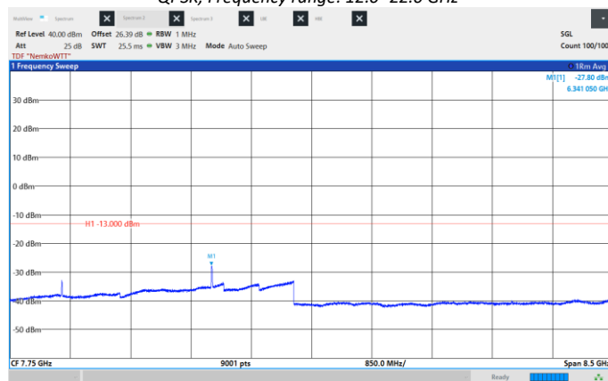
Figure 8.6-68: Conducted Spurious Emissions, Low CH 2115 MHz, 10 MHz, 16QAM, Frequency range: 3.5 - 12.0 GHz.
