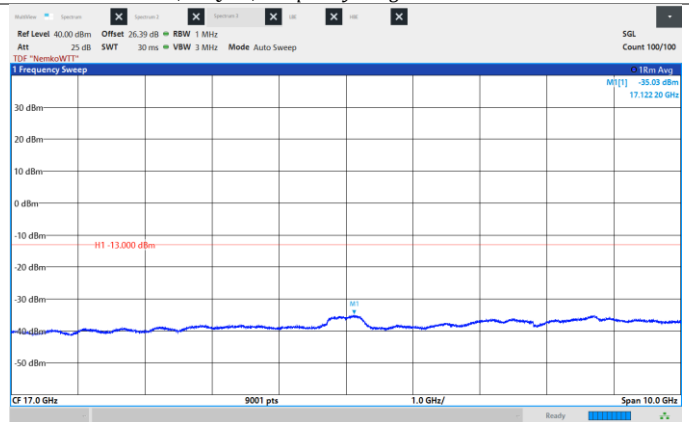
Figure 8.6-136: Conducted Spurious Emissions, Low CH 2117.5 MHz, 15 MHz, 64QAM, Frequency range: 12.0 - 22.0 GHz.
