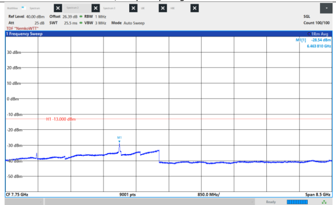
Figure 8.6-50: Conducted Spurious Emissions, Mid CH 2155 MHz, 15 MHz, 1024QAM, Frequency range: 3.5 - 12.0 GHz.
