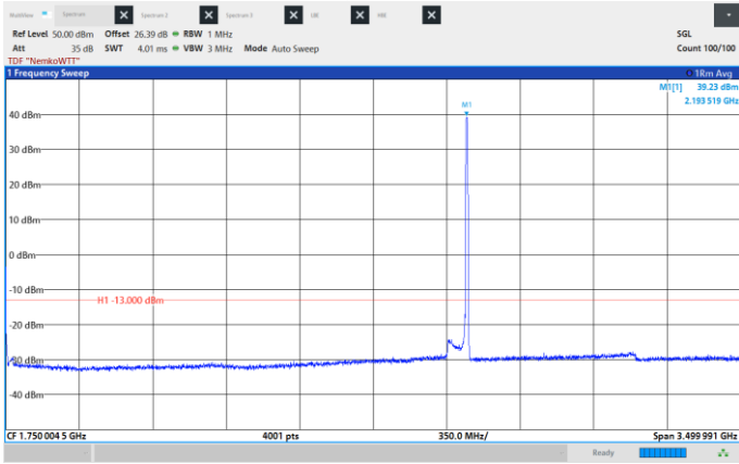
Figure 8.6-74: Conducted Spurious Emissions, High CH 2195 MHz, 10 MHz, 16QAM, Frequency range: 0.009 -3500 MHz.
