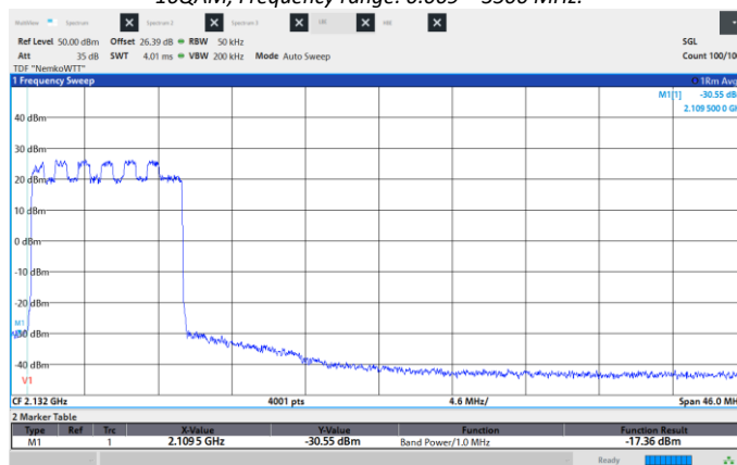
Figure 8.6-69: Conducted Spurious Emissions, Low CH 2115 MHz, 10 MHz, 16QAM, Low band edge.
