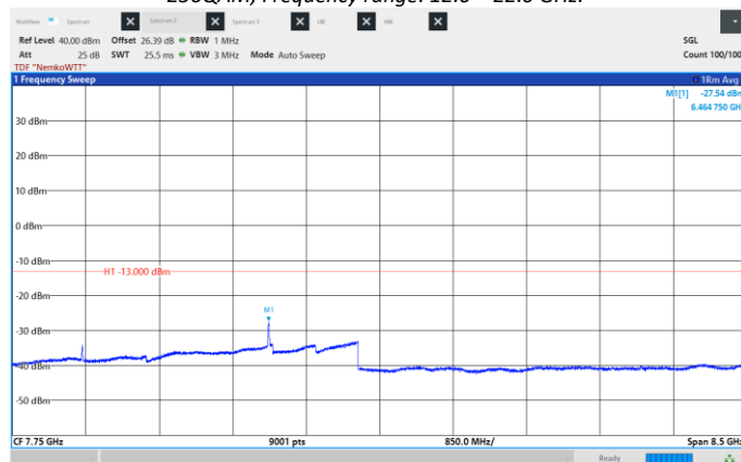
Figure 8.6-94: Conducted Spurious Emissions, Mid CH 2155 MHz, 10 MHz, 256QAM, Frequency range: 3.5 – 12.0 GHz.
