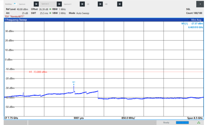
Figure 8.6-105: Conducted Spurious Emissions, Mid CH 2155 MHz, 10 MHz, 1024QAM, Frequency range: 3.5 – 12.0 GHz.
