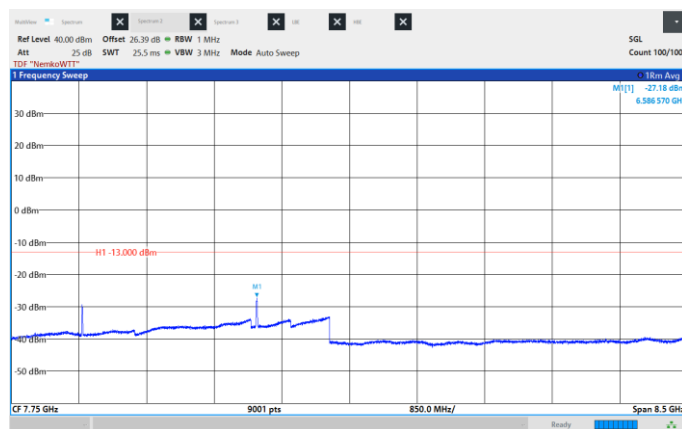
Figure 8.6-108: Conducted Spurious Emissions, High CH 2195 MHz, 10 MHz, 1024QAM, Frequency range: 3.5 -12.0 GHz.
