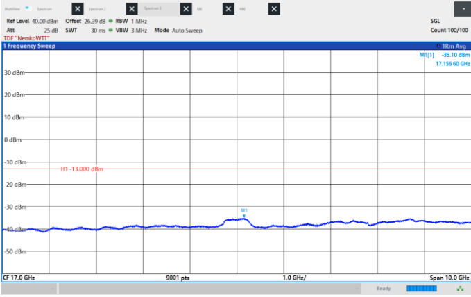
Figure 8.6-77: Conducted Spurious Emissions, High CH 2195 MHz, 10 MHz, 16QAM, Frequency range: 12.0 -22.0 GHz.
