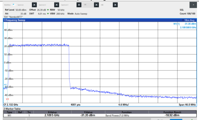
Figure 8.6-145: Conducted Spurious Emissions, Low CH 2117.5 MHz, 15 MHz, 256QAM, Low band edge.
