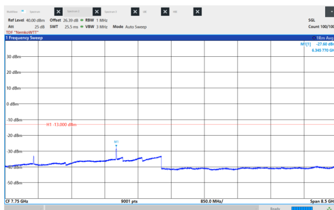
Figure 8.6-79: Conducted Spurious Emissions, Low CH 2115 MHz, 10 MHz, 64QAM, Frequency range: 3.5 - 12.0 GHz.
