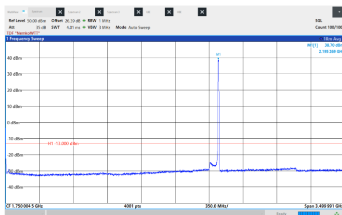
Figure 8.6-96: Conducted Spurious Emissions, High CH 2195 MHz, 10 MHz, 256QAM, Frequency range: 0.009 -3500 MHz.
