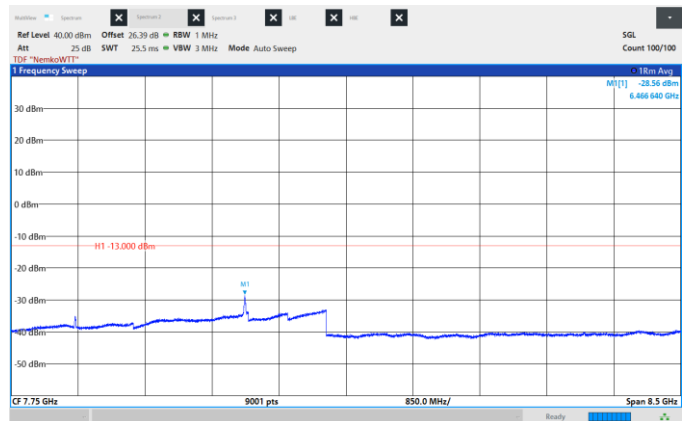
Figure 8.6-138: Conducted Spurious Emissions, Mid CH 2155 MHz, 15 MHz, 64QAM, Frequency range: 3.5 -12.0 GHz.
