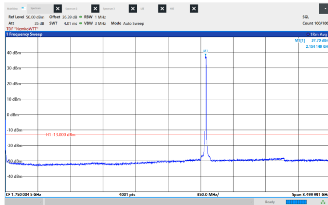
Figure 8.6-137: Conducted Spurious Emissions, Mid CH 2155 MHz, 15 MHz, 64QAM, Frequency range: 0.009 -3500 MHz
