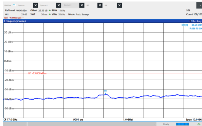
Figure 8.6-143: Conducted Spurious Emissions, High CH 2192.5 MHz, 15 MHz, 64QAM, Frequency range: 12.0 -22.0 GHz
