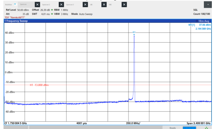
Figure 8.6-107: Conducted Spurious Emissions, High CH 2195 MHz, 10 MHz, 1024QAM, Frequency range: 0.009 -3500 MHz.
