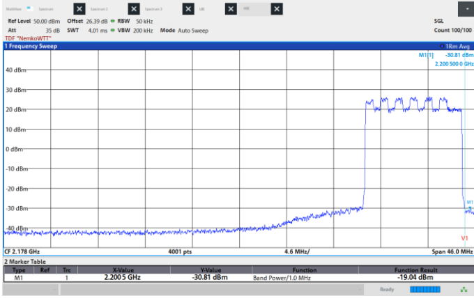
Figure 8.6-76: Conducted Spurious Emissions, High CH 2195 MHz, 10 MHz, 16QAM, High band edge
