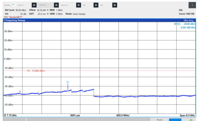
Figure 8.6-155: Conducted Spurious Emissions, Low CH 2117.5 MHz, 15 MHz, 1024QAM, Frequency range: 3.5 -12.0 GHz.
