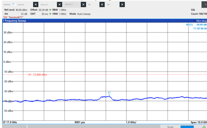
Figure 8.6-106: Conducted Spurious Emissions, Mid CH 2155 MHz, 10 MHz, 1024QAM, Frequency range: 12.0 -22.0 GHz.
