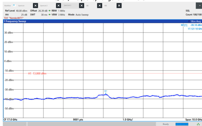
Figure 8.6-121: Conducted Spurious Emissions, High CH 2192.5 MHz, 15 MHz, QPSK, Frequency range: 12.0 -22.0 GHz
