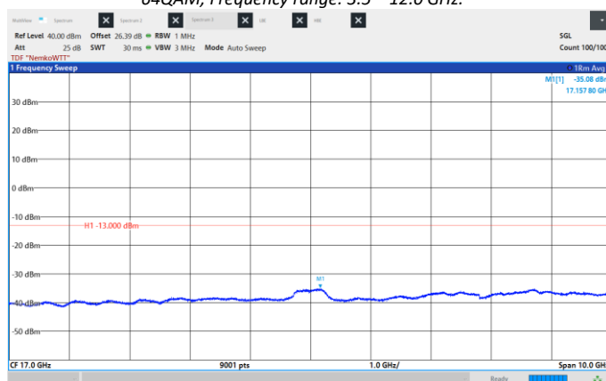
Figure 8.6-81: Conducted Spurious Emissions, Low CH 2115 MHz, 10 MHz, 64QAM, Frequency range: 12.0 - 22.0 GHz.
