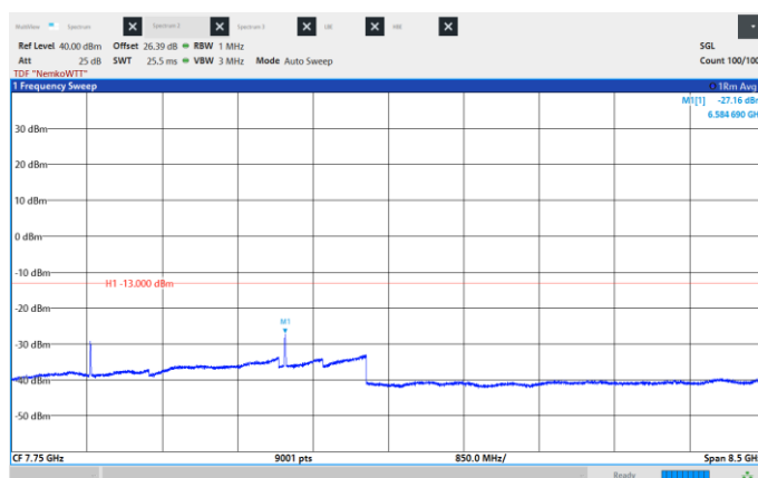
Figure 8.6-97: Conducted Spurious Emissions, High CH 2195 MHz, 10 MHz, 256QAM, Frequency range: 3.5 - 12.0 GHz
