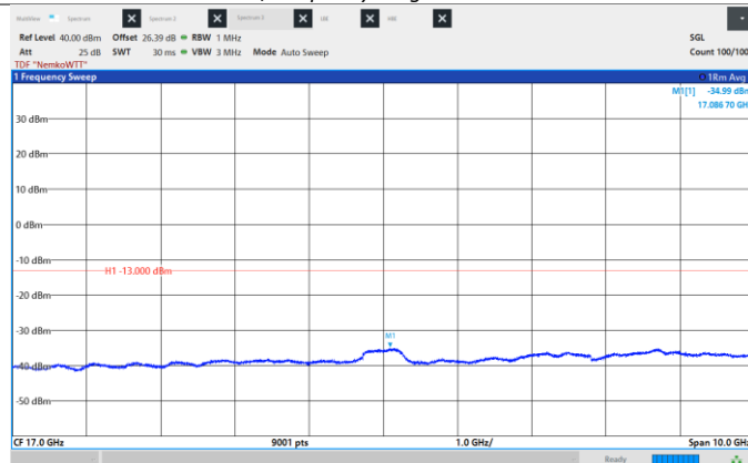
Figure 8.6-146: Conducted Spurious Emissions, Low CH 2117.5 MHz, 15 MHz, 256QAM, Frequency range: 12.0 - 22.0 GHz.
