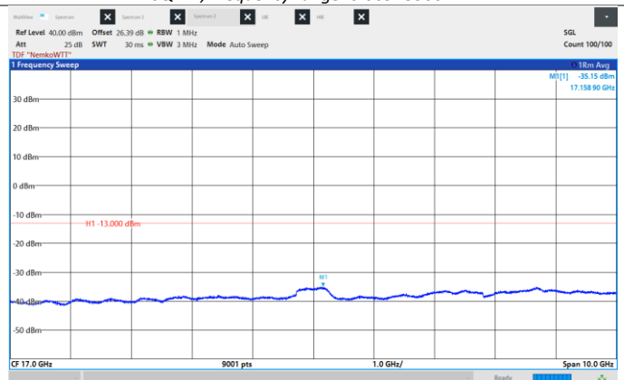
Figure 8.6-128: Conducted Spurious Emissions, Mid CH 2155 MHz, 15 MHz, 16QAM, Frequency range: 12.0 - 22.0 GHz.
