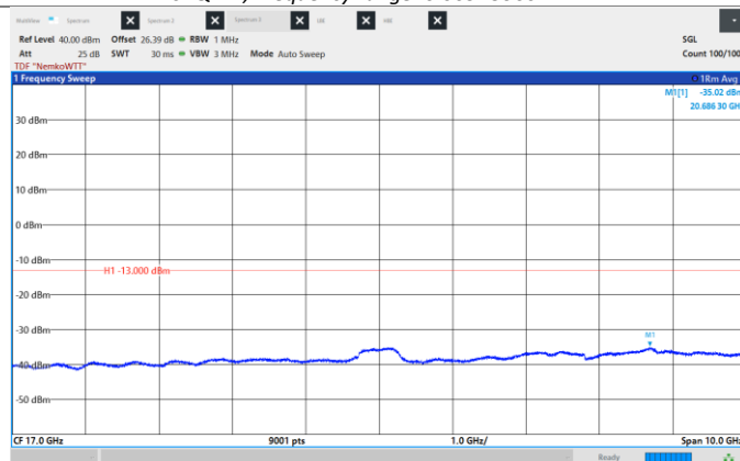
Figure 8.6-139: Conducted Spurious Emissions, Mid CH 2155 MHz, 15 MHz, 64QAM, Frequency range: 12.0 – 22.0 GHz.
