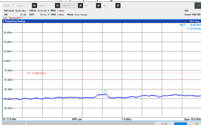
Figure 8.6-153: Conducted Spurious Emissions, High CH 2192.5 MHz, 15 MHz, 256QAM, Frequency range: 12.0 – 22.0 GHz.
