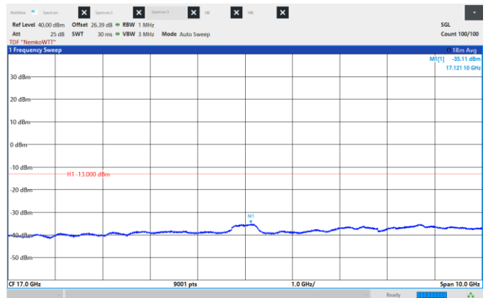
Figure 8.6-132: Conducted Spurious Emissions, High CH 2192.5 MHz, 15 MHz, 16QAM, Frequency range: 12.0 -22.0 GHz.
