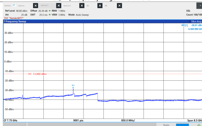
Figure 8.6-127: Conducted Spurious Emissions, Mid CH 2155 MHz, 15 MHz, 16QAM, Frequency range: 3.5 -12.0 GHz.
