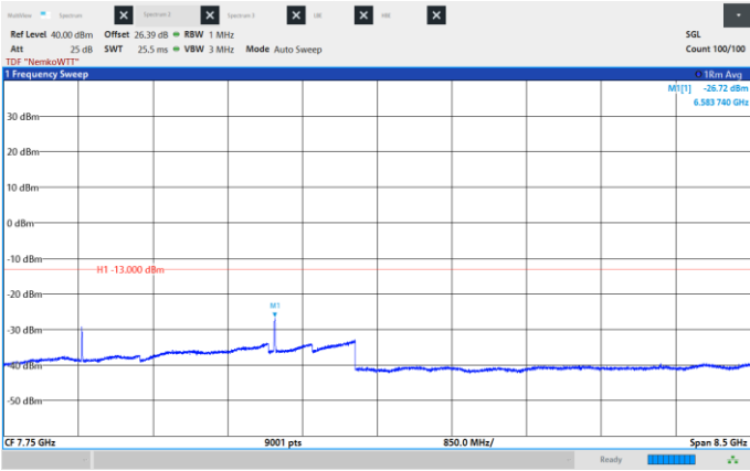
Figure 8.6-75: Conducted Spurious Emissions, High CH 2195 MHz, 10 MHz, 16QAM, Frequency range: 3.5 – 12.0 GHz
