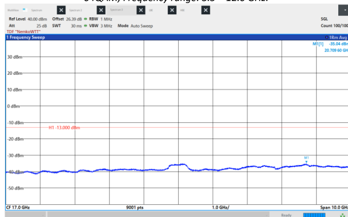
Figure 8.6-88: Conducted Spurious Emissions, High CH 2195 MHz, 10 MHz, 64QAM, Frequency range: 12.0 - 22.0 GHz
