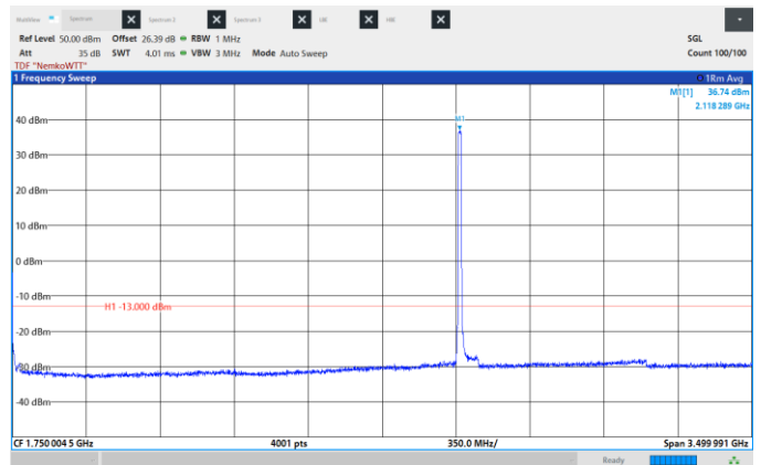
Figure 8.6-34: Conducted Spurious Emissions, Low CH 2117.5 MHz, 15 MHz, 256QAM, Frequency range: 0.009 -3500 MHz.
