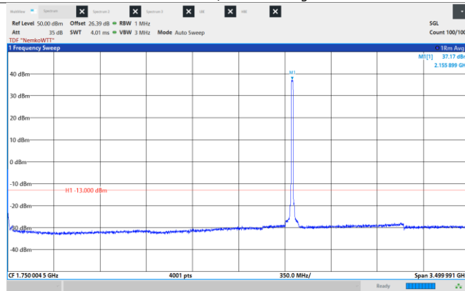
Figure 8.6-158: Conducted Spurious Emissions, Mid CH 2155 MHz, 15 MHz, 1024QAM, Frequency range: 0.009 - 3500 MHz.
