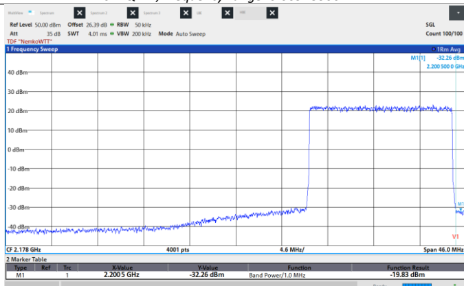
Figure 8.6-161: Conducted Spurious Emissions, High CH 2192.5 MHz, 15 MHz, 1024QAM, High band edge.
