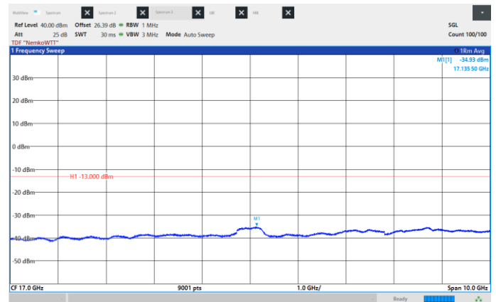
Figure 8.6-103: Conducted Spurious Emissions, Low CH 2115 MHz, 10 MHz, 1024QAM, Frequency range: 12.0 – 22.0 GHz.
