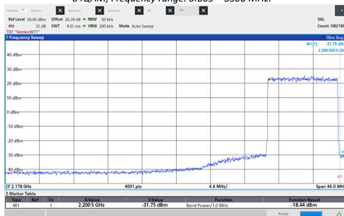
Figure 8.6-87: Conducted Spurious Emissions, High CH 2195 MHz, 10 MHz, 64QAM, High band edge.
