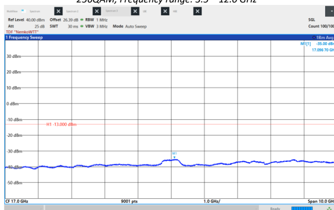
Figure 8.6-99: Conducted Spurious Emissions, High CH 2195 MHz, 10 MHz, 256QAM, Frequency range: 12.0 - 22.0 GHz.
