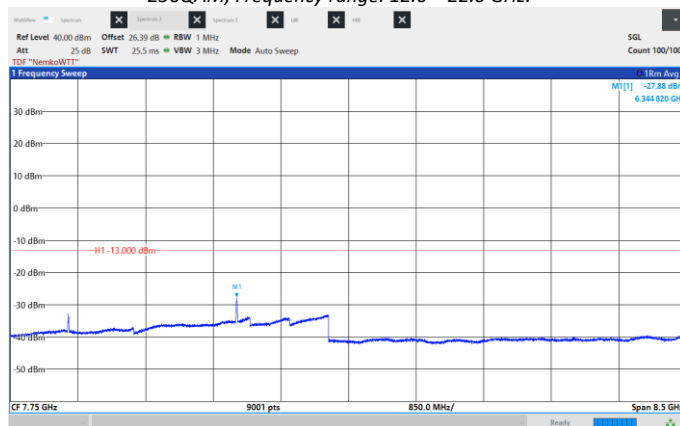
Figure 8.6-101: Conducted Spurious Emissions, Low CH 2115 MHz, 10 MHz, 1024QAM, Frequency range: 3.5 -12.0 GHz.
