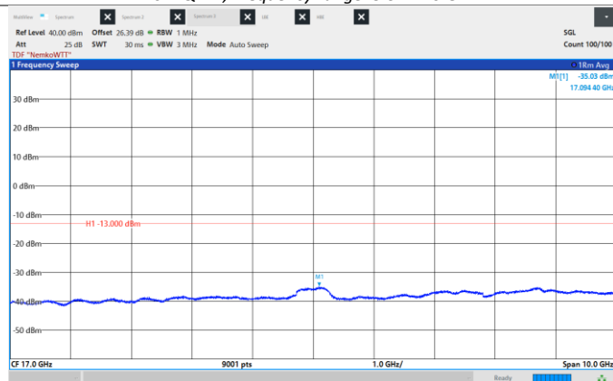
Figure 8.6-162: Conducted Spurious Emissions High CH 2192.5 MHz, 15 MHz, 1024QAM, Frequency range: 12.0 -22.0 GHz.
