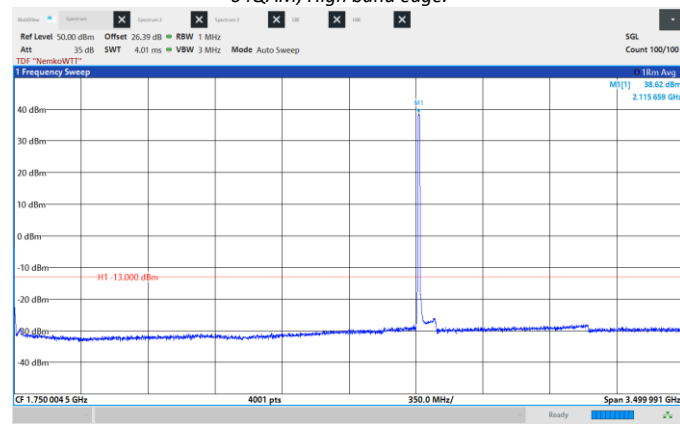
Figure 8.6-89: Conducted Spurious Emissions, Low CH 2115 MHz, 10 MHz, 256QAM, Frequency range: 0.009 - 3500 MHz.
