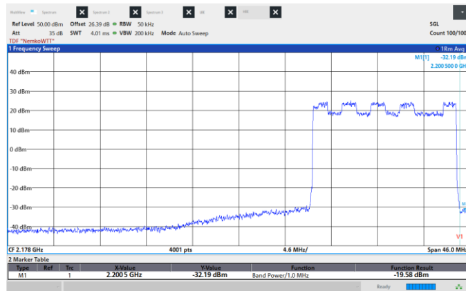
Figure 8.6-131: Conducted Spurious Emissions, High CH 2192.5 MHz, 15 MHz, 16QAM, High band edge
