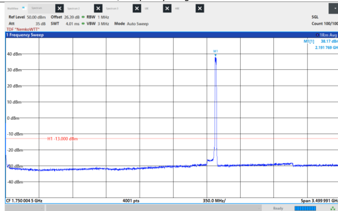
Figure 8.6-129: Conducted Spurious Emissions, High CH 2192.5 MHz, 15 MHz, 16QAM, Frequency range: 0.009 -3500 MHz.
