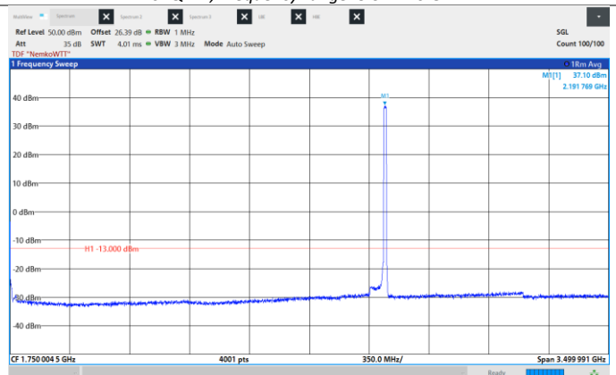
Figure 8.6-140: Conducted Spurious Emissions, High CH 2192.5 MHz, 15 MHz, 64QAM, Frequency range: 0.009 – 3500 MHz.
