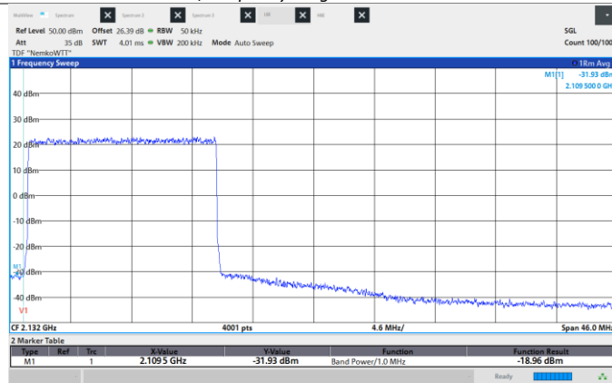
Figure 8.6-135: Conducted Spurious Emissions, Low CH 2117.5 MHz, 15 MHz, 64QAM, Low band edge
