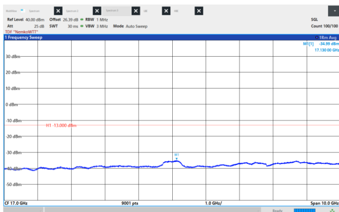
Figure 8.6-149: Conducted Spurious Emissions, Mid CH 2155 MHz, 15 MHz, 256QAM, Frequency range: 12.0 -22.0 GHz.
