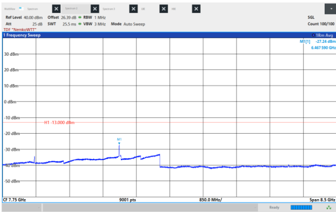
Figure 8.6-72: Conducted Spurious Emissions, Mid CH 2155 MHz, 10 MHz, 16QAM, Frequency range: 3.5 -12.0 GHz.
