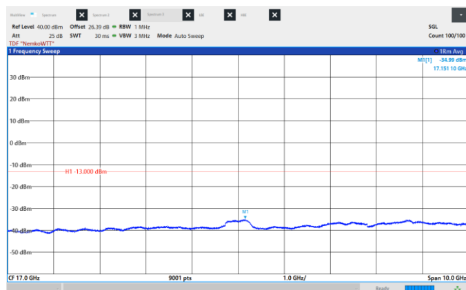
Figure 8.6-159: Conducted Spurious Emissions, Mid CH 2155 MHz, 15 MHz, 1024QAM, Frequency range: 12.0 -22.0 GHz.
