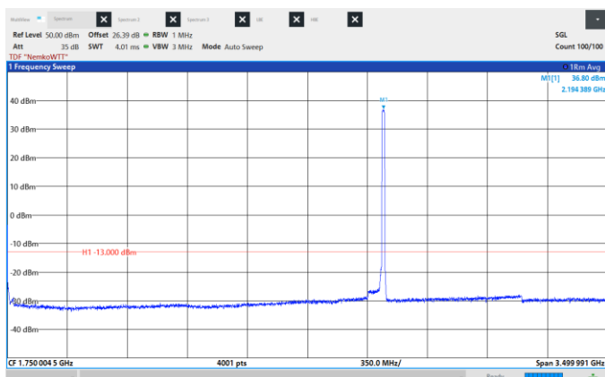
Figure 8.6-52: Conducted Spurious Emissions, High CH 2192.5 MHz, 15 MHz, 1024QAM, Frequency range: 0.009 -3500 MHz.
