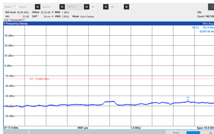
Figure 8.6-66: Conducted Spurious Emissions, High CH 2195 MHz, 10 MHz, QPSK, Frequency range: 12.0 -22.0 GHz
