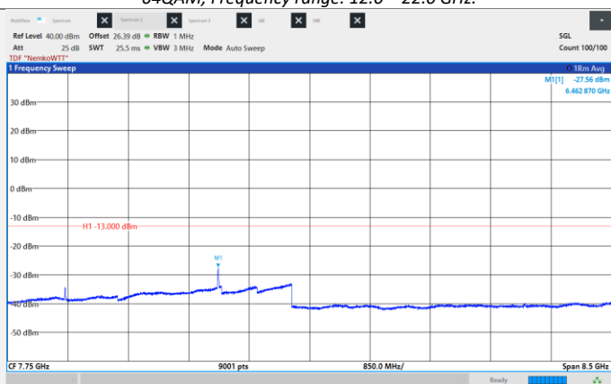
Figure 8.6-83: Conducted Spurious Emissions, Mid CH 2155 MHz, 10 MHz, 64QAM, Frequency range: 3.5 -12.0 GHz.
