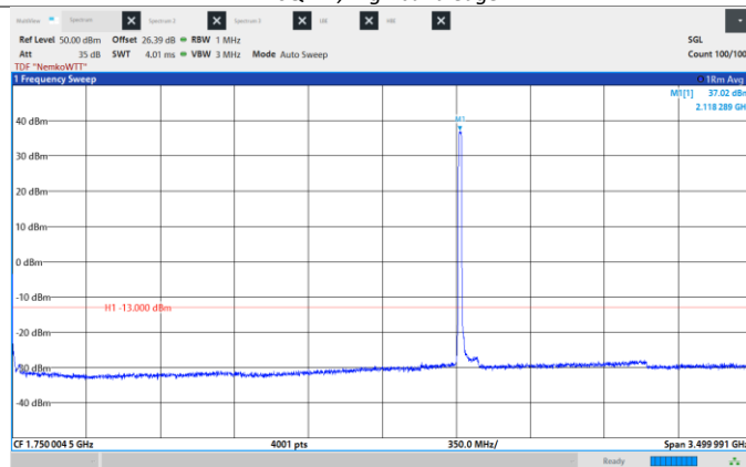
Figure 8.6-133: Conducted Spurious Emissions, Low CH 2117.5 MHz, 15 MHz, 64QAM, Frequency range: 0.009 -3500 MHz.
