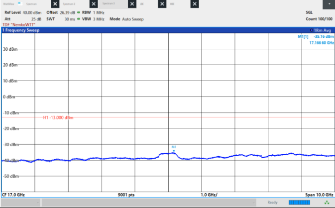
Figure 8.6-221: Conducted Spurious Emissions, Low CH 2122.5 MHz, 25 MHz, QPSK, Frequency range: 12.0 – 22.0 GHz.
