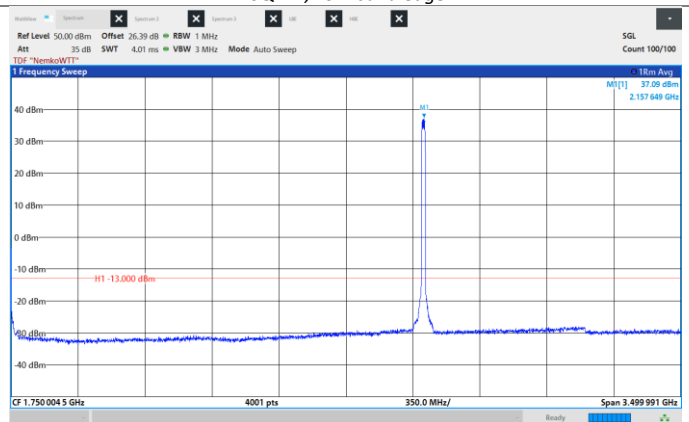
Figure 8.6-178: Conducted Spurious Emissions, Mid CH 2155 MHz, 20 MHz, 16QAM, Frequency range: 0.009 -3500 MHz
