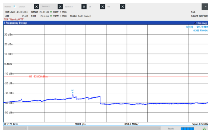
Figure 8.6-252: Conducted Spurious Emissions, Low CH 2122.5 MHz, 25 MHz, 256QAM, Frequency range: 3.5 – 12.0 GHz.
