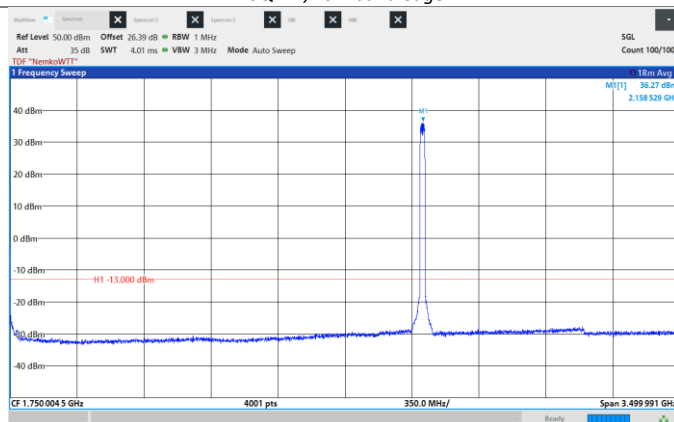
Figure 8.6-233: Conducted Spurious Emissions, Mid CH 2155 MHz, 25 MHz, 16QAM, Frequency range: 0.009 -3500 MHz
