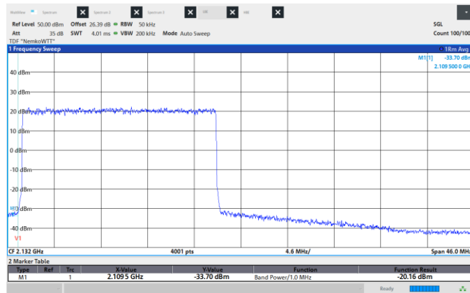
Figure 8.6-187: Conducted Spurious Emissions, Low CH 2120 MHz, 20 MHz, 64QAM, Low band edge
