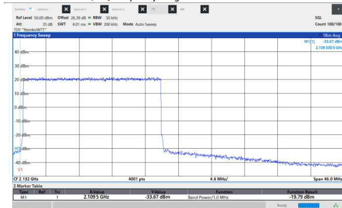
Figure 8.6-165: Conducted Spurious Emissions, Low CH 2120 MHz, 20 MHz, QPSK, Low band edge.
