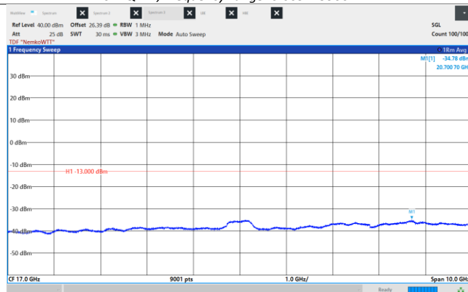
Figure 8.6-213: Conducted Spurious Emissions, Mid CH 2155 MHz, 20 MHz, 1024QAM, Frequency range: 12.0 -22.0 GHz.
