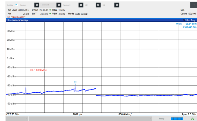
Figure 8.6-193: Conducted Spurious Emissions, High CH 2190 MHz, 20 MHz, 64QAM, Frequency range: 3.5 – 12.0 GHz.
