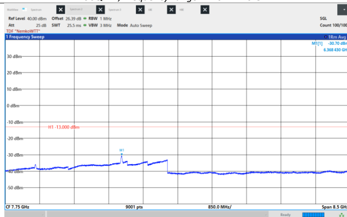
Figure 8.6-263: Conducted Spurious Emissions, Low CH 2122.5 MHz, 25 MHz, 1024QAM, Frequency range: 3.5 -12.0 GHz.
