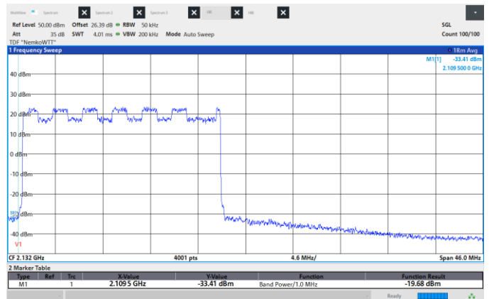
Figure 8.6-176: Conducted Spurious Emissions, Low CH 2120 MHz, 20 MHz, 16QAM, Low band edge.
