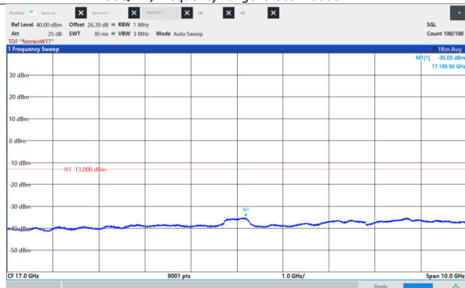
Figure 8.6-257: Conducted Spurious Emissions, Mid CH 2155 MHz, 25 MHz, 256QAM, Frequency range: 12.0 - 22.0 GHz.
