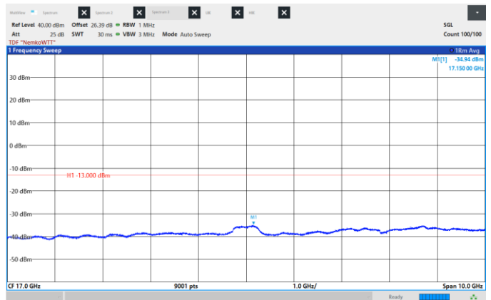
Figure 8.6-188: Conducted Spurious Emissions, Low CH 2120 MHz, 20 MHz, 64QAM, Frequency range: 12.0 – 22.0 GHz.
