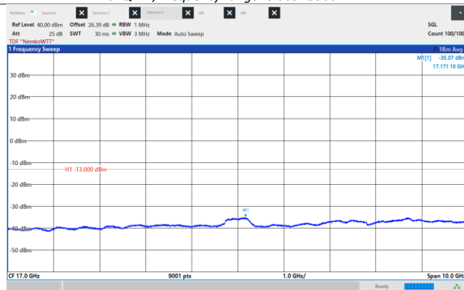
Figure 8.6-191: Conducted Spurious Emissions, Mid CH 2155 MHz, 20 MHz, 64QAM, Frequency range: 12.0 – 22.0 GHz.
