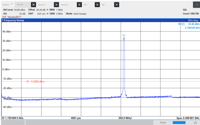
Figure 8.6-222: Conducted Spurious Emissions, Mid CH 2155 MHz, 25 MHz, QPSK, Frequency range: 0.009 -3500 MHz.
