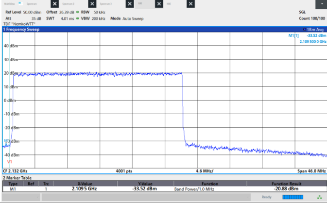
Figure 8.6-220: Conducted Spurious Emissions, Low CH 2122.5 MHz, 25 MHz, QPSK, Low band edge.
