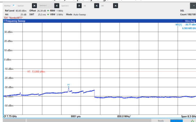
Figure 8.6-230: Conducted Spurious Emissions, Low CH 2122.5 MHz, 25 MHz, 16QAM, Frequency range: 3.5 – 12.0 GHz.
