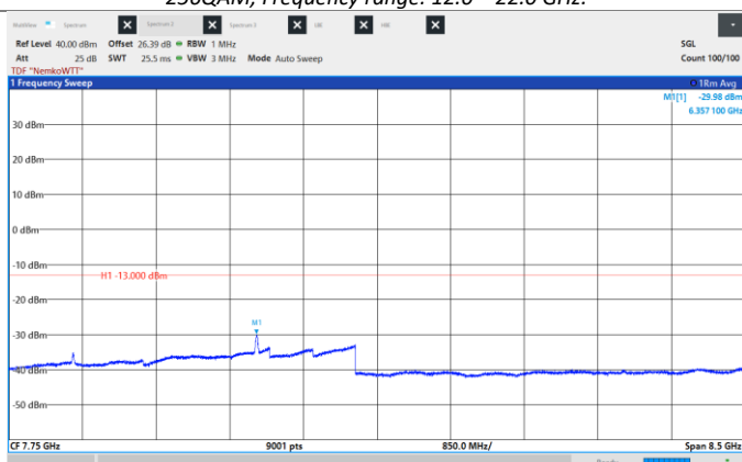
Figure 8.6-208: Conducted Spurious Emissions, Low CH 2120 MHz, 20 MHz, 1024QAM, Frequency range: 3.5 -12.0 GHz.
