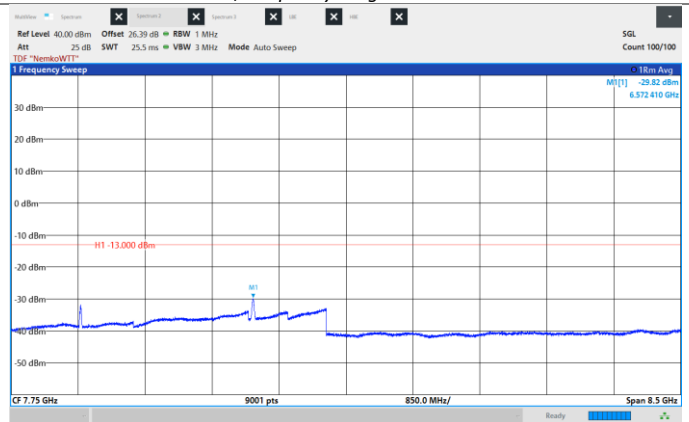
Figure 8.6-204: Conducted Spurious Emissions, High CH 2190 MHz, 20 MHz, 256QAM, Frequency range: 3.5 – 12.0 GHz
