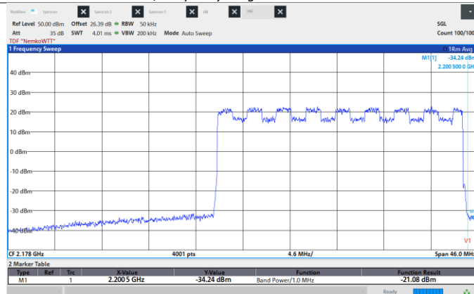
Figure 8.6-238: Conducted Spurious Emissions, High CH 2187.5 MHz, 25 MHz, 16QAM, High band edge
