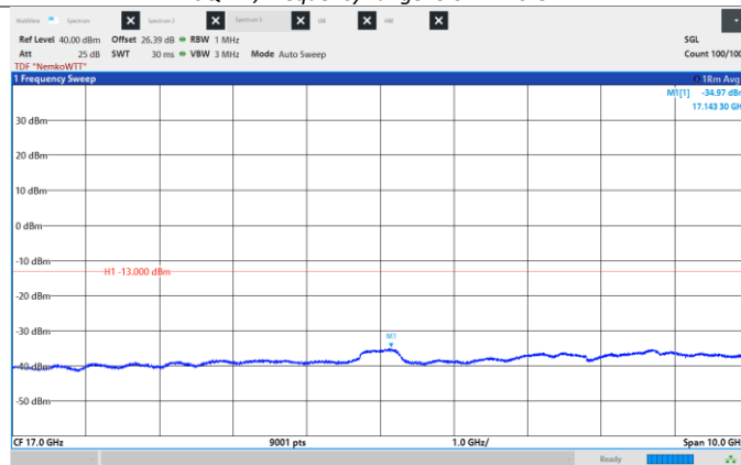
Figure 8.6-177: Conducted Spurious Emissions, Low CH 2120 MHz, 20 MHz, 16QAM, Frequency range: 12.0 - 22.0 GHz
