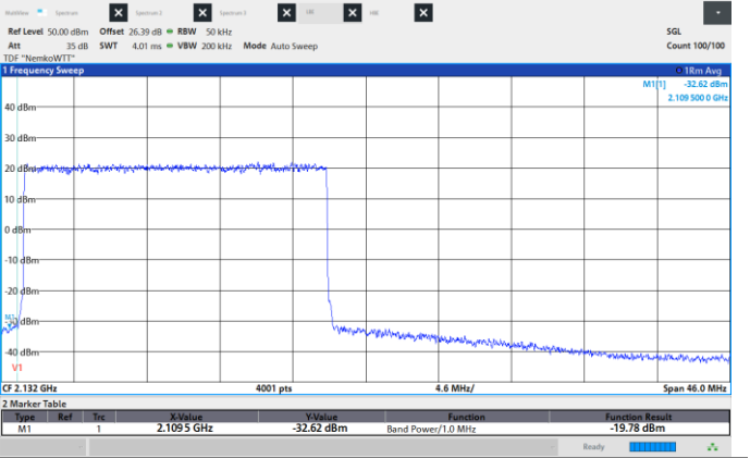
Figure 8.6-198: Conducted Spurious Emissions, Low CH 2120 MHz, 20 MHz, 256QAM, Low band edge.
