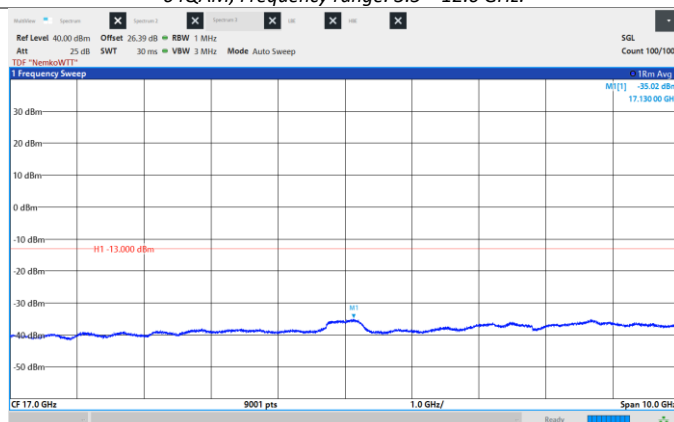
Figure 8.6-243: Conducted Spurious Emissions, Low CH 2122.5 MHz, 25 MHz, 64QAM, Frequency range: 12.0 - 22.0 GHz.
