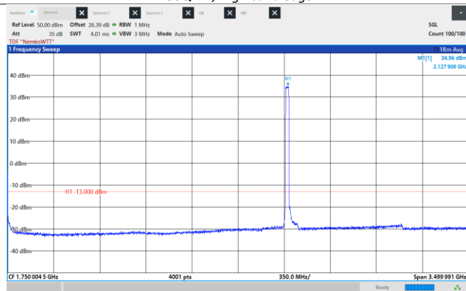
Figure 8.6-262: Conducted Spurious Emissions, Low CH 2122.5 MHz, 25 MHz, 1024QAM, Frequency range: 0.009 -3500 MHz.
