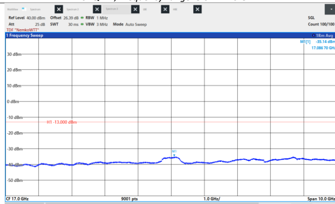
Figure 8.6-250: Conducted Spurious Emissions, High CH 2187.5 MHz, 25 MHz, 64QAM, Frequency range: 12.0 - 22.0 GHz
