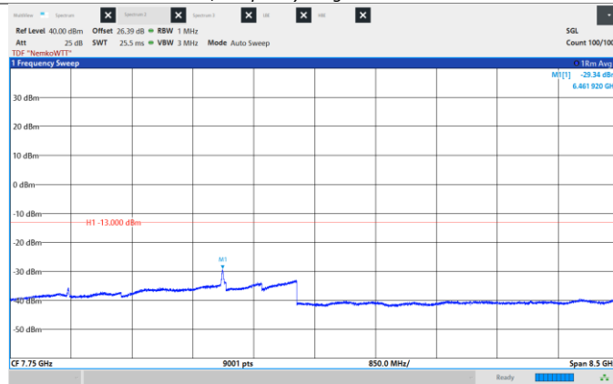
Figure 8.6-179: Conducted Spurious Emissions, Mid CH 2155 MHz, 20 MHz, 16QAM, Frequency range: 3.5 -12.0 GHz.
