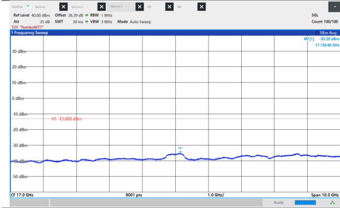
Figure 8.6-195: Conducted Spurious Emissions, High CH 2190 MHz, 20 MHz, 64QAM, Frequency range: 12.0 - 22.0 GHz
