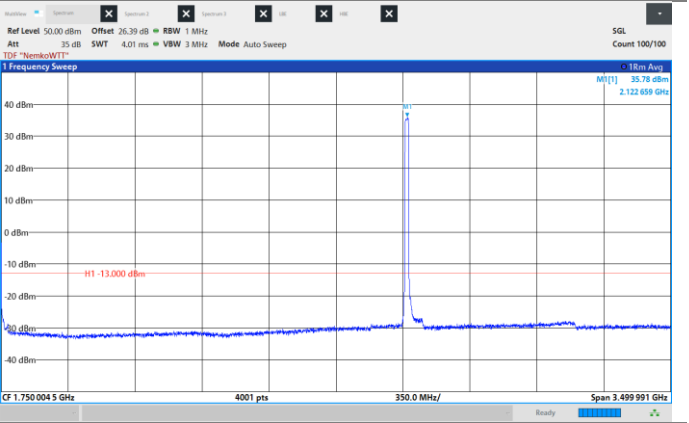
Figure 8.6-196: Conducted Spurious Emissions, Low CH 2120 MHz, 20 MHz, 256QAM, Frequency range: 0.009 - 3500 MHz.
