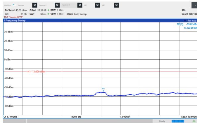
Figure 8.6-199: Conducted Spurious Emissions, Low CH 2120 MHz, 20 MHz, 256QAM, Frequency range: 12.0 – 22.0 GHz.
