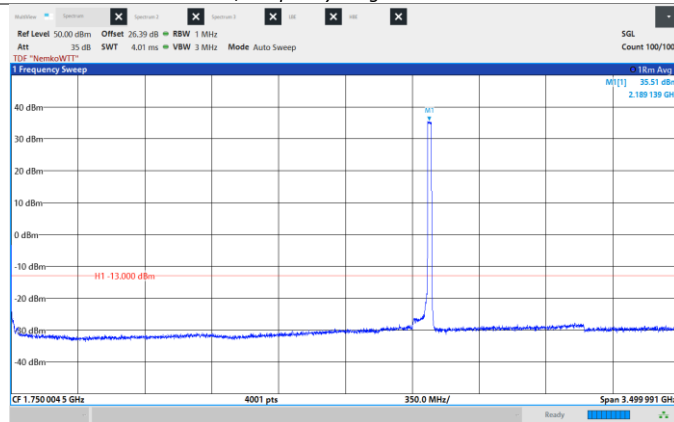
Figure 8.6-203: Conducted Spurious Emissions, High CH 2190 MHz, 20 MHz, 256QAM, Frequency range: 0.009 - 3500 MHz.
