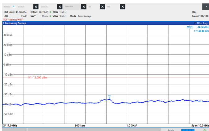
Figure 8.6-206: Conducted Spurious Emissions, High CH 2190 MHz, 20 MHz, 256QAM, Frequency range: 12.0 – 22.0 GHz.
