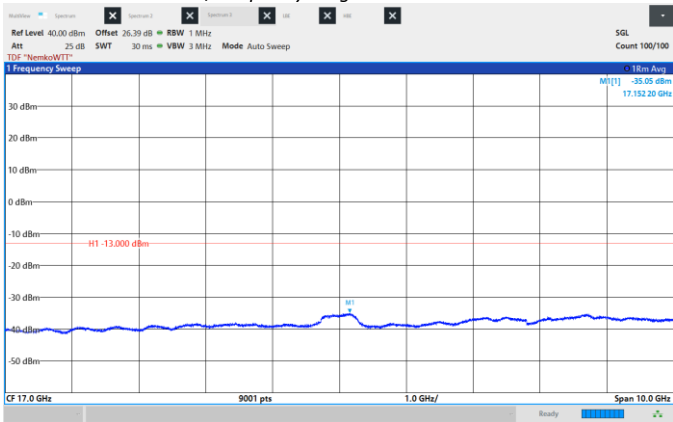
Figure 8.6-224: Conducted Spurious Emissions, Mid CH 2155 MHz, 25 MHz, QPSK, Frequency range: 12.0 – 22.0 GHz.
