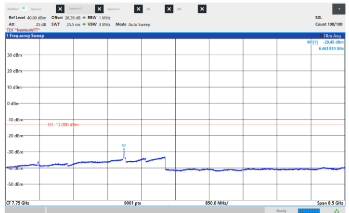
Figure 8.6-212: Conducted Spurious Emissions, Mid CH 2155 MHz, 20 MHz, 1024QAM, Frequency range: 3.5 – 12.0 GHz.
