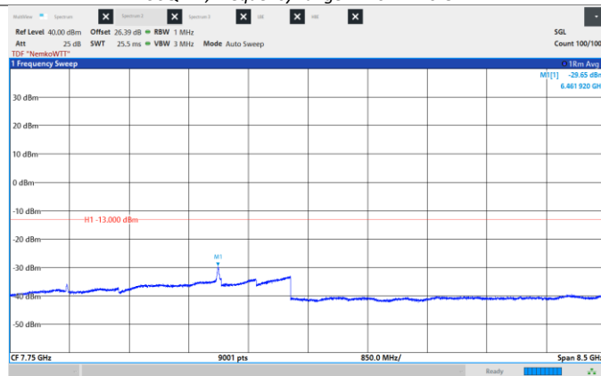
Figure 8.6-201: Conducted Spurious Emissions, Mid CH 2155 MHz, 20 MHz, 256QAM, Frequency range: 3.5 – 12.0 GHz.
