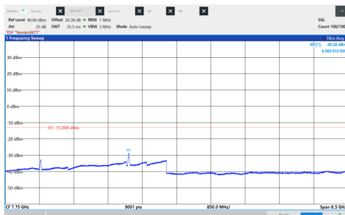
Figure 8.6-259: Conducted Spurious Emissions, High CH 2187.5 MHz, 25 MHz, 256QAM, Frequency range: 3.5 - 12.0 GHz
