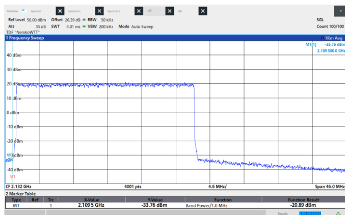
Figure 8.6-253: Conducted Spurious Emissions, Low CH 2122.5 MHz, 25 MHz, 256QAM, Low band edge.
