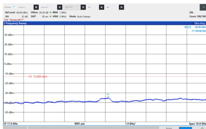
Figure 8.6-228: Conducted Spurious Emissions, High CH 2187.5 MHz, 25 MHz, QPSK, Frequency range: 12.0 -22.0 GHz
