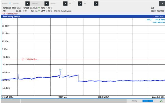
Figure 8.6-226: Conducted Spurious Emissions, High CH 2187.5 MHz, 25 MHz, QPSK, Frequency range: 3.5 -12.0 GHz.
