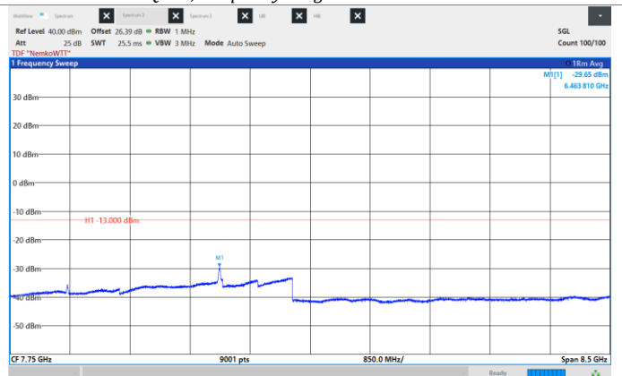
Figure 8.6-168: Conducted Spurious Emissions, Mid CH 2155 MHz, 20 MHz, QPSK, Frequency range: 3.5 -12.0 GHz.
