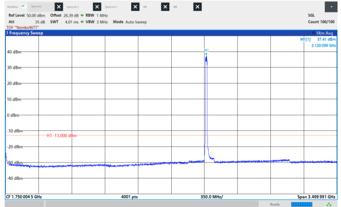
Figure 8.6-174: Conducted Spurious Emissions, Low CH 2120 MHz, 20 MHz, 16QAM, Frequency range: 0.009 – 3500 MHz.
