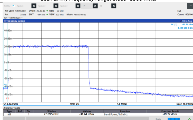
Figure 8.6-209: Conducted Spurious Emissions, Low CH 2120 MHz, 20 MHz, 1024QAM, Low band edge.
