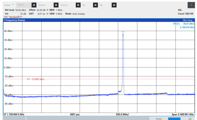
Figure 8.6-170: Conducted Spurious Emissions, High CH 2190 MHz, 20 MHz, QPSK, Frequency range: 0.009 – 3500 MHz.
