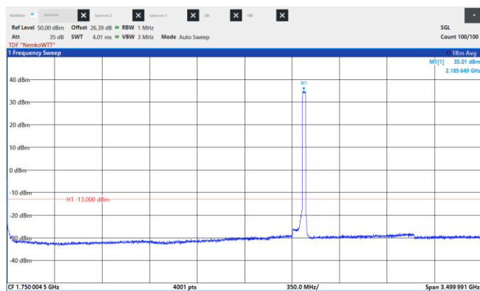
Figure 8.6-247: Conducted Spurious Emissions, High CH 2187.5 MHz, 25 MHz, 64QAM, Frequency range: 0.009 – 3500 MHz.
