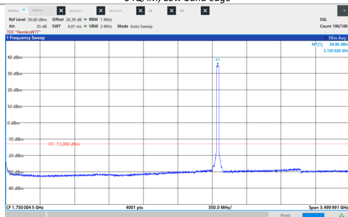
Figure 8.6-244: Conducted Spurious Emissions, Mid CH 2155 MHz, 25 MHz, 64QAM, Frequency range: 0.009 -3500 MHz
