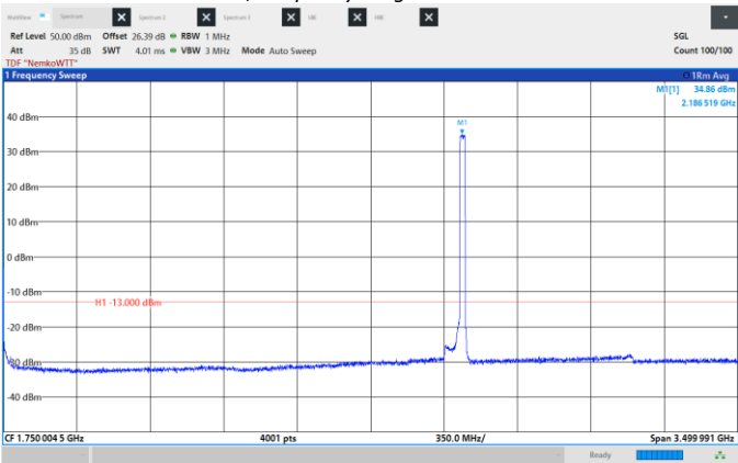
Figure 8.6-225: Conducted Spurious Emissions, High CH 2187.5 MHz, 25 MHz, QPSK, Frequency range: 0.009 – 3500 MHz.
