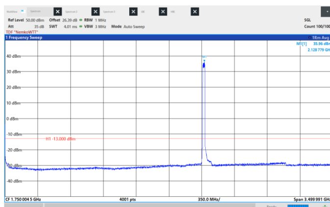
Figure 8.6-229: Conducted Spurious Emissions, Low CH 2122.5 MHz, 25 MHz, 16QAM, Frequency range: 0.009 – 3500 MHz.
