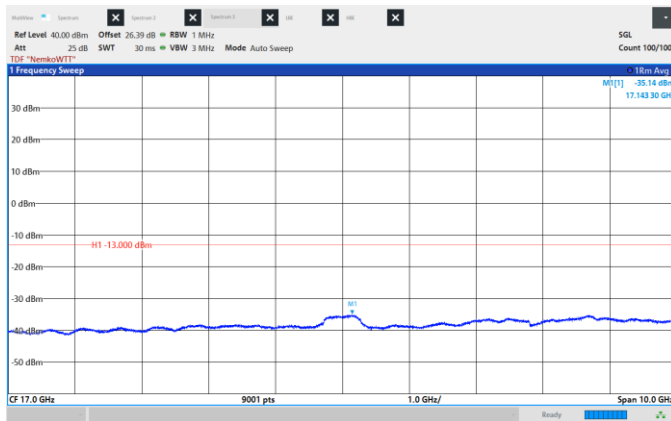
Figure 8.6-169: Conducted Spurious Emissions, Mid CH 2155 MHz, 20 MHz, QPSK, Frequency range: 12.0 – 22.0 GHz.
