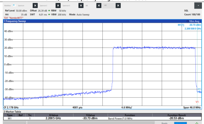
Figure 8.6-216: Conducted Spurious Emissions, High CH 2190 MHz, 20 MHz, 1024QAM, High band edge.
