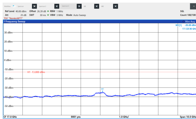
Figure 8.6-246: Conducted Spurious Emissions, Mid CH 2155 MHz, 25 MHz, 64QAM, Frequency range: 12.0 – 22.0 GHz.
