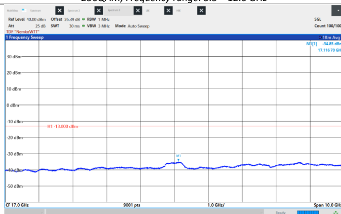
Figure 8.6-261: Conducted Spurious Emissions, High CH 2187.5 MHz, 25 MHz, 256QAM, Frequency range: 12.0 - 22.0 GHz.
