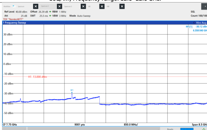
Figure 8.6-186: Conducted Spurious Emissions, Low CH 2120 MHz, 20 MHz, 64QAM, Frequency range: 3.5 - 12.0 GHz.
