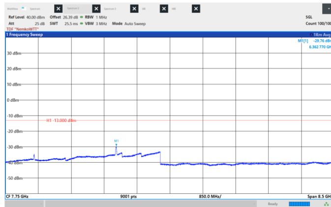
Figure 8.6-175: Conducted Spurious Emissions, Low CH 2120 MHz, 20 MHz, 16QAM, Frequency range: 3.5 – 12.0 GHz.
