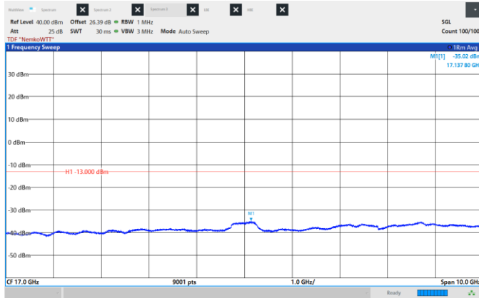
Figure 8.6-173: Conducted Spurious Emissions, High CH 2190 MHz, 20 MHz, QPSK, Frequency range: 12.0 -22.0 GHz
