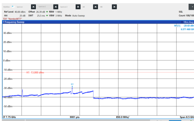
Figure 8.6-182: Conducted Spurious Emissions, High CH 2190 MHz, 20 MHz, 16QAM, Frequency range: 3.5 - 12.0 GHz
