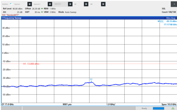
Figure 8.6-217: Conducted Spurious Emissions High CH 2190 MHz, 20 MHz, 1024QAM, Frequency range: 12.0 -22.0 GHz.
