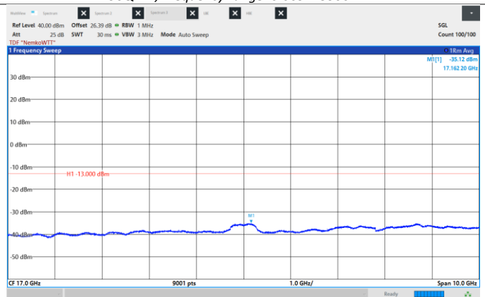
Figure 8.6-202: Conducted Spurious Emissions, Mid CH 2155 MHz, 20 MHz, 256QAM, Frequency range: 12.0 - 22.0 GHz.
