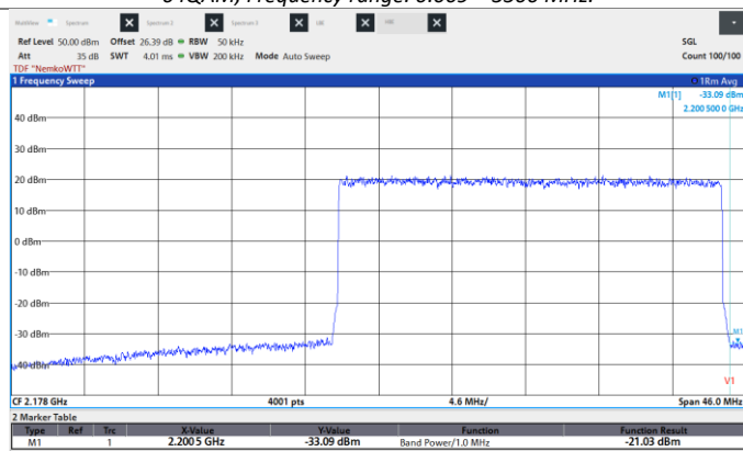
Figure 8.6-249: Conducted Spurious Emissions, High CH 2187.5 MHz, 25 MHz, 64QAM, High band edge.
