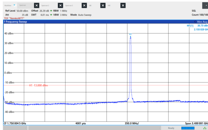
Figure 8.6-211: Conducted Spurious Emissions, Mid CH 2155 MHz, 20 MHz, 1024QAM, Frequency range: 0.009 – 3500 MHz.
