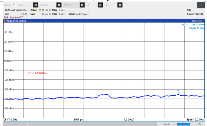
Figure 8.6-180: Conducted Spurious Emissions, Mid CH 2155 MHz, 20 MHz, 16QAM, Frequency range: 12.0 – 22.0 GHz.
