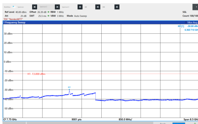
Figure 8.6-241: Conducted Spurious Emissions, Low CH 2122.5 MHz, 25 MHz, 64QAM, Frequency range: 3.5 - 12.0 GHz.
