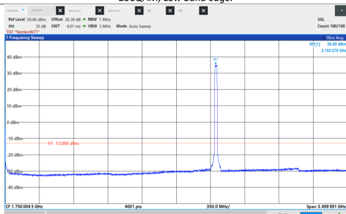
Figure 8.6-255: Conducted Spurious Emissions, Mid CH 2155 MHz, 25 MHz, 256QAM, Frequency range: 0.009 – 3500 MHz.
