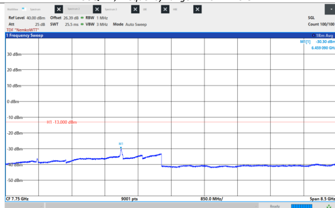
Figure 8.6-256: Conducted Spurious Emissions, Mid CH 2155 MHz, 25 MHz, 256QAM, Frequency range: 3.5 – 12.0 GHz.
