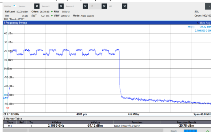
Figure 8.6-231: Conducted Spurious Emissions, Low CH 2122.5 MHz, 25 MHz, 16QAM, Low band edge.
