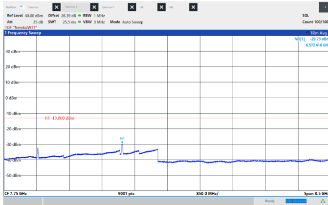
Figure 8.6-171: Conducted Spurious Emissions, High CH 2190 MHz, 20 MHz, QPSK, Frequency range: 3.5 -12.0 GHz.
