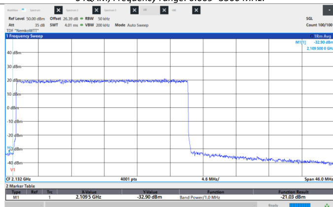
Figure 8.6-242: Conducted Spurious Emissions, Low CH 2122.5 MHz, 25 MHz, 64QAM, Low band edge
