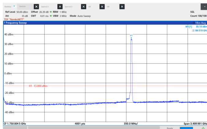
Figure 8.6-258: Conducted Spurious Emissions, High CH 2187.5 MHz, 25 MHz, 256QAM, Frequency range: 0.009 -3500 MHz.
