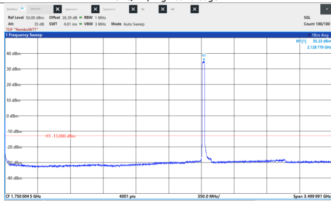
Figure 8.6-251: Conducted Spurious Emissions, Low CH 2122.5 MHz, 25 MHz, 256QAM, Frequency range: 0.009 - 3500 MHz.
