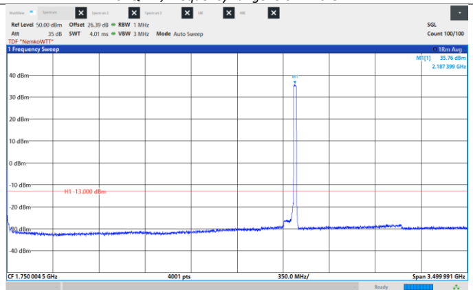
Figure 8.6-192: Conducted Spurious Emissions, High CH 2190 MHz, 20 MHz, 64QAM, Frequency range: 0.009 – 3500 MHz.
