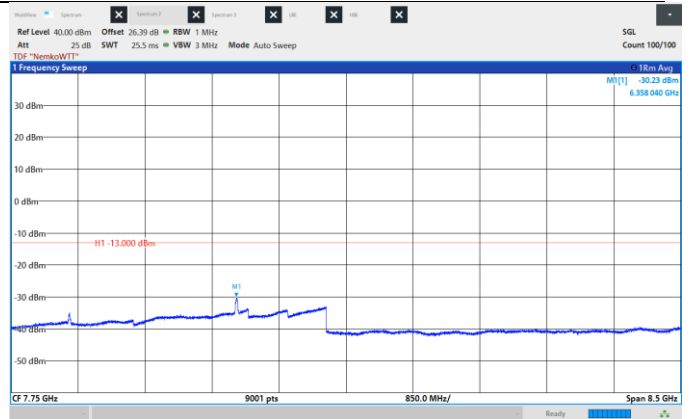
Figure 8.6-164: Conducted Spurious Emissions, Low CH 2120 MHz, 20 MHz, QPSK, Frequency range: 3.5 -12.0 GHz.
