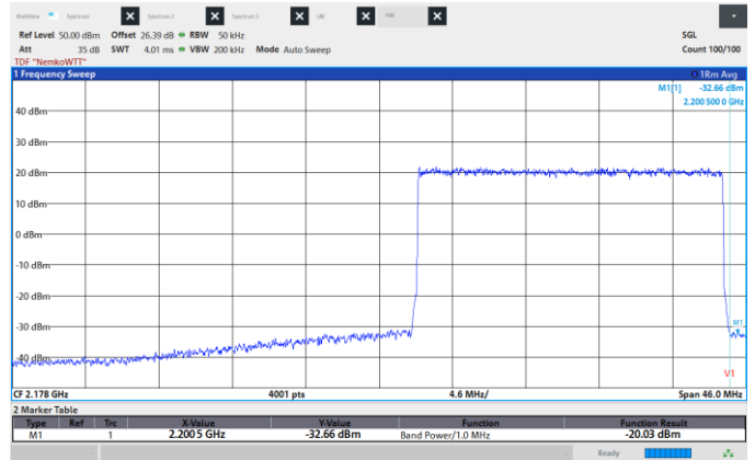
Figure 8.6-172: Conducted Spurious Emissions, High CH 2190 MHz, 20 MHz, QPSK, High band edge.
