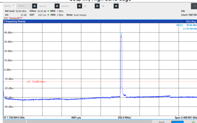
Figure 8.6-185: Conducted Spurious Emissions, Low CH 2120 MHz, 20 MHz, 64QAM, Frequency range: 0.009 -3500 MHz.
