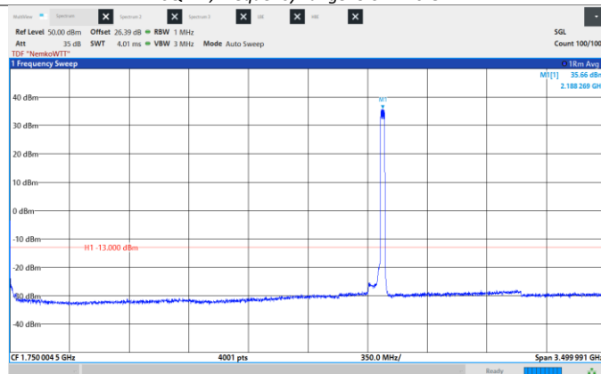
Figure 8.6-236: Conducted Spurious Emissions, High CH 2187.5 MHz, 25 MHz, 16QAM, Frequency range: 0.009 -3500 MHz.
