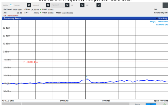
Figure 8.6-210: Conducted Spurious Emissions, Low CH 2120 MHz, 20 MHz, 1024QAM, Frequency range: 12.0 – 22.0 GHz.
