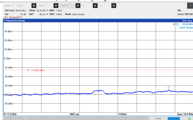
Figure 8.6-232: Conducted Spurious Emissions, Low CH 2122.5 MHz, 25 MHz, 16QAM, Frequency range: 12.0 -22.0 GHz
