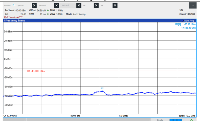
Figure 8.6-166: Conducted Spurious Emissions, Low CH 2120 MHz, 20 MHz, QPSK, Frequency range: 12.0 – 22.0 GHz.
