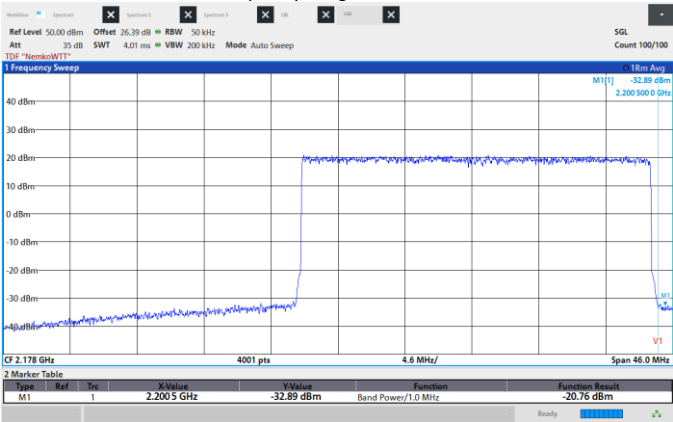
Figure 8.6-227: Conducted Spurious Emissions, High CH 2187.5 MHz, 25 MHz, QPSK, High band edge.
