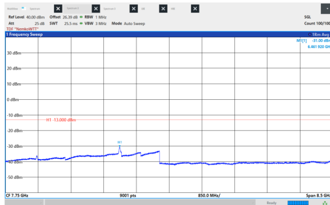
Figure 8.6-234: Conducted Spurious Emissions, Mid CH 2155 MHz, 25 MHz, 16QAM, Frequency range: 3.5 -12.0 GHz.
