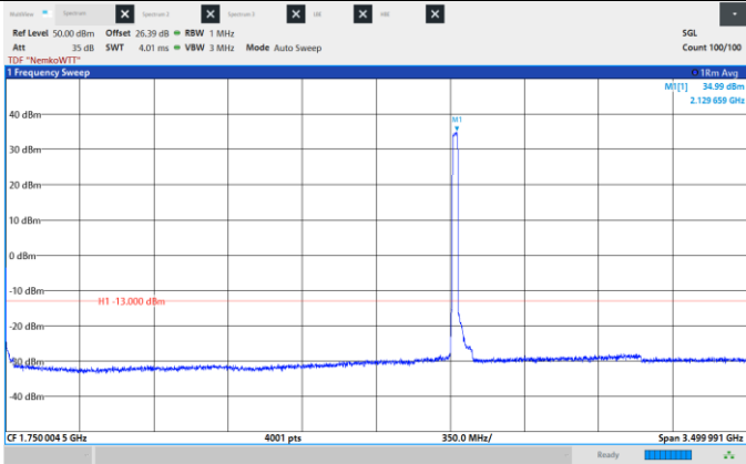
Figure 8.6-218: Conducted Spurious Emissions, Low CH 2122.5 MHz, 25 MHz, QPSK, Frequency range: 0.009 – 3500 MHz.
