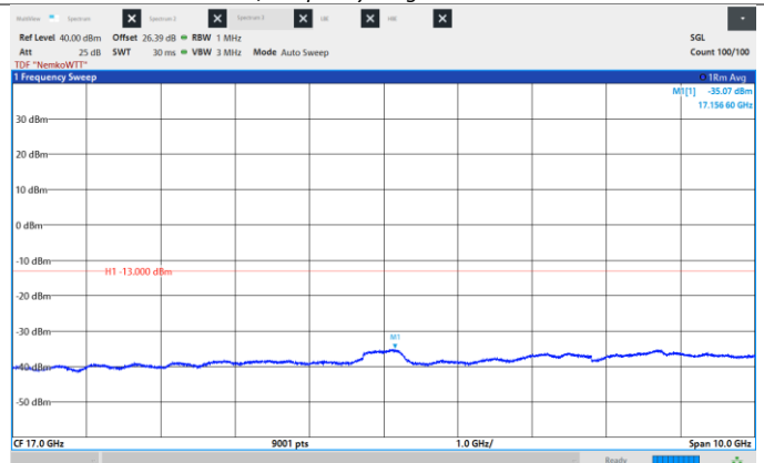
Figure 8.6-239: Conducted Spurious Emissions, High CH 2187.5 MHz, 25 MHz, 16QAM, Frequency range: 12.0 -22.0 GHz.
