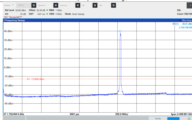
Figure 8.6-189: Conducted Spurious Emissions, Mid CH 2155 MHz, 20 MHz, 64QAM, Frequency range: 0.009 -3500 MHz
