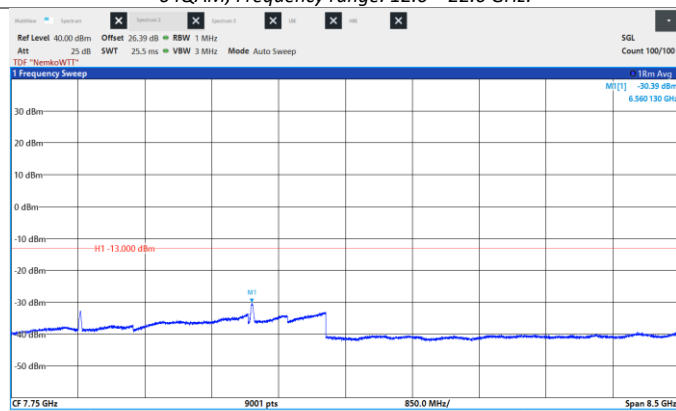
Figure 8.6-248: Conducted Spurious Emissions, High CH 2187.5 MHz, 25 MHz, 64QAM, Frequency range: 3.5 – 12.0 GHz.
