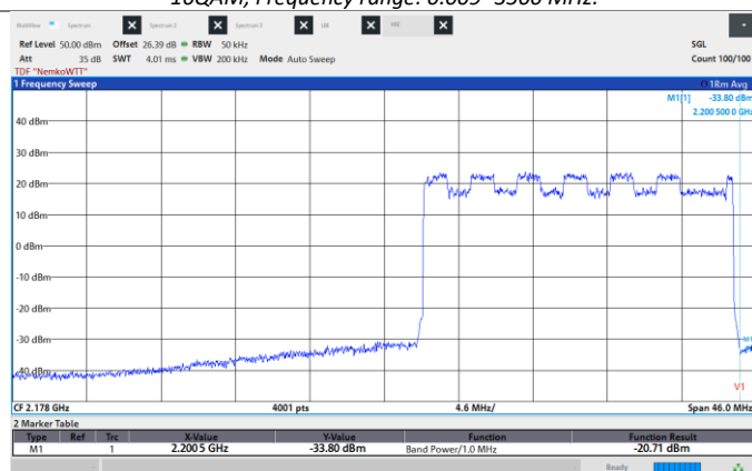
Figure 8.6-183: Conducted Spurious Emissions, High CH 2190 MHz, 20 MHz, 16QAM, High band edge
