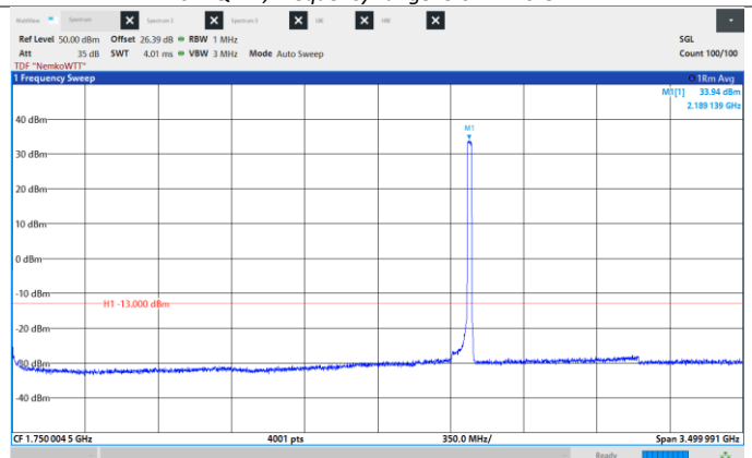
Figure 8.6-214: Conducted Spurious Emissions, High CH 2190 MHz, 20 MHz, 1024QAM, Frequency range: 0.009 -3500 MHz.
