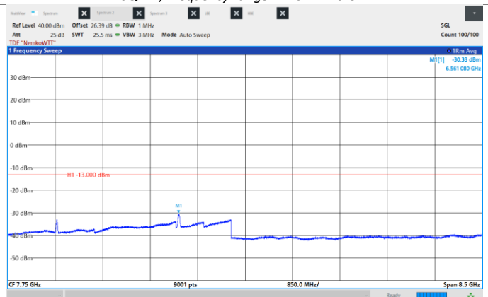
Figure 8.6-237: Conducted Spurious Emissions, High CH 2187.5 MHz, 25 MHz, 16QAM, Frequency range: 3.5 - 12.0 GHz
