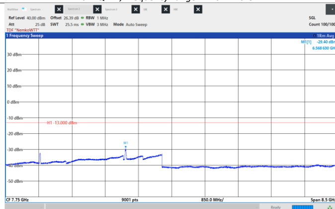
Figure 8.6-215: Conducted Spurious Emissions, High CH 2190 MHz, 20 MHz, 1024QAM, Frequency range: 3.5 -12.0 GHz.
