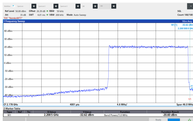
Figure 8.6-205: Conducted Spurious Emissions, High CH 2190 MHz, 20 MHz, 256QAM, High band edge.
