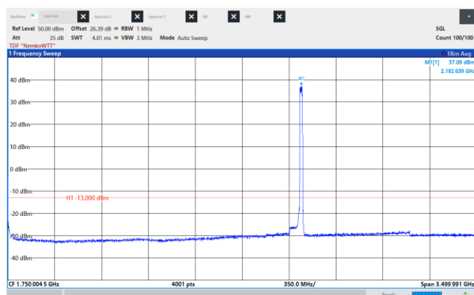
Figure 8.6-181: Conducted Spurious Emissions, High CH 2190 MHz, 20 MHz, 16QAM, Frequency range: 0.009 -3500 MHz.
