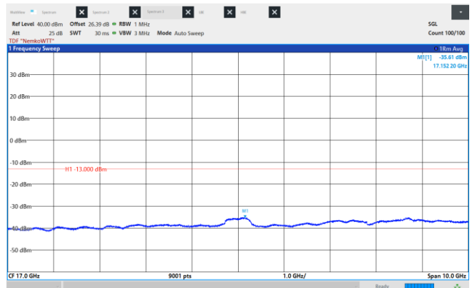
Figure 8.6-235: Conducted Spurious Emissions, Mid CH 2155 MHz, 25 MHz, 16QAM, Frequency range: 12.0 - 22.0 GHz.
