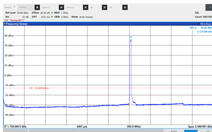
Figure 8.6-240: Conducted Spurious Emissions, Low CH 2122.5 MHz, 25 MHz, 64QAM, Frequency range: 0.009 -3500 MHz.
