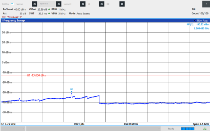
Figure 8.6-219: Conducted Spurious Emissions, Low CH 2122.5 MHz, 25 MHz, QPSK, Frequency range: 3.5 -12.0 GHz.
