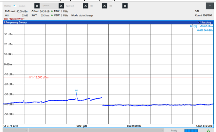
Figure 8.6-190: Conducted Spurious Emissions, Mid CH 2155 MHz, 20 MHz, 64QAM, Frequency range: 3.5 -12.0 GHz.
