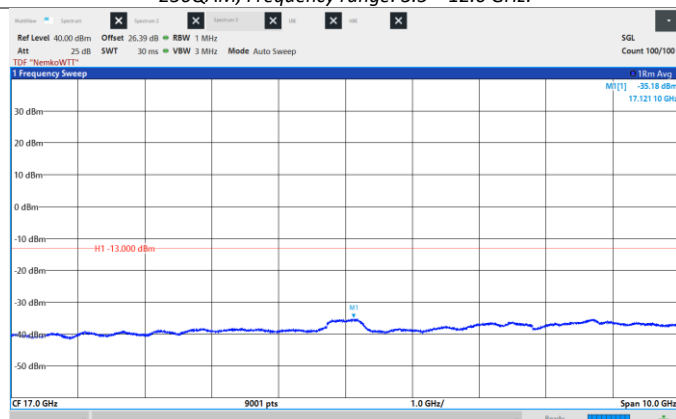
Figure 8.6-254: Conducted Spurious Emissions, Low CH 2122.5 MHz, 25 MHz, 256QAM, Frequency range: 12.0 – 22.0 GHz.
