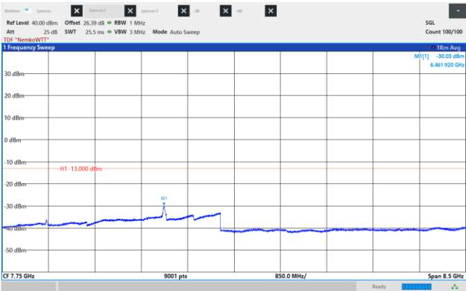
Figure 8.6-223: Conducted Spurious Emissions, Mid CH 2155 MHz, 25 MHz, QPSK, Frequency range: 3.5 -12.0 GHz.
