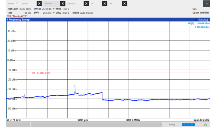
Figure 8.6-197: Conducted Spurious Emissions, Low CH 2120 MHz, 20 MHz, 256QAM, Frequency range: 3.5 – 12.0 GHz.
