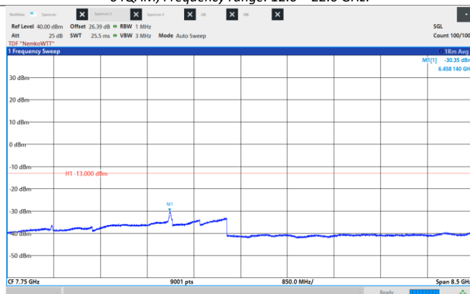
Figure 8.6-245: Conducted Spurious Emissions, Mid CH 2155 MHz, 25 MHz, 64QAM, Frequency range: 3.5 -12.0 GHz.
