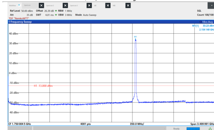
Figure 8.6-167: Conducted Spurious Emissions, Mid CH 2155 MHz, 20 MHz, QPSK, Frequency range: 0.009 -3500 MHz.
