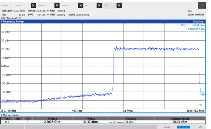
Figure 8.6-194: Conducted Spurious Emissions, High CH 2190 MHz, 20 MHz, 64QAM, High band edge.
