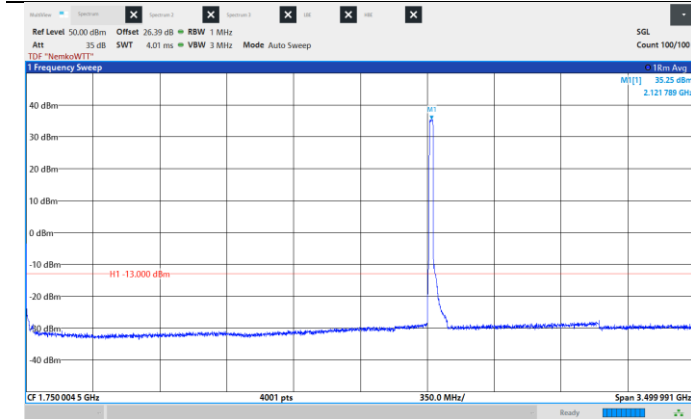
Figure 8.6-163: Conducted Spurious Emissions, Low CH 2120 MHz, 20 MHz, QPSK, Frequency range: 0.009 – 3500 MHz.
