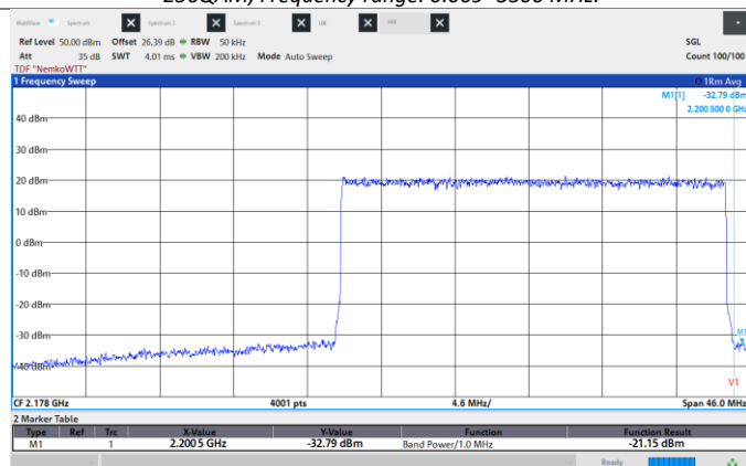
Figure 8.6-260: Conducted Spurious Emissions, High CH 2187.5 MHz, 25 MHz, 256QAM, High band edge.
