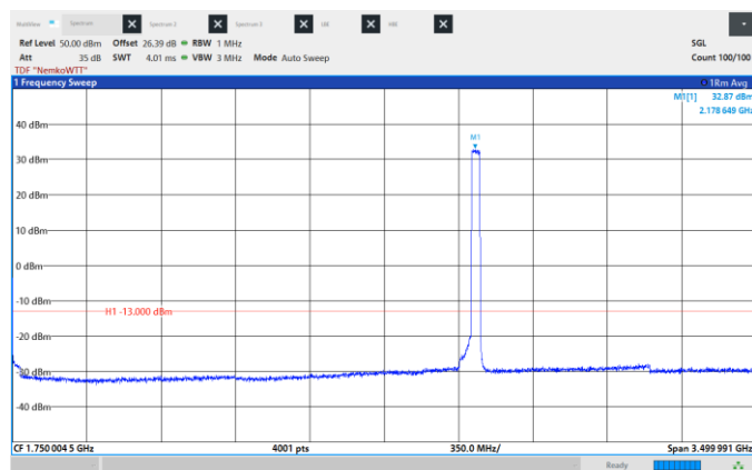
Figure 8.6-423: Conducted Spurious Emissions, High CH 2180 MHz, 40 MHz, 256QAM, Frequency range: 0.009 -3500 MHz.
