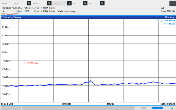
Figure 8.6-404: Conducted Spurious Emissions, High CH 2180 MHz, 40 MHz, 16QAM, Frequency range: 12.0 -22.0 GHz.
