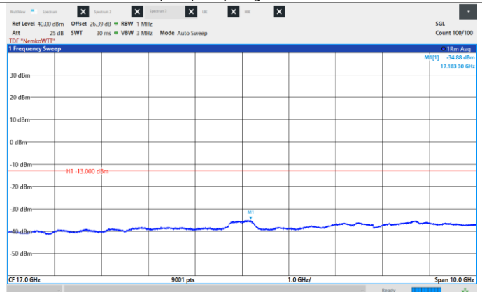
Figure 8.6-463: Conducted Spurious Emissions, Low CH 2132.5 MHz, 45 MHz, 64QAM, Frequency range: 12.0 - 22.0 GHz.
