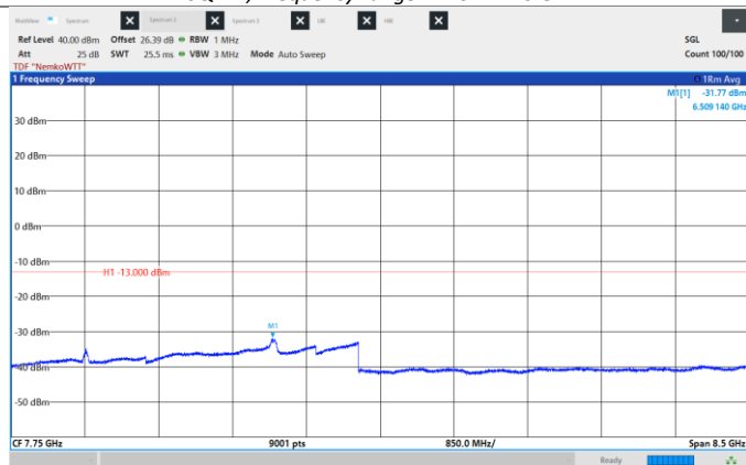
Figure 8.6-457: Conducted Spurious Emissions, High CH 2177.5 MHz, 45 MHz, 16QAM, Frequency range: 3.5 - 12.0 GHz
