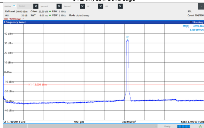
Figure 8.6-409: Conducted Spurious Emissions, Mid CH 2155 MHz, 40 MHz, 64QAM, Frequency range: 0.009 -3500 MHz
