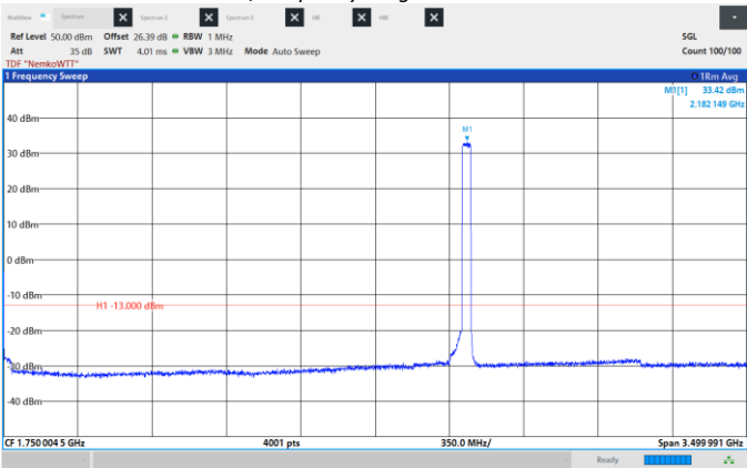
Figure 8.6-390: Conducted Spurious Emissions, High CH 2180 MHz, 40 MHz, QPSK, Frequency range: 0.009 – 3500 MHz.
