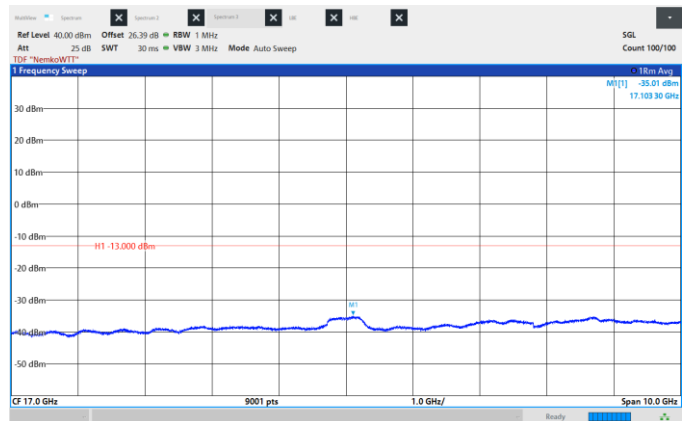
Figure 8.6-430: Conducted Spurious Emissions, Low CH 2130 MHz, 40 MHz, 1024QAM, Frequency range: 12.0 – 22.0 GHz.
