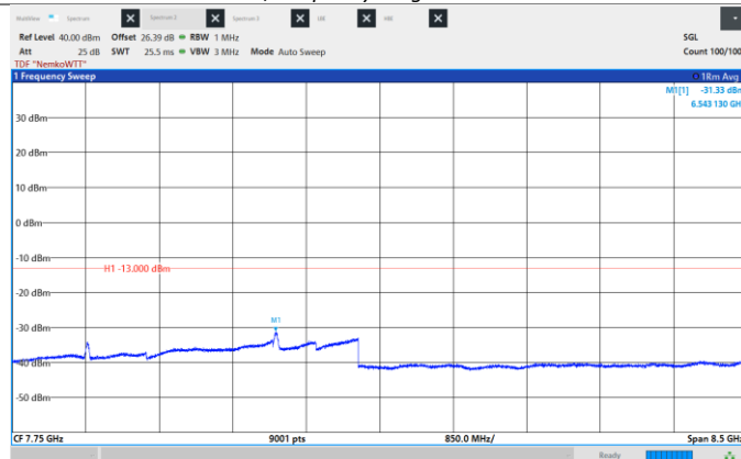
Figure 8.6-380: Conducted Spurious Emissions, High CH 2182.5 MHz, 35 MHz, 1024QAM, Frequency range: 3.5 -12.0 GHz.
