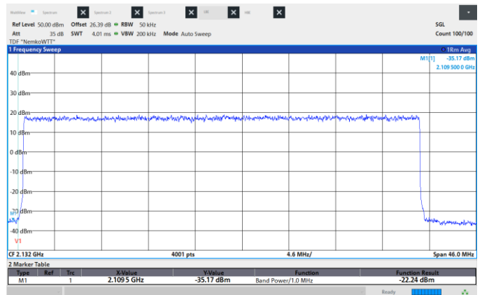
Figure 8.6-418: Conducted Spurious Emissions, Low CH 2130 MHz, 40 MHz, 256QAM, Low band edge.
