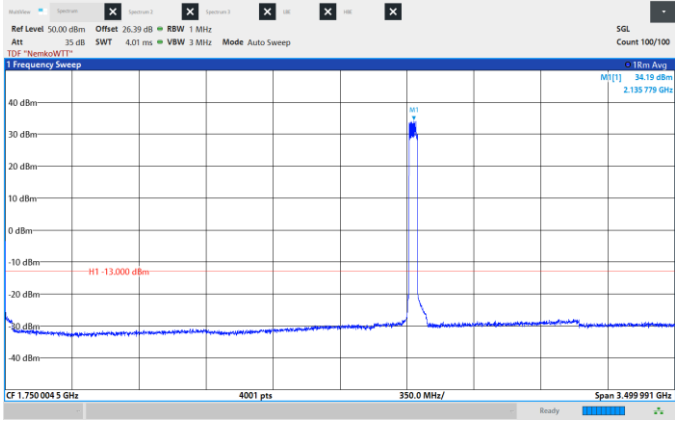
Figure 8.6-449: Conducted Spurious Emissions, Low CH 2132.5 MHz, 45 MHz, 16QAM, Frequency range: 0.009 - 3500 MHz.
