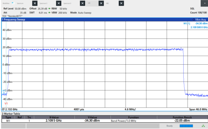
Figure 8.6-385: Conducted Spurious Emissions, Low CH 2130 MHz, 40 MHz, QPSK, Low band edge.
