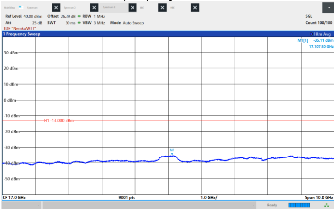
Figure 8.6-389: Conducted Spurious Emissions, Mid CH 2155 MHz, 40 MHz, QPSK, Frequency range: 12.0 – 22.0 GHz.
