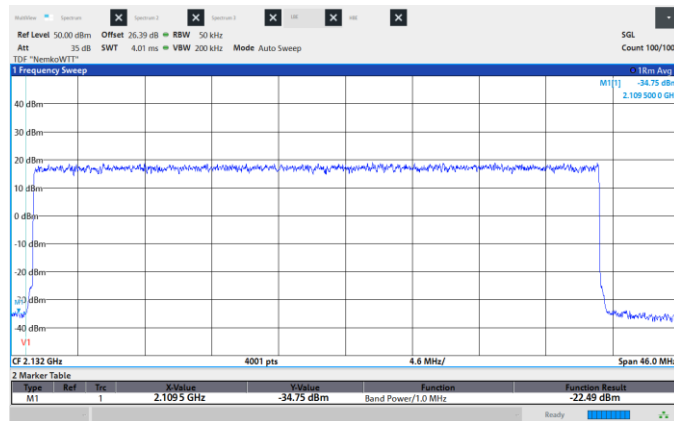
Figure 8.6-429: Conducted Spurious Emissions, Low CH 2130 MHz, 40 MHz, 1024QAM, Low band edge.
