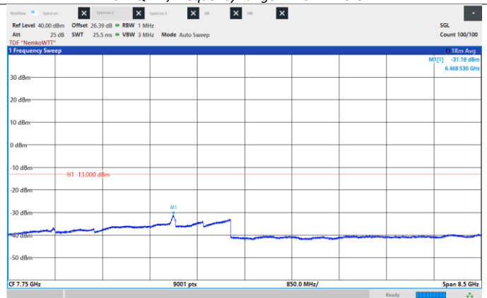
Figure 8.6-432: Conducted Spurious Emissions, Mid CH 2155 MHz, 40 MHz, 1024QAM, Frequency range: 3.5 – 12.0 GHz.
