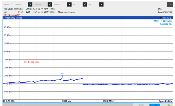
Figure 8.6-377: Conducted Spurious Emissions, Mid CH 2155 MHz, 35 MHz, 1024QAM, Frequency range: 3.5 – 12.0 GHz.
