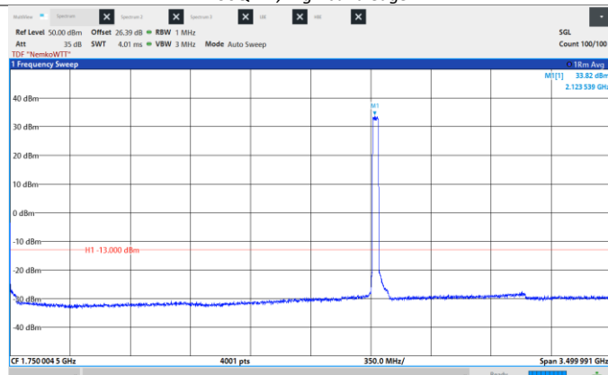
Figure 8.6-372: Conducted Spurious Emissions, Low CH 2127.5 MHz, 35 MHz, 1024QAM, Frequency range: 0.009 -3500 MHz.
