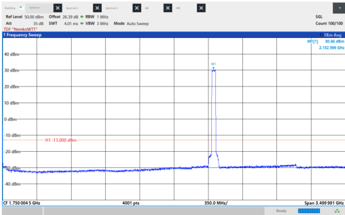
Figure 8.6-387: Conducted Spurious Emissions, Mid CH 2155 MHz, 40 MHz, QPSK, Frequency range: 0.009 -3500 MHz.
