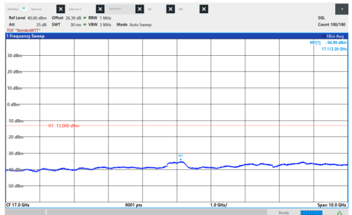
Figure 8.6-441: Conducted Spurious Emissions, Low CH 2132.5 MHz, 45 MHz, QPSK, Frequency range: 12.0 – 22.0 GHz.
