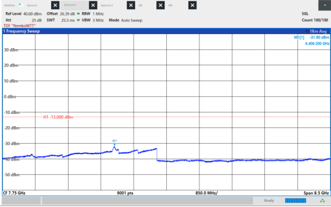
Figure 8.6-450: Conducted Spurious Emissions, Low CH 2132.5 MHz, 45 MHz, 16QAM, Frequency range: 3.5 - 12.0 GHz.
