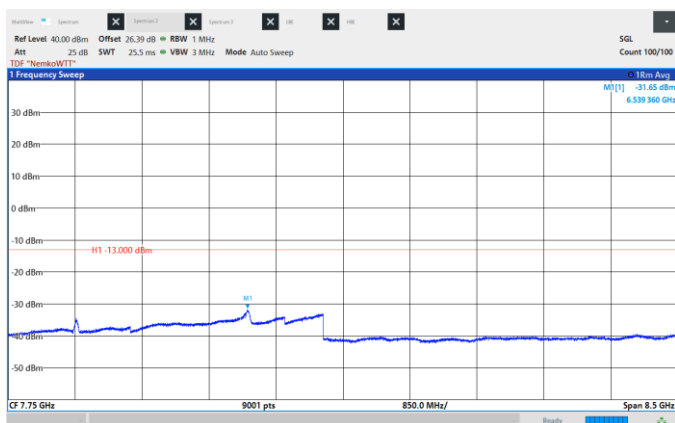
Figure 8.6-424: Conducted Spurious Emissions, High CH 2180 MHz, 40 MHz, 256QAM, Frequency range: 3.5 – 12.0 GHz
