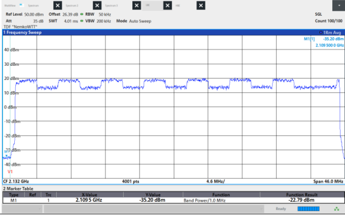
Figure 8.6-451: Conducted Spurious Emissions, Low CH 2132.5 MHz, 45 MHz, 16QAM, Low band edge.
