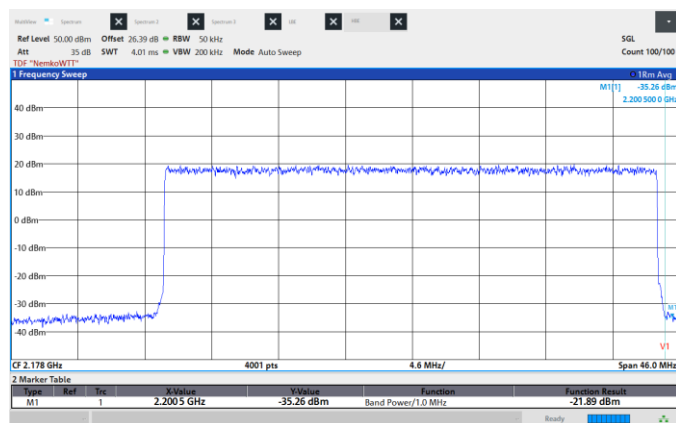
Figure 8.6-370: Conducted Spurious Emissions, High CH 2182.5 MHz, 35 MHz, 256QAM, High band edge.
