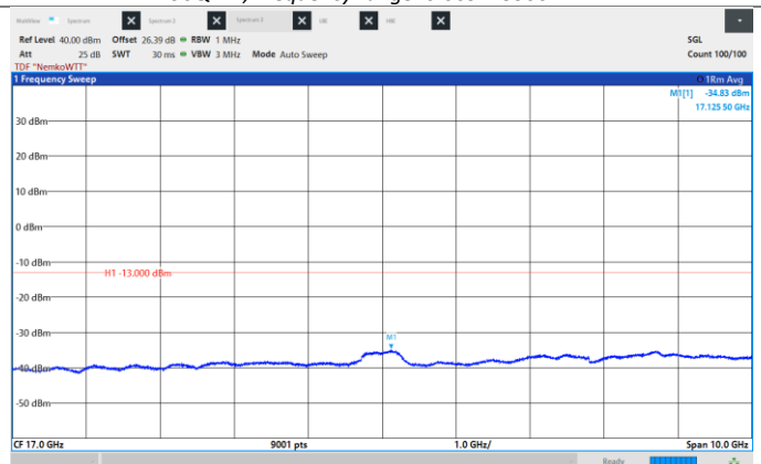
Figure 8.6-367: Conducted Spurious Emissions, Mid CH 2155 MHz, 35 MHz, 256QAM, Frequency range: 12.0 - 22.0 GHz.
