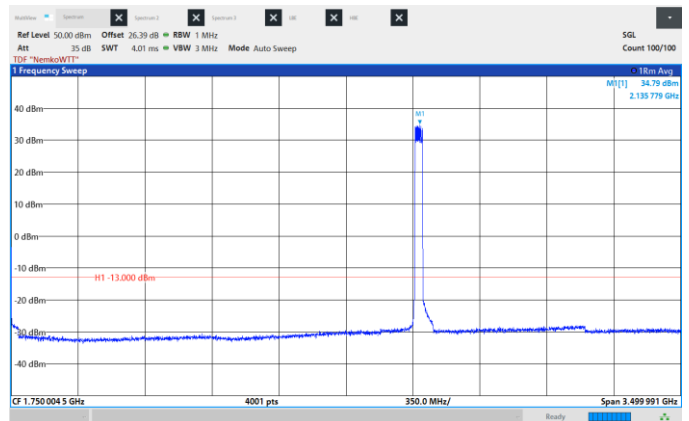
Figure 8.6-394: Conducted Spurious Emissions, Low CH 2130 MHz, 40 MHz, 16QAM, Frequency range: 0.009 - 3500 MHz.
