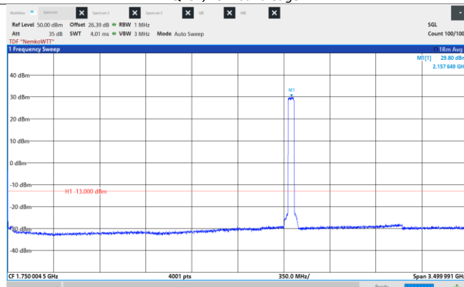
Figure 8.6-442: Conducted Spurious Emissions, Mid CH 2155 MHz, 45 MHz, QPSK, Frequency range: 0.009 - 3500 MHz.
