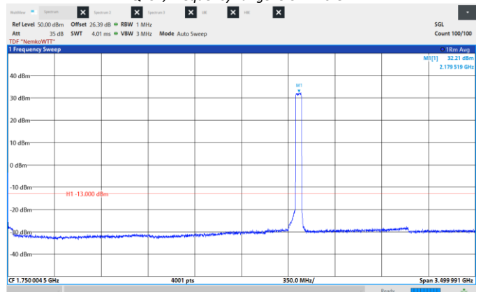
Figure 8.6-445: Conducted Spurious Emissions, High CH 2177.5 MHz, 45 MHz, QPSK, Frequency range: 0.009 – 3500 MHz.
