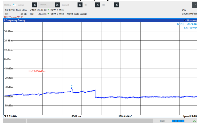
Figure 8.6-421: Conducted Spurious Emissions, Mid CH 2155 MHz, 40 MHz, 256QAM, Frequency range: 3.5 – 12.0 GHz.
