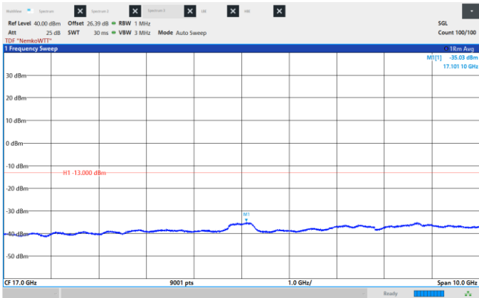
Figure 8.6-382: Conducted Spurious Emissions High CH 2182.5 MHz, 35 MHz, 1024QAM, Frequency range: 12.0 -22.0 GHz.
