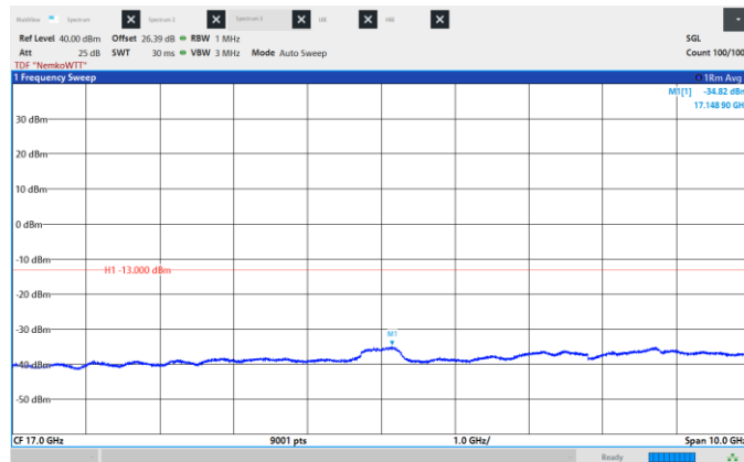
Figure 8.6-411: Conducted Spurious Emissions, Mid CH 2155 MHz, 40 MHz, 64QAM, Frequency range: 12.0 – 22.0 GHz.
