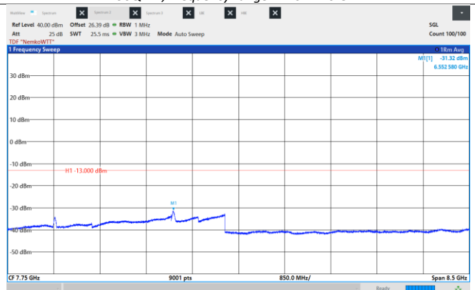
Figure 8.6-369: Conducted Spurious Emissions, High CH 2182.5 MHz, 35 MHz, 256QAM, Frequency range: 3.5 – 12.0 GHz
