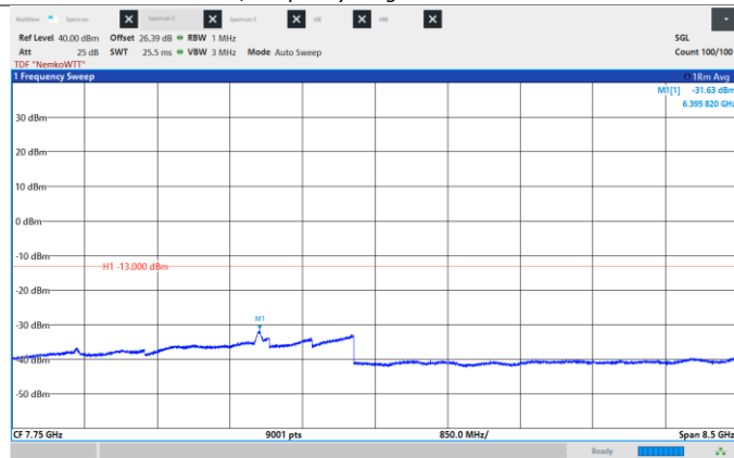
Figure 8.6-395: Conducted Spurious Emissions, Low CH 2130 MHz, 40 MHz, 16QAM, Frequency range: 3.5 - 12.0 GHz.
