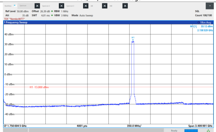
Figure 8.6-420: Conducted Spurious Emissions, Mid CH 2155 MHz, 40 MHz, 256QAM, Frequency range: 0.009 – 3500 MHz.
