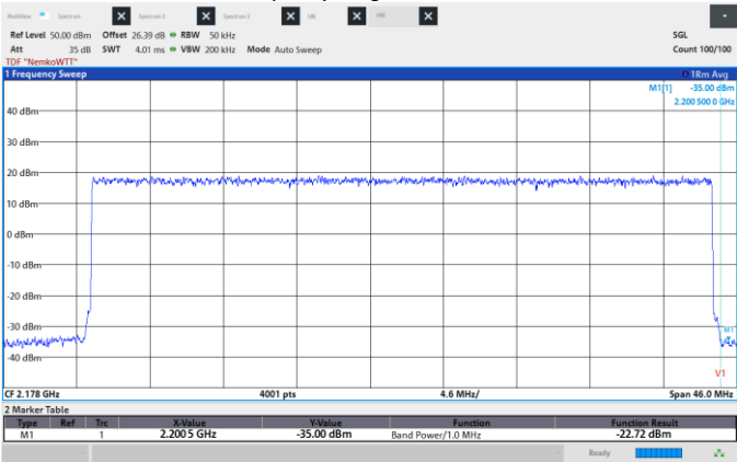
Figure 8.6-392: Conducted Spurious Emissions, High CH 2180 MHz, 40 MHz, QPSK, High band edge.
