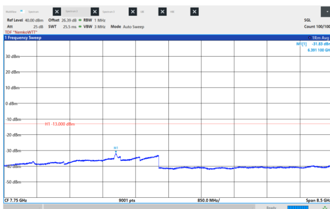
Figure 8.6-406: Conducted Spurious Emissions, Low CH 2130 MHz, 40 MHz, 64QAM, Frequency range: 3.5 - 12.0 GHz.
