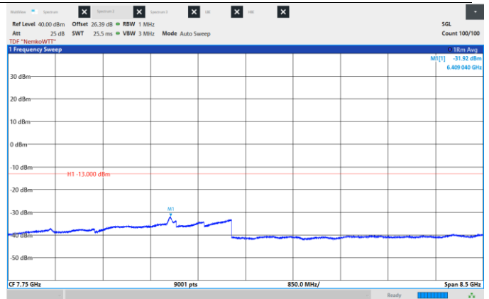
Figure 8.6-439: Conducted Spurious Emissions, Low CH 2132.5 MHz, 45 MHz, QPSK, Frequency range: 3.5 -12.0 GHz.
