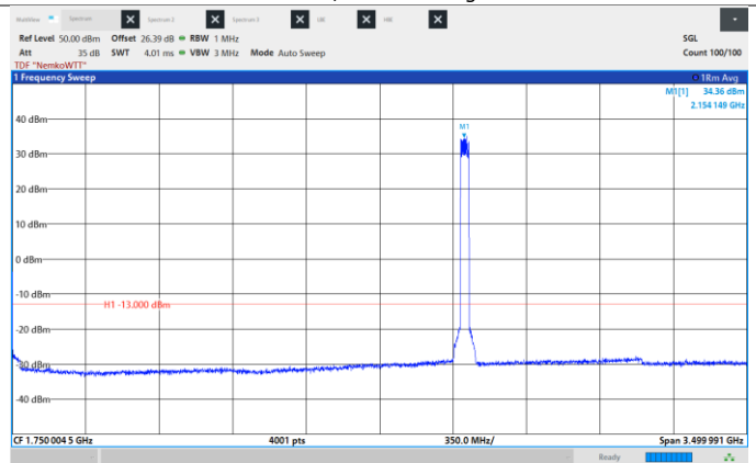
Figure 8.6-398: Conducted Spurious Emissions, Mid CH 2155 MHz, 40 MHz, 16QAM, Frequency range: 0.009 -3500 MHz
