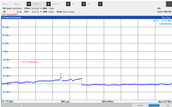
Figure 8.6-399: Conducted Spurious Emissions, Mid CH 2155 MHz, 40 MHz, 16QAM, Frequency range: 3.5 -12.0 GHz.
