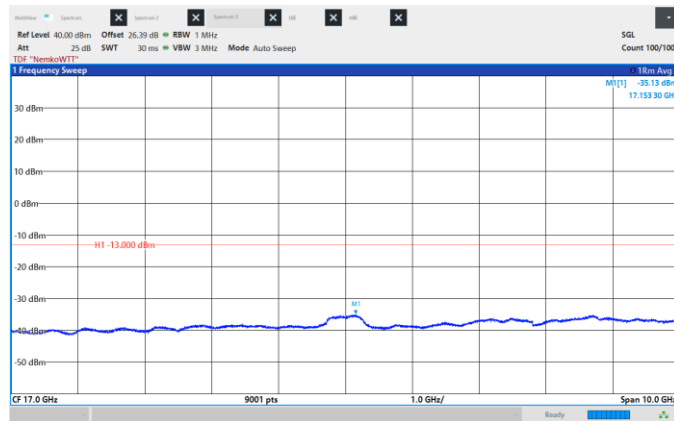
Figure 8.6-364: Conducted Spurious Emissions, Low CH 2127.5 MHz, 35 MHz, 256QAM, Frequency range: 12.0 – 22.0 GHz.
