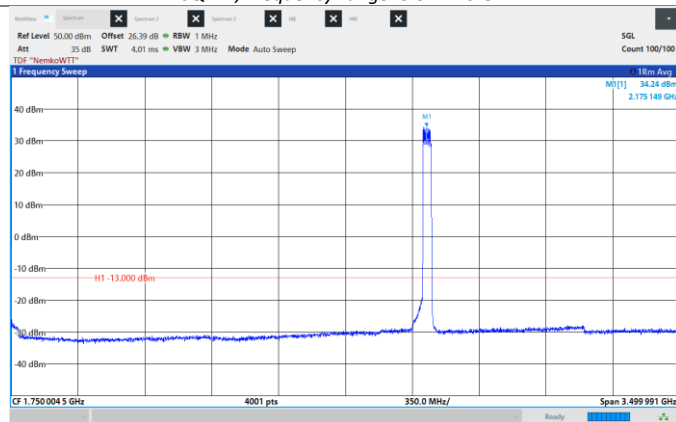
Figure 8.6-456: Conducted Spurious Emissions, High CH 2177.5 MHz, 45 MHz, 16QAM, Frequency range: 0.009 -3500 MHz.
