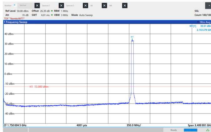
Figure 8.6-376: Conducted Spurious Emissions, Mid CH 2155 MHz, 35 MHz, 1024QAM, Frequency range: 0.009 – 3500 MHz.
