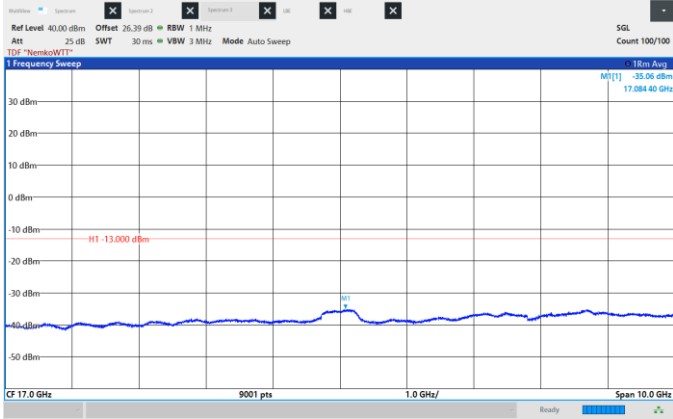
Figure 8.6-386: Conducted Spurious Emissions, Low CH 2130 MHz, 40 MHz, QPSK, Frequency range: 12.0 – 22.0 GHz.
