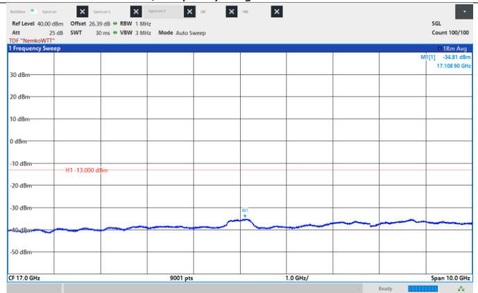
Figure 8.6-422: Conducted Spurious Emissions, Mid CH 2155 MHz, 40 MHz, 256QAM, Frequency range: 12.0 - 22.0 GHz.
