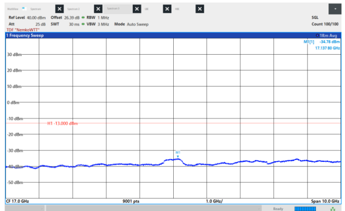
Figure 8.6-459: Conducted Spurious Emissions, High CH 2177.5 MHz, 45 MHz, 16QAM, Frequency range: 12.0 -22.0 GHz.
