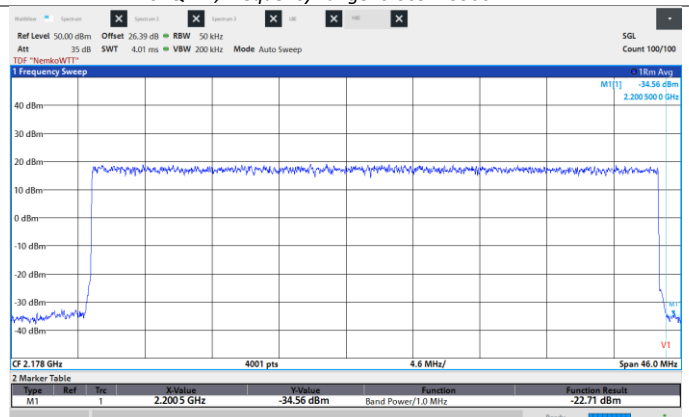
Figure 8.6-414: Conducted Spurious Emissions, High CH 2180 MHz, 40 MHz, 64QAM, High band edge.
