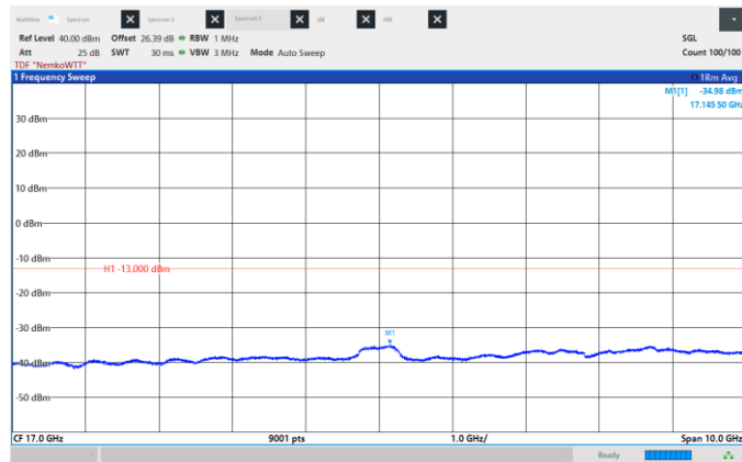
Figure 8.6-393: Conducted Spurious Emissions, High CH 2180 MHz, 40 MHz, QPSK, Frequency range: 12.0 -22.0 GHz
