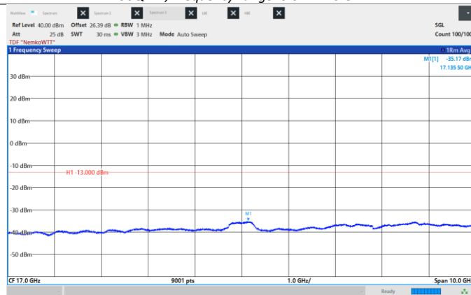
Figure 8.6-419: Conducted Spurious Emissions, Low CH 2130 MHz, 40 MHz, 256QAM, Frequency range: 12.0 – 22.0 GHz.
