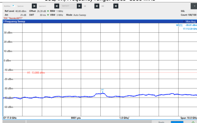
Figure 8.6-455: Conducted Spurious Emissions, Mid CH 2155 MHz, 45 MHz, 16QAM, Frequency range: 12.0 - 22.0 GHz.
