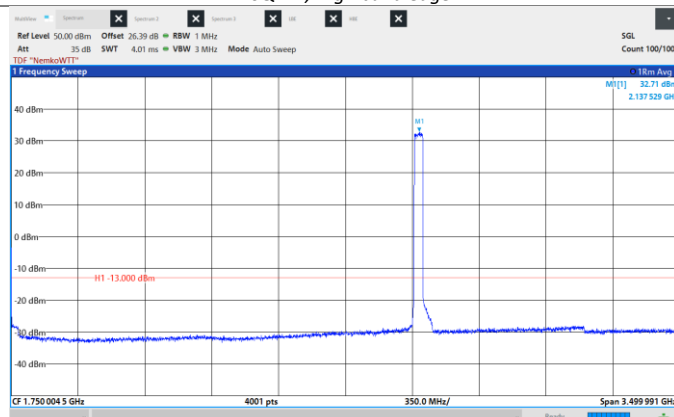
Figure 8.6-460: Conducted Spurious Emissions, Low CH 2132.5 MHz, 45 MHz, 64QAM, Frequency range: 0.009 -3500 MHz.
