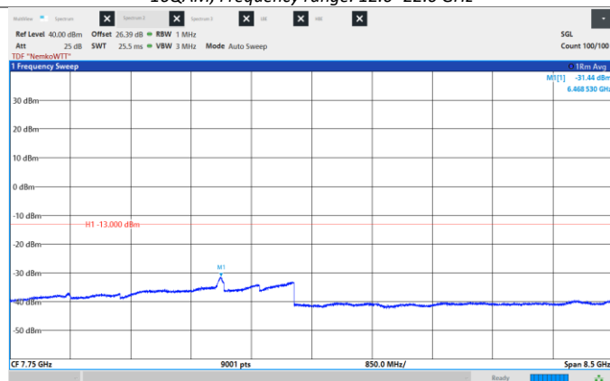
Figure 8.6-454: Conducted Spurious Emissions, Mid CH 2155 MHz, 45 MHz, 16QAM, Frequency range: 3.5 -12.0 GHz.
