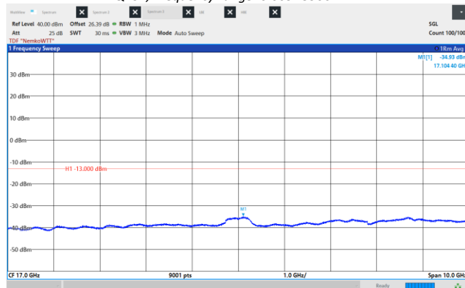
Figure 8.6-444: Conducted Spurious Emissions, Mid CH 2155 MHz, 45 MHz, QPSK, Frequency range: 12.0 – 22.0 GHz.
