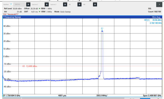
Figure 8.6-379: Conducted Spurious Emissions, High CH 2182.5 MHz, 35 MHz, 1024QAM, Frequency range: 0.009 -3500 MHz.
