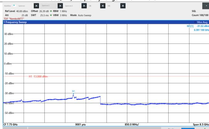
Figure 8.6-373: Conducted Spurious Emissions, Low CH 2127.5 MHz, 35 MHz, 1024QAM, Frequency range: 3.5 -12.0 GHz.
