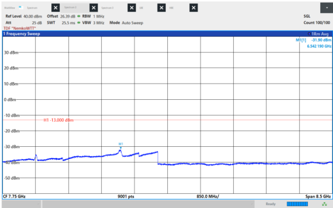
Figure 8.6-446: Conducted Spurious Emissions, High CH 2177.5 MHz, 45 MHz, QPSK, Frequency range: 3.5 -12.0 GHz.
