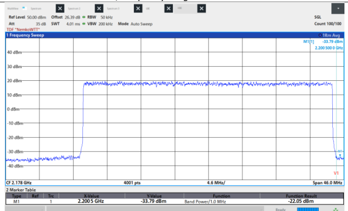
Figure 8.6-381: Conducted Spurious Emissions, High CH 2182.5 MHz, 35 MHz, 1024QAM, High band edge.
