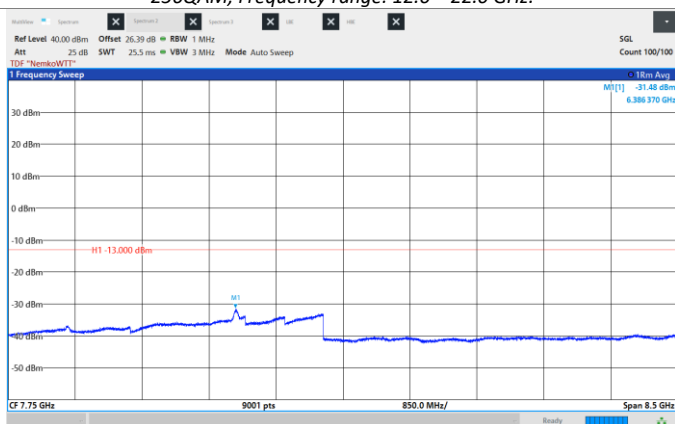
Figure 8.6-428: Conducted Spurious Emissions, Low CH 2130 MHz, 40 MHz, 1024QAM, Frequency range: 3.5 -12.0 GHz.
