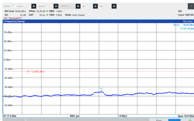
Figure 8.6-371: Conducted Spurious Emissions, High CH 2182.5 MHz, 35 MHz, 256QAM, Frequency range: 12.0 – 22.0 GHz.
