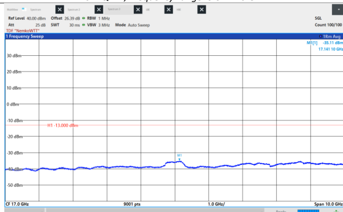
Figure 8.6-375: Conducted Spurious Emissions, Low CH 2127.5 MHz, 35 MHz, 1024QAM, Frequency range: 12.0 – 22.0 GHz.
