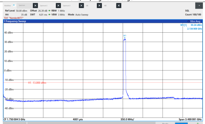
Figure 8.6-416: Conducted Spurious Emissions, Low CH 2130 MHz, 40 MHz, 256QAM, Frequency range: 0.009 - 3500 MHz.
