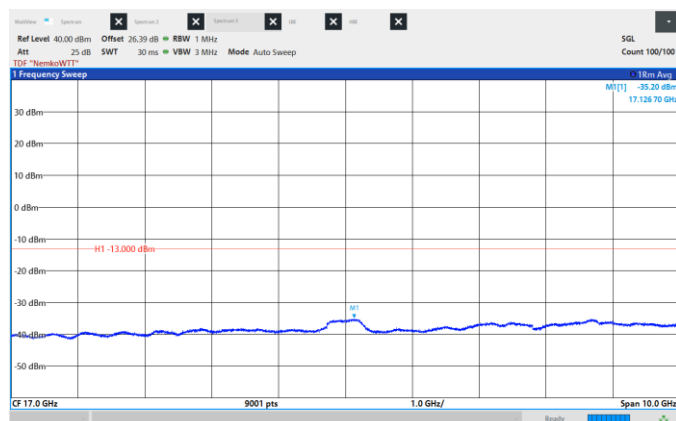
Figure 8.6-452: Conducted Spurious Emissions, Low CH 2132.5 MHz, 45 MHz, 16QAM, Frequency range: 12.0 -22.0 GHz
