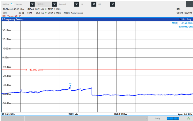
Figure 8.6-391: Conducted Spurious Emissions, High CH 2180 MHz, 40 MHz, QPSK, Frequency range: 3.5 -12.0 GHz.
