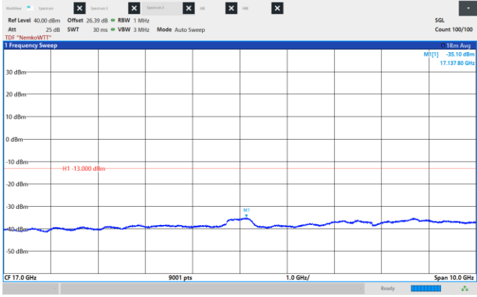
Figure 8.6-448: Conducted Spurious Emissions, High CH 2177.5 MHz, 45 MHz, QPSK, Frequency range: 12.0 -22.0 GHz
