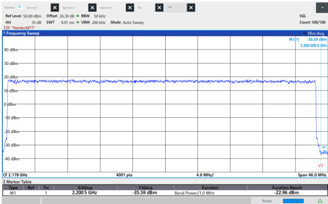
Figure 8.6-447: Conducted Spurious Emissions, High CH 2177.5 MHz, 45 MHz, QPSK, High band edge.
