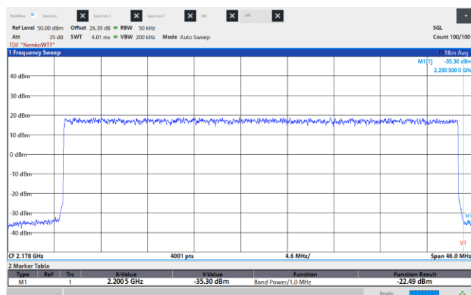
Figure 8.6-425: Conducted Spurious Emissions, High CH 2180 MHz, 40 MHz, 256QAM, High band edge.
