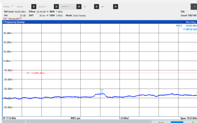
Figure 8.6-426: Conducted Spurious Emissions, High CH 2180 MHz, 40 MHz, 256QAM, Frequency range: 12.0 – 22.0 GHz.
