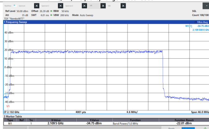
Figure 8.6-374: Conducted Spurious Emissions, Low CH 2127.5 MHz, 35 MHz, 1024QAM, Low band edge.
