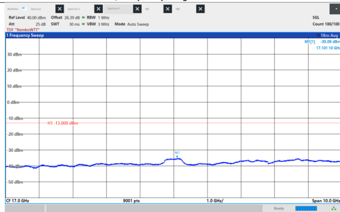
Figure 8.6-397: Conducted Spurious Emissions, Low CH 2130 MHz, 40 MHz, 16QAM, Frequency range: 12.0 -22.0 GHz
