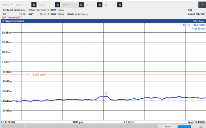
Figure 8.6-400: Conducted Spurious Emissions, Mid CH 2155 MHz, 40 MHz, 16QAM, Frequency range: 12.0 – 22.0 GHz.
