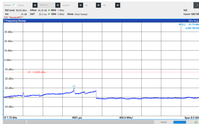
Figure 8.6-435: Conducted Spurious Emissions, High CH 2180 MHz, 40 MHz, 1024QAM, Frequency range: 3.5 -12.0 GHz.
