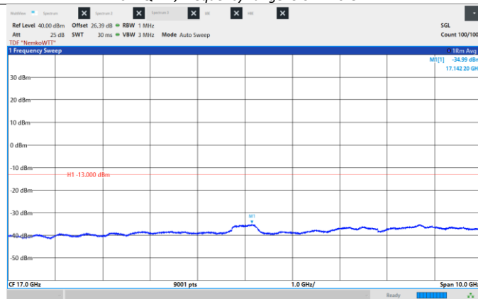
Figure 8.6-437: Conducted Spurious Emissions High CH 2180 MHz, 40 MHz, 1024QAM, Frequency range: 12.0 -22.0 GHz.
