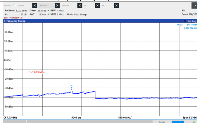
Figure 8.6-366: Conducted Spurious Emissions, Mid CH 2155 MHz, 35 MHz, 256QAM, Frequency range: 3.5 – 12.0 GHz.
