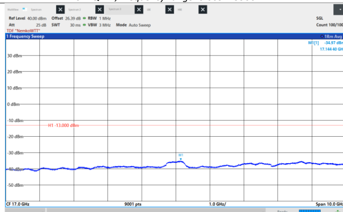
Figure 8.6-378: Conducted Spurious Emissions, Mid CH 2155 MHz, 35 MHz, 1024QAM, Frequency range: 12.0 -22.0 GHz.
