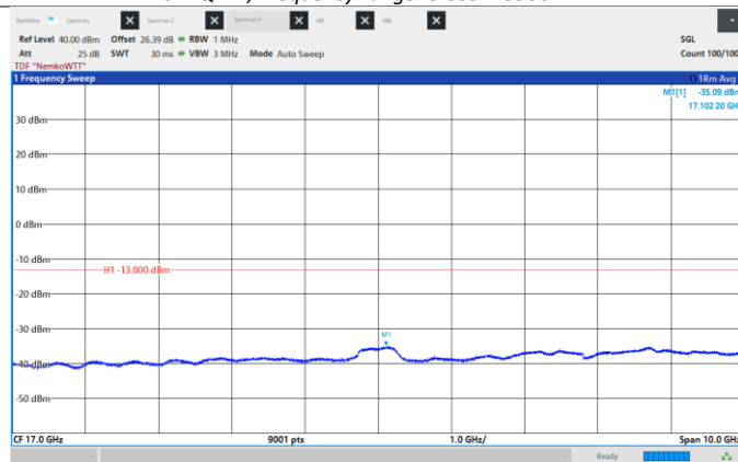
Figure 8.6-433: Conducted Spurious Emissions, Mid CH 2155 MHz, 40 MHz, 1024QAM, Frequency range: 12.0 -22.0 GHz.
