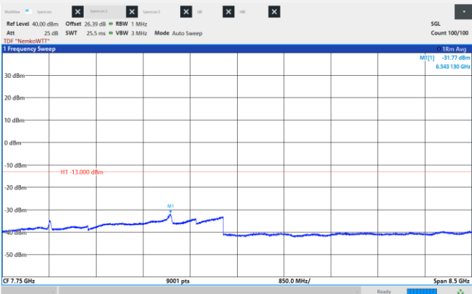
Figure 8.6-402: Conducted Spurious Emissions, High CH 2180 MHz, 40 MHz, 16QAM, Frequency range: 3.5 – 12.0 GHz
