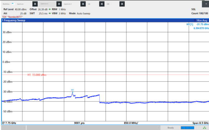
Figure 8.6-384: Conducted Spurious Emissions, Low CH 2130 MHz, 40 MHz, QPSK, Frequency range: 3.5 -12.0 GHz.
