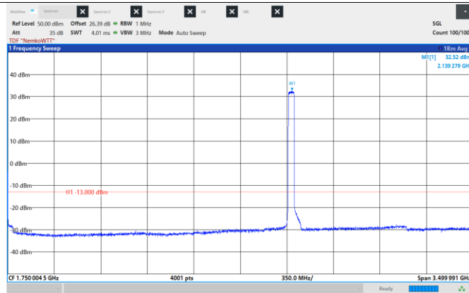
Figure 8.6-438: Conducted Spurious Emissions, Low CH 2132.5 MHz, 45 MHz, QPSK, Frequency range: 0.009 – 3500 MHz.
