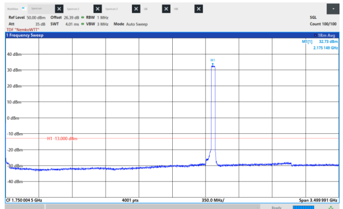
Figure 8.6-412: Conducted Spurious Emissions, High CH 2180 MHz, 40 MHz, 64QAM, Frequency range: 0.009 – 3500 MHz.
