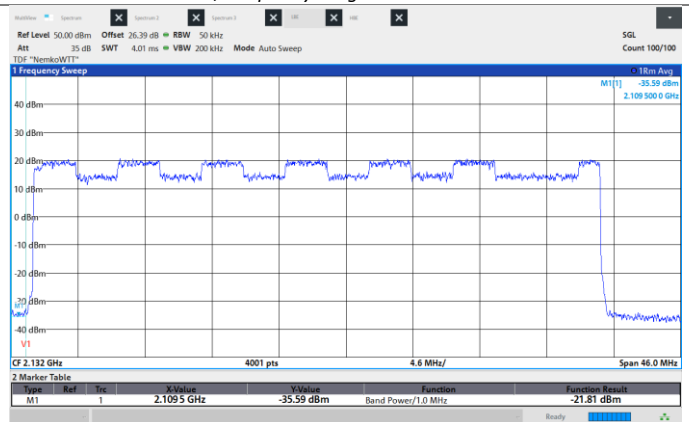
Figure 8.6-396: Conducted Spurious Emissions, Low CH 2130 MHz, 40 MHz, 16QAM, Low band edge.
