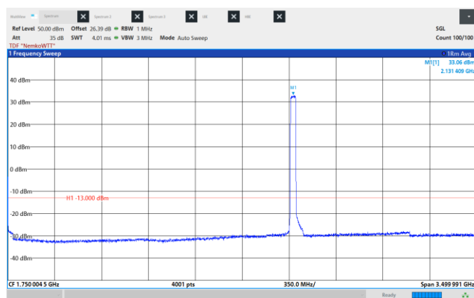
Figure 8.6-405: Conducted Spurious Emissions, Low CH 2130 MHz, 40 MHz, 64QAM, Frequency range: 0.009 -3500 MHz.
