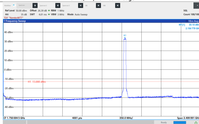
Figure 8.6-431: Conducted Spurious Emissions, Mid CH 2155 MHz, 40 MHz, 1024QAM, Frequency range: 0.009 – 3500 MHz.
