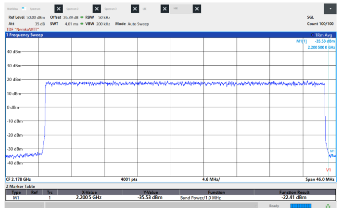
Figure 8.6-436: Conducted Spurious Emissions, High CH 2180 MHz, 40 MHz, 1024QAM, High band edge.
