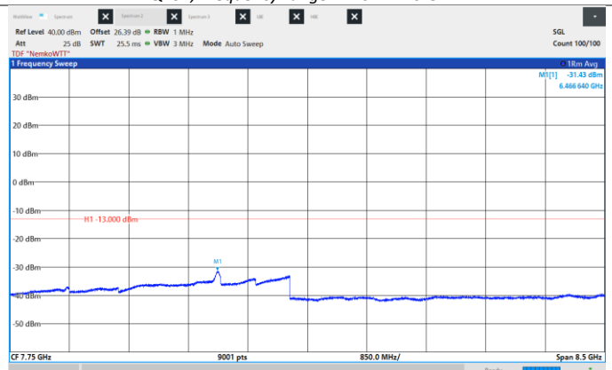
Figure 8.6-443: Conducted Spurious Emissions, Mid CH 2155 MHz, 45 MHz, QPSK, Frequency range: 3.5 - 12.0 GHz.
