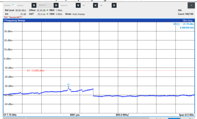
Figure 8.6-461: Conducted Spurious Emissions, Low CH 2132.5 MHz, 45 MHz, 64QAM, Frequency range: 3.5 - 12.0 GHz.
