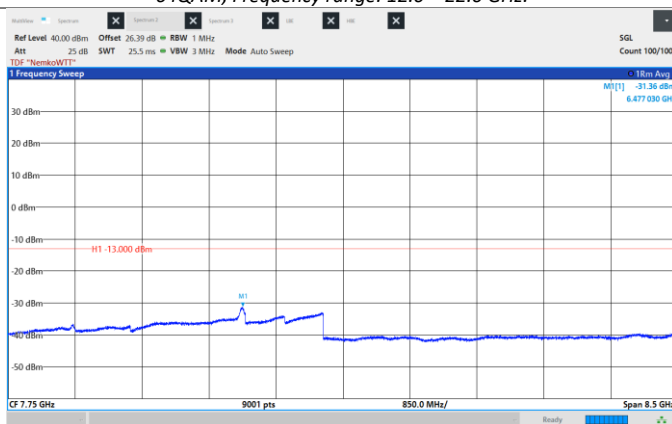
Figure 8.6-410: Conducted Spurious Emissions, Mid CH 2155 MHz, 40 MHz, 64QAM, Frequency range: 3.5 -12.0 GHz.
