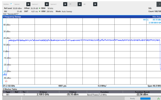
Figure 8.6-440: Conducted Spurious Emissions, Low CH 2132.5 MHz, 45 MHz, QPSK, Low band edge.
