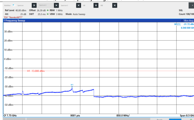
Figure 8.6-413: Conducted Spurious Emissions, High CH 2180 MHz, 40 MHz, 64QAM, Frequency range: 3.5 – 12.0 GHz.
