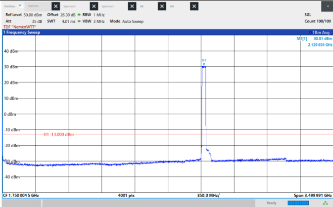
Figure 8.6-383: Conducted Spurious Emissions, Low CH 2130 MHz, 40 MHz, QPSK, Frequency range: 0.009 – 3500 MHz.
