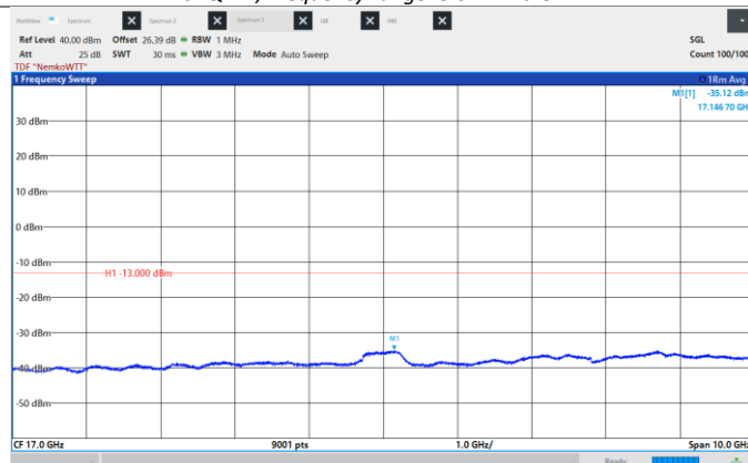
Figure 8.6-415: Conducted Spurious Emissions, High CH 2180 MHz, 40 MHz, 64QAM, Frequency range: 12.0 - 22.0 GHz
