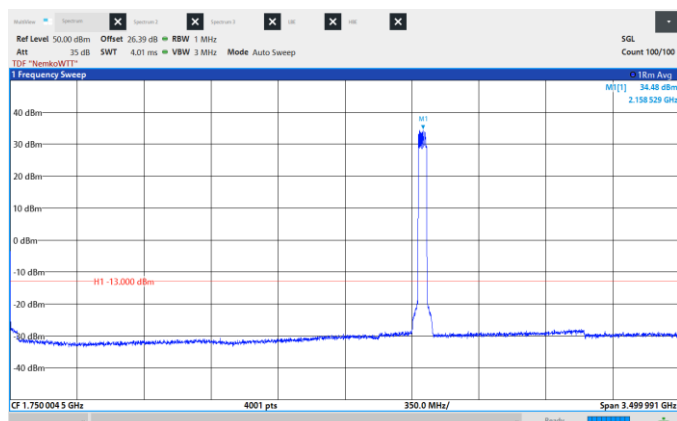
Figure 8.6-453: Conducted Spurious Emissions, Mid CH 2155 MHz, 45 MHz, 16QAM, Frequency range: 0.009 -3500 MHz
