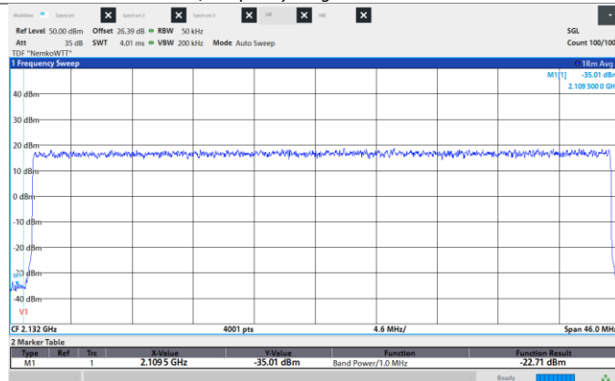
Figure 8.6-462: Conducted Spurious Emissions, Low CH 2132.5 MHz, 45 MHz, 64QAM, Low band edge
