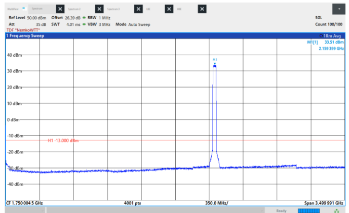
Figure 8.6-365: Conducted Spurious Emissions, Mid CH 2155 MHz, 35 MHz, 256QAM, Frequency range: 0.009 – 3500 MHz.
