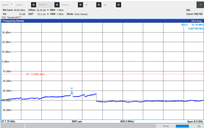
Figure 8.6-388: Conducted Spurious Emissions, Mid CH 2155 MHz, 40 MHz, QPSK, Frequency range: 3.5 -12.0 GHz.
