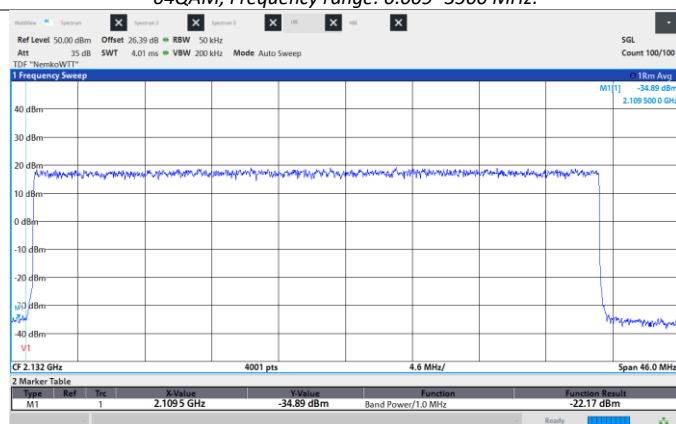
Figure 8.6-407: Conducted Spurious Emissions, Low CH 2130 MHz, 40 MHz, 64QAM, Low band edge
