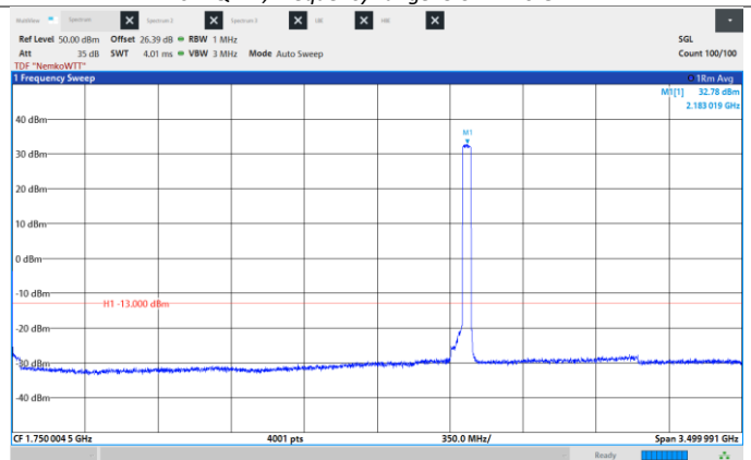
Figure 8.6-434: Conducted Spurious Emissions, High CH 2180 MHz, 40 MHz, 1024QAM, Frequency range: 0.009 -3500 MHz.
