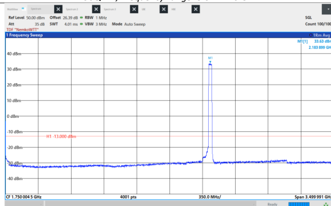
Figure 8.6-368: Conducted Spurious Emissions, High CH 2182.5 MHz, 35 MHz, 256QAM, Frequency range: 0.009 - 3500 MHz.
