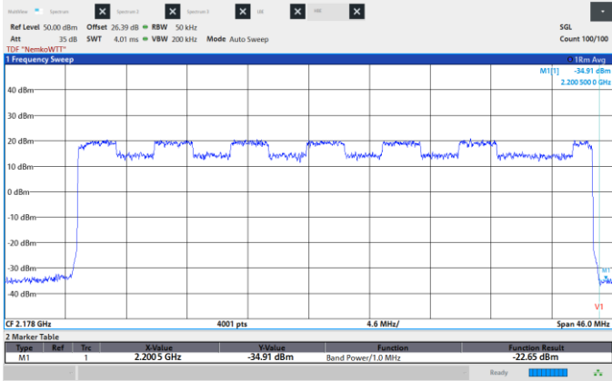
Figure 8.6-403: Conducted Spurious Emissions, High CH 2180 MHz, 40 MHz, 16QAM, High band edge
