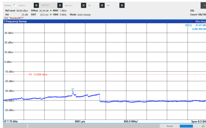
Figure 8.6-417: Conducted Spurious Emissions, Low CH 2130 MHz, 40 MHz, 256QAM, Frequency range: 3.5 – 12.0 GHz.
