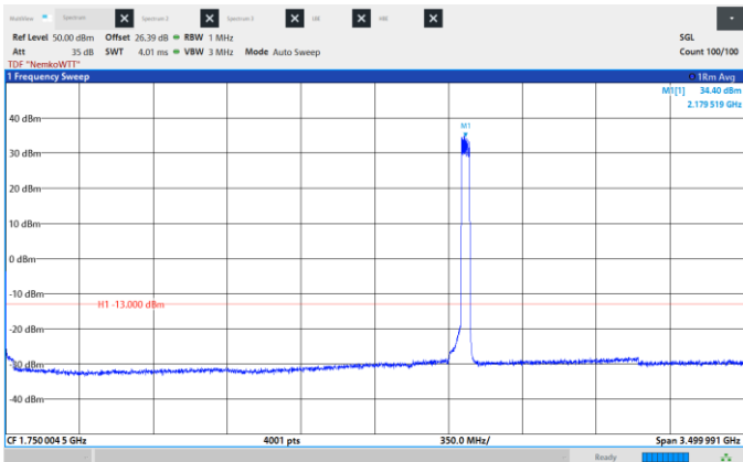
Figure 8.6-401: Conducted Spurious Emissions, High CH 2180 MHz, 40 MHz, 16QAM, Frequency range: 0.009 -3500 MHz.
