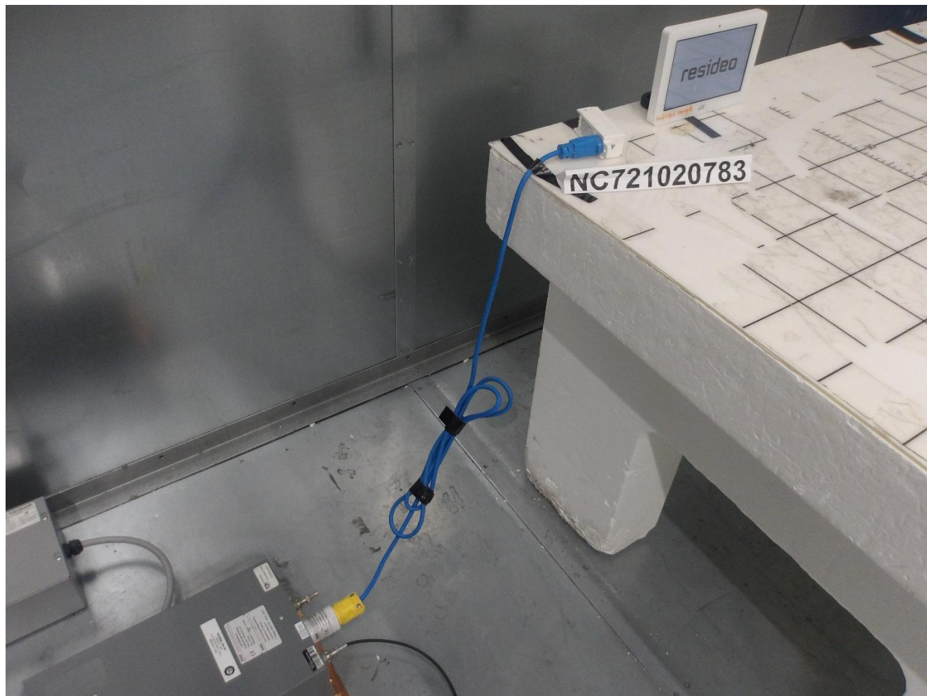
Photo 2-3 – Power Line Conducted Emissions – Side View
