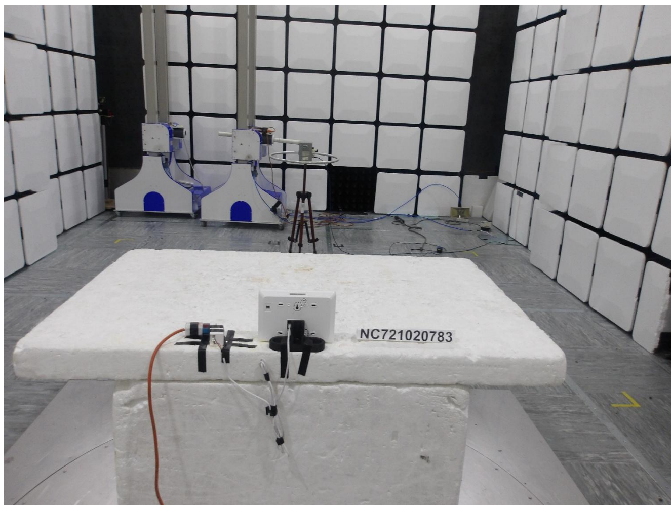
Photo 1-6 – Radiated Spurious Emissions 9 kHz-30 MHz – Rear View [Horizontal Co-Planar]
