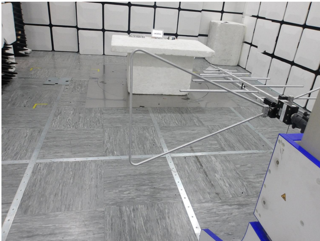
Photo 1-7 – Radiated Spurious Emissions 30MHz – 1GHz – Front View
