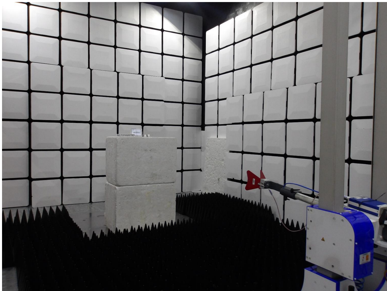
Photo 1-9 – Radiated Spurious Emissions 1GHz – 18GHz – Front View
