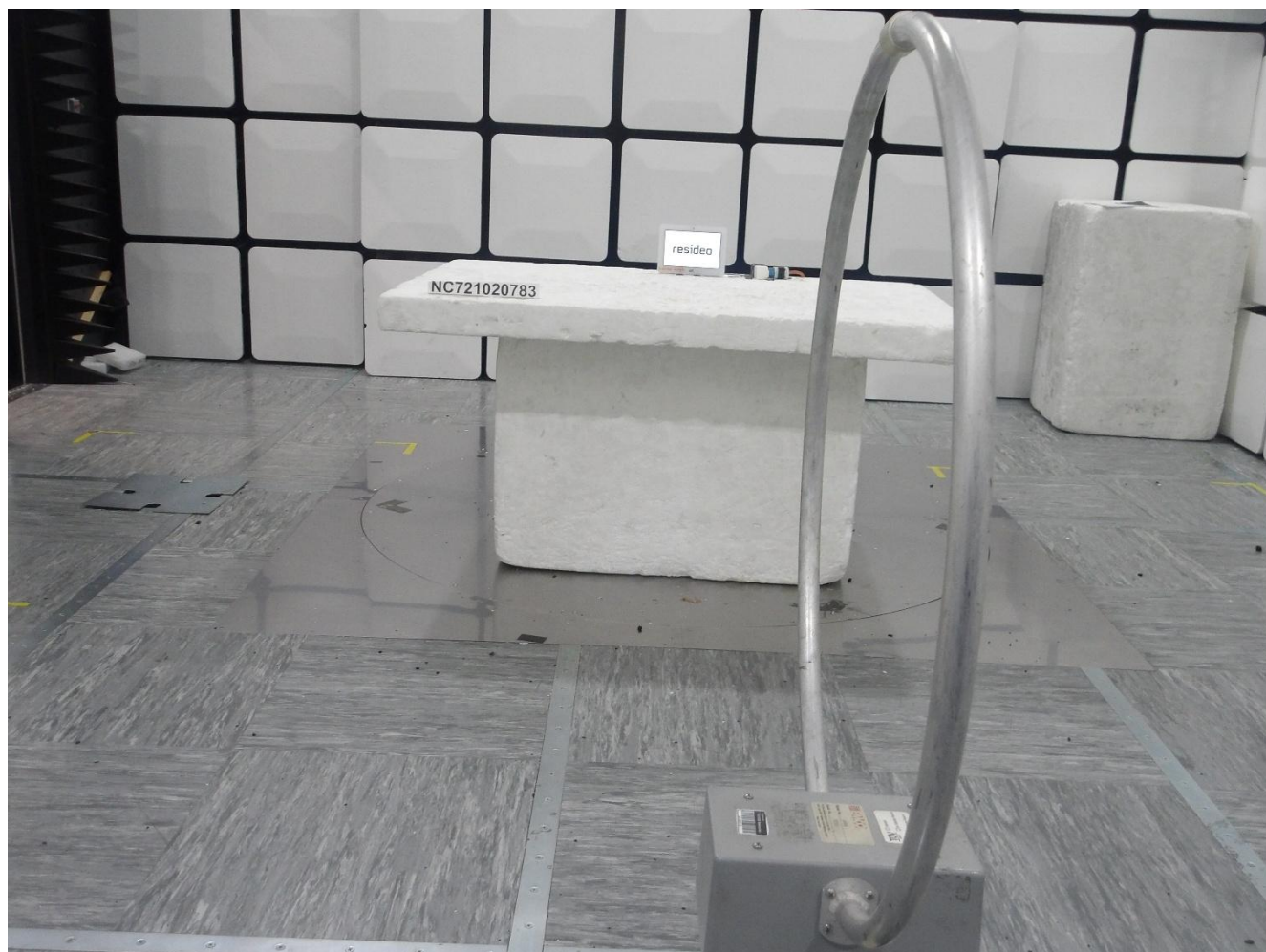
Photo 1-3 – Radiated Spurious Emissions 9 kHz-30 MHz – Front View [Vertical Co-Planar]
