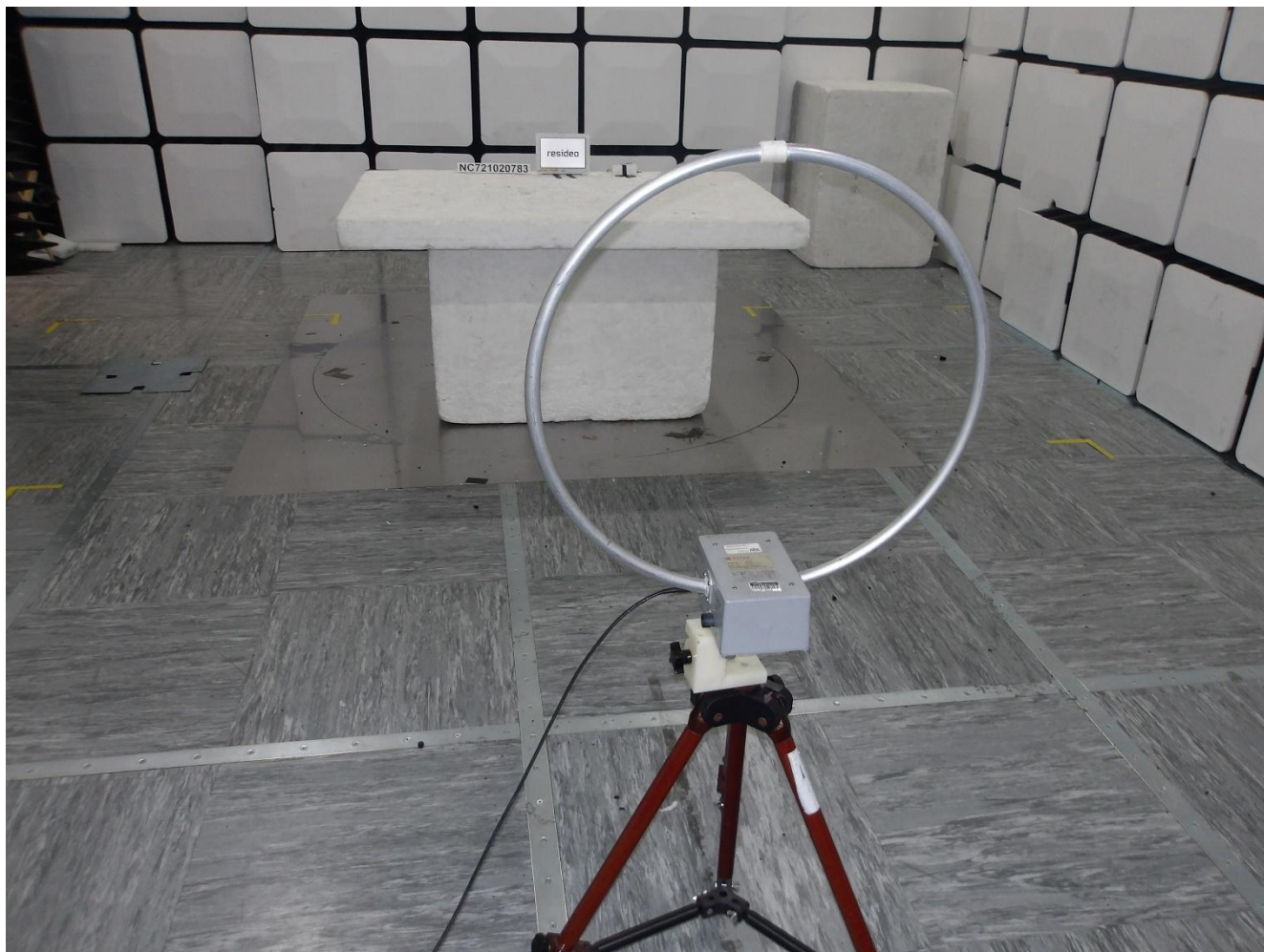
Photo 1-2 – Radiated Spurious Emissions 9 kHz-30 MHz – Rear View [Vertical Co-Axial]
