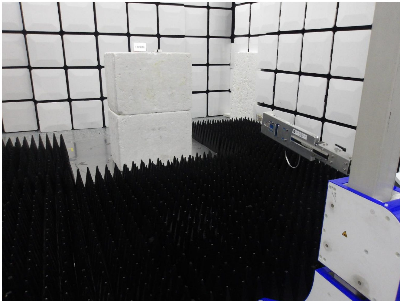
Photo 1-11 – Radiated Spurious Emissions 18GHz – 40GHz – Front View
