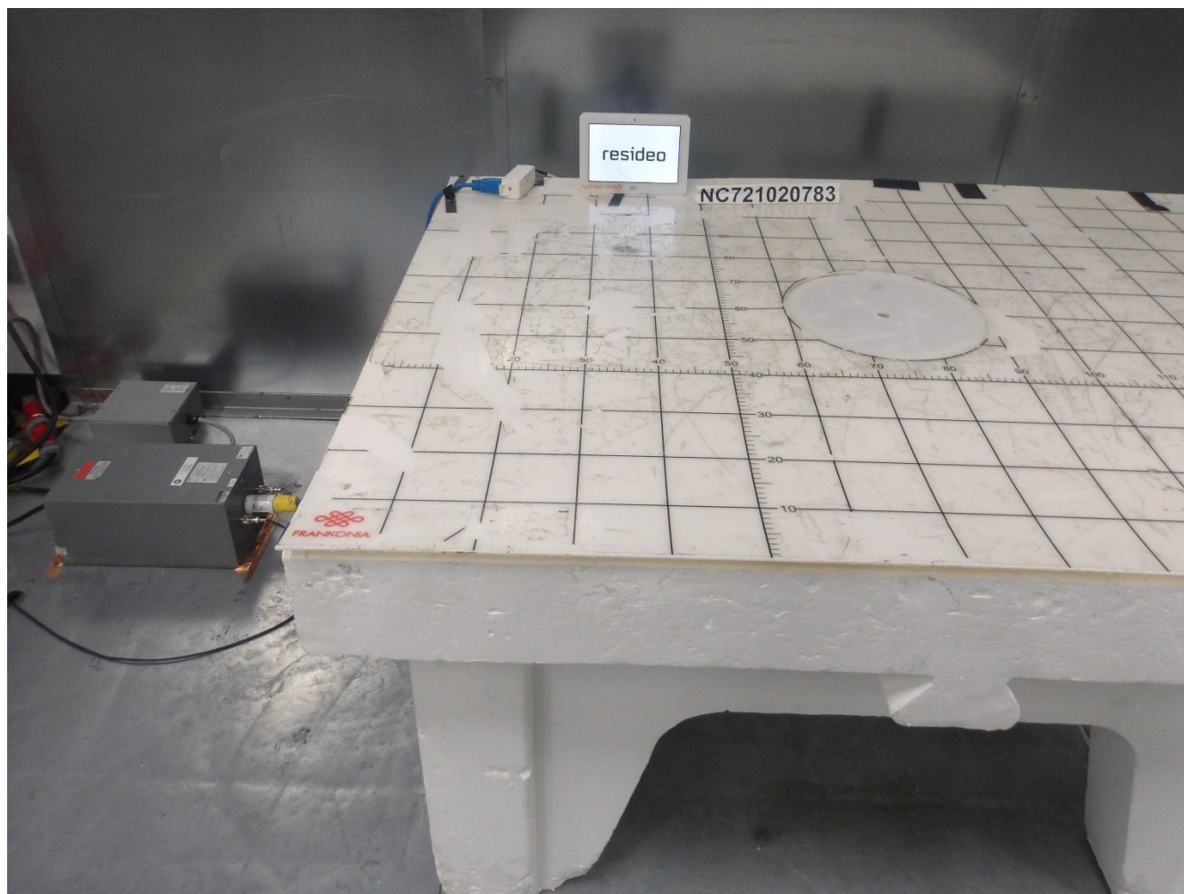
Photo 2-1 – Power Line Conducted Emissions – Front View
