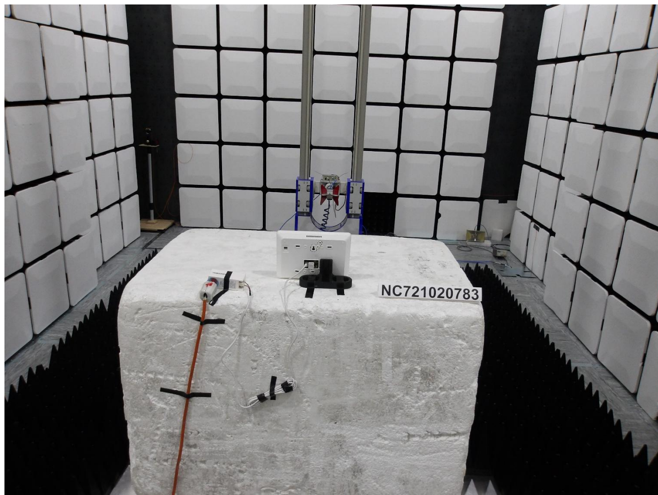
Photo 1-10 – Radiated Spurious Emissions 1GHz – 18GHz – Rear View
