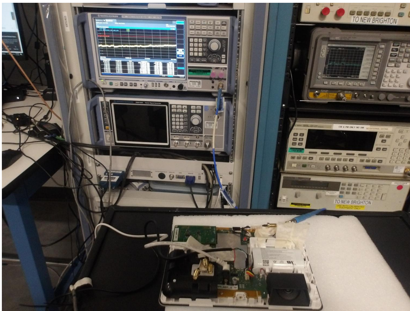
Photo 3-1 – RF Conducted Measurements
