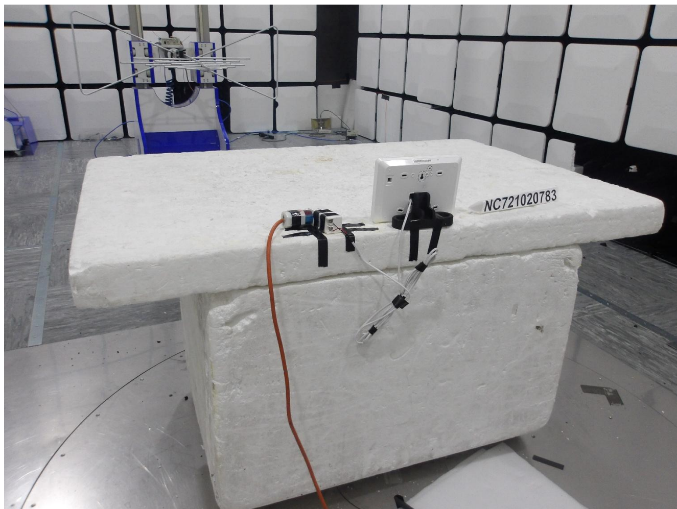
Photo 1-8 – Radiated Spurious Emissions 30MHz – 1GHz – Rear View
