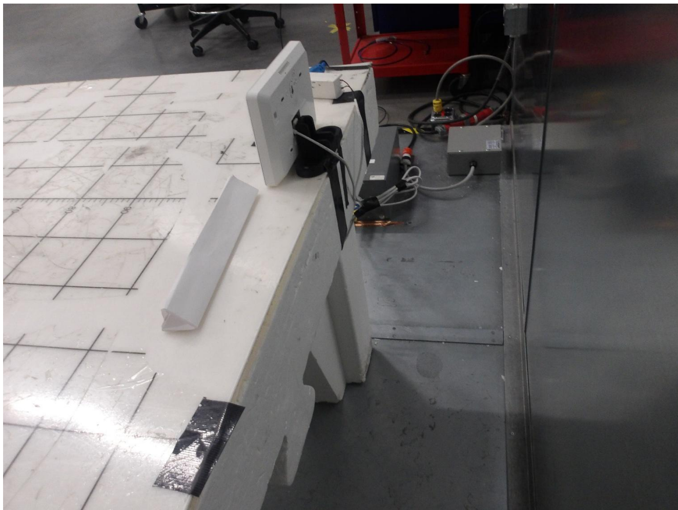
Photo 2-2 – Power Line Conducted Emissions – Side View
