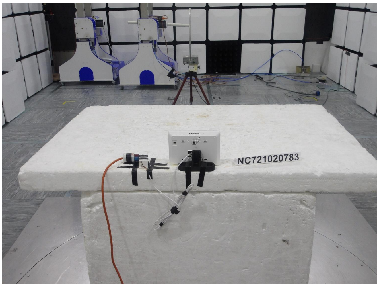
Photo 1-4 – Radiated Spurious Emissions 9 kHz-30 MHz – Rear View [Vertical Co-Planar]
