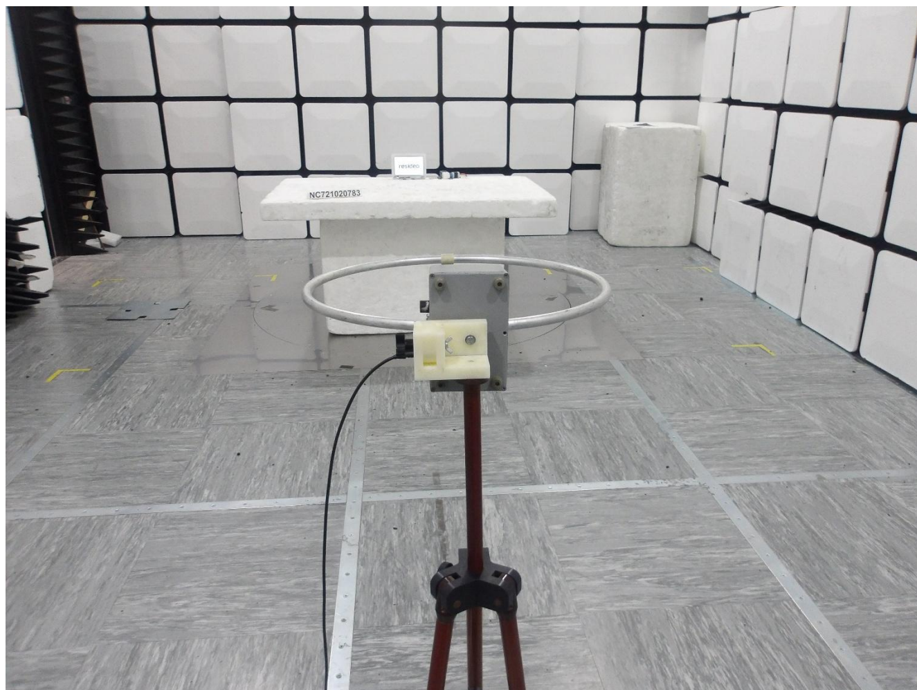
Photo 1-5 – Radiated Spurious Emissions 9 kHz-30 MHz – Front View [Horizontal Co-Planar]
