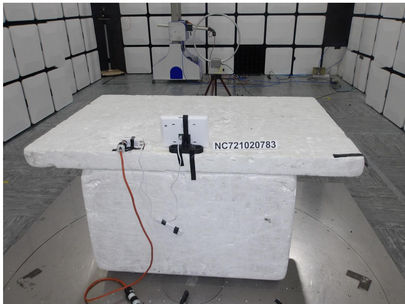
Photo 1-1 – Radiated Spurious Emissions 9 kHz-30 MHz – Front View [Vertical Co-Axial]
