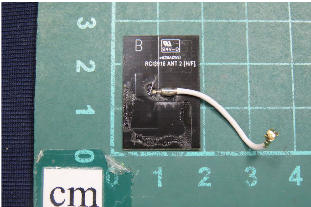
(25) EUT Photo
