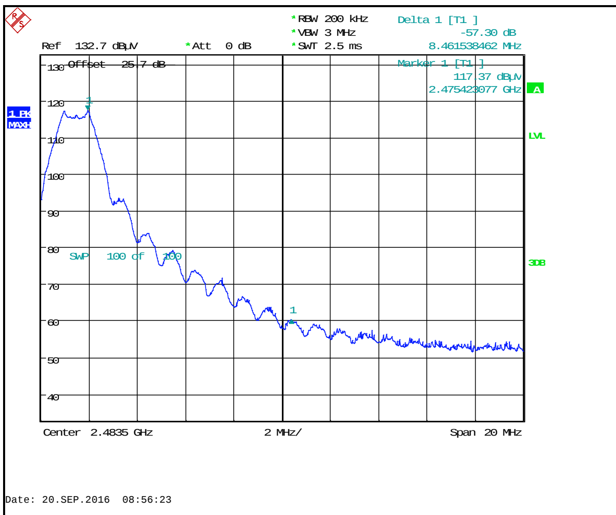
Plot 4-2: Upper Band Edge - Antenna #1
