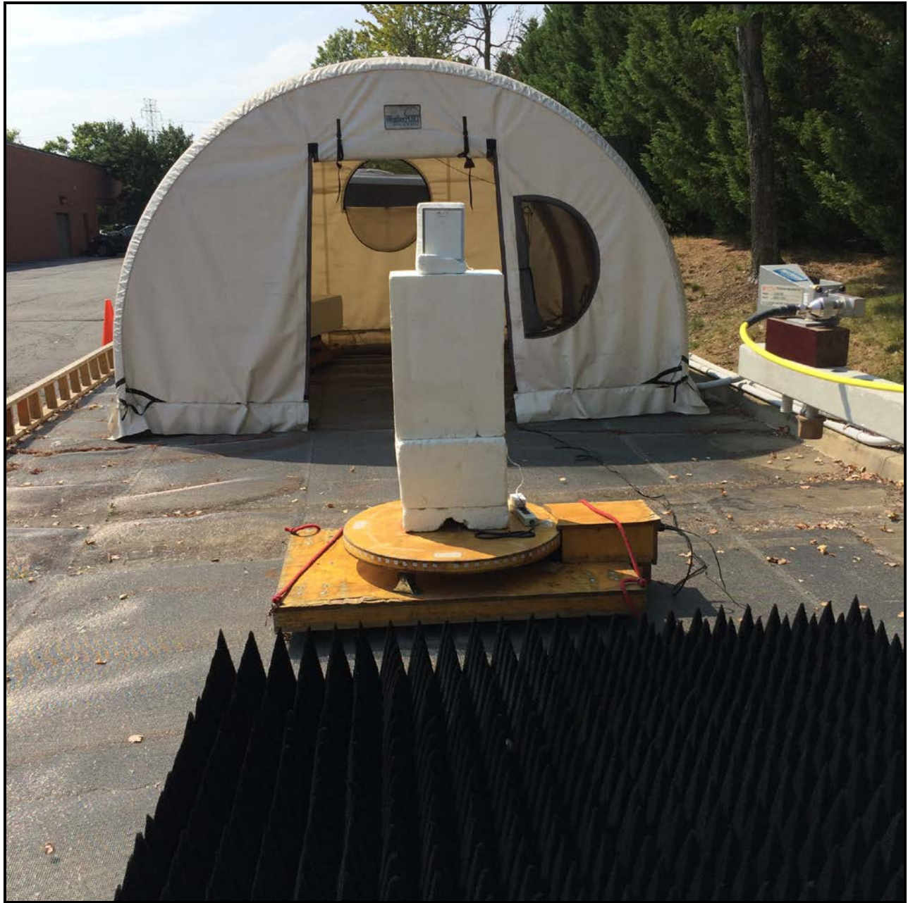
Photograph 1: Radiated Emissions Testing – Front View
