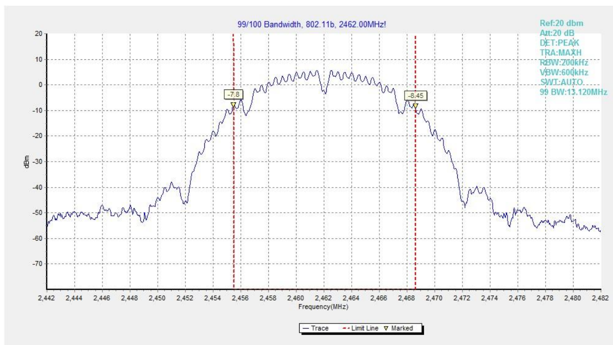
Fig.58 99% Occupied Bandwidth (802.11b, CH 11)
