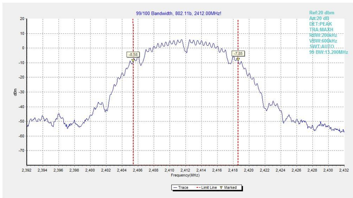
Fig.56 99% Occupied Bandwidth (802.11b, CH 1)
