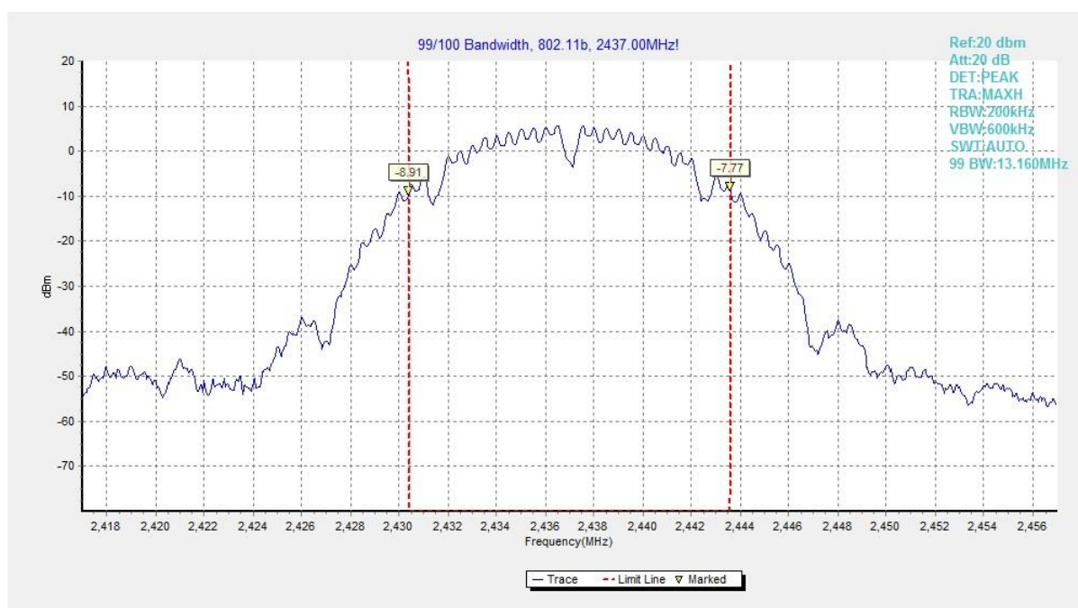
Fig.57 99% Occupied Bandwidth (802.11b, CH 6)
