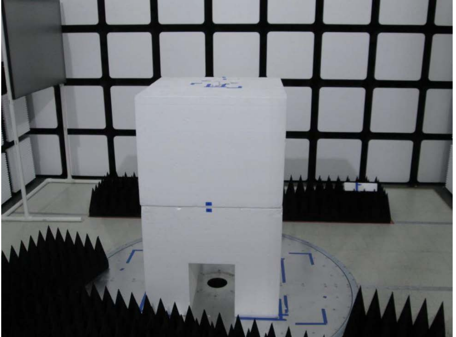
ANT1 Radiated RF Measurement Setup Above 1GHz - Front View
