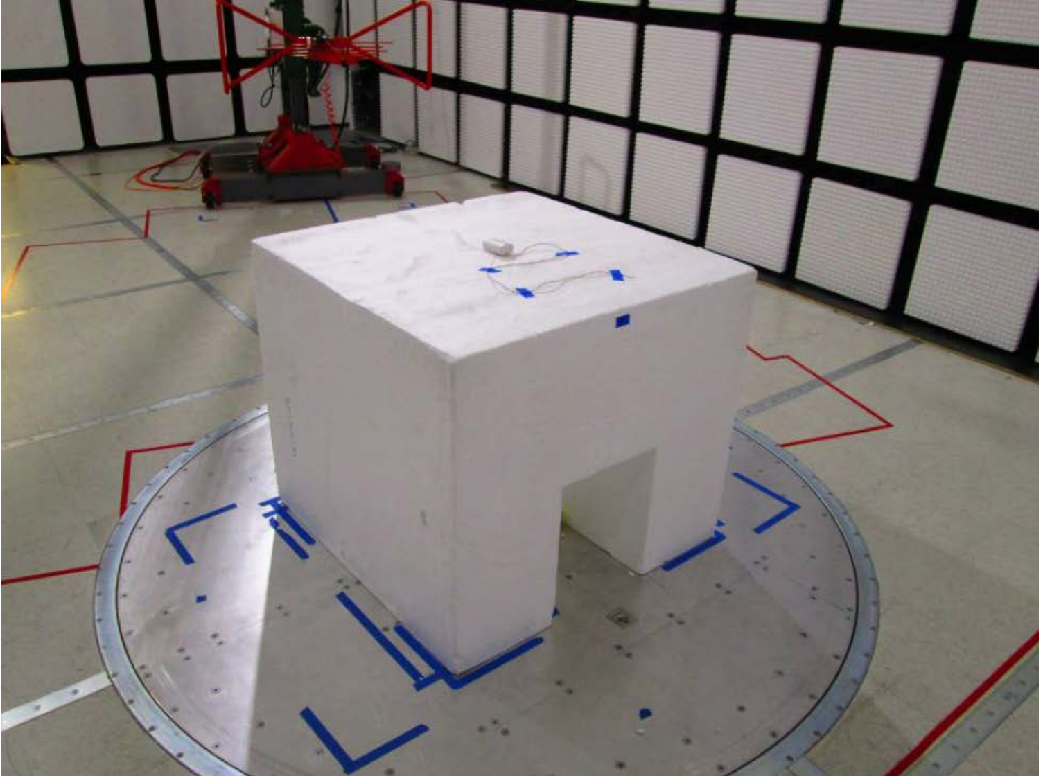
ANT1 Radiated Testing Below 1GHz - Back View
