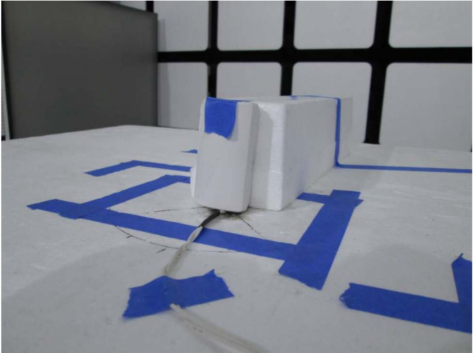
XYZ Orientation Setup - Z Axis
