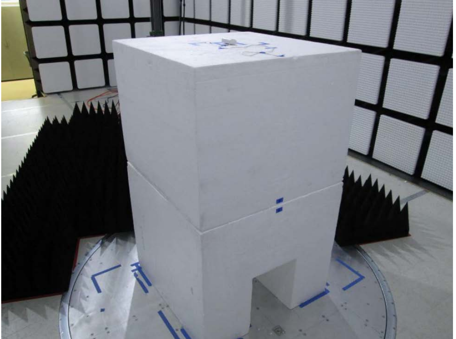
ANT1 Radiated Testing Above 1GHz - Back View
