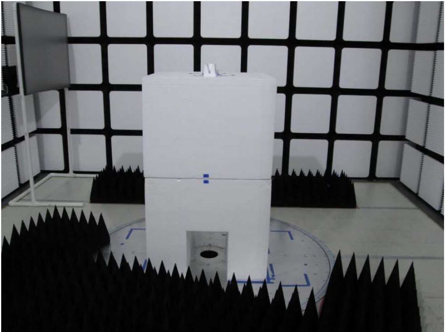
ANT2 Radiated Testing Above 1GHz - Front View
