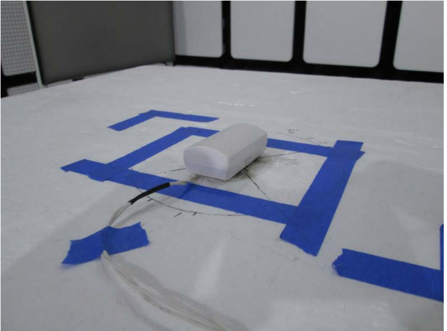
XYZ Orientation Setup - X Axis
