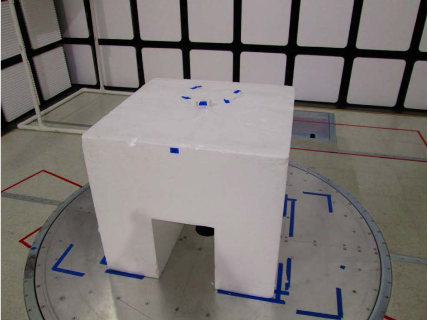
ANT2 Radiated Testing Below 1GHz - Front View
