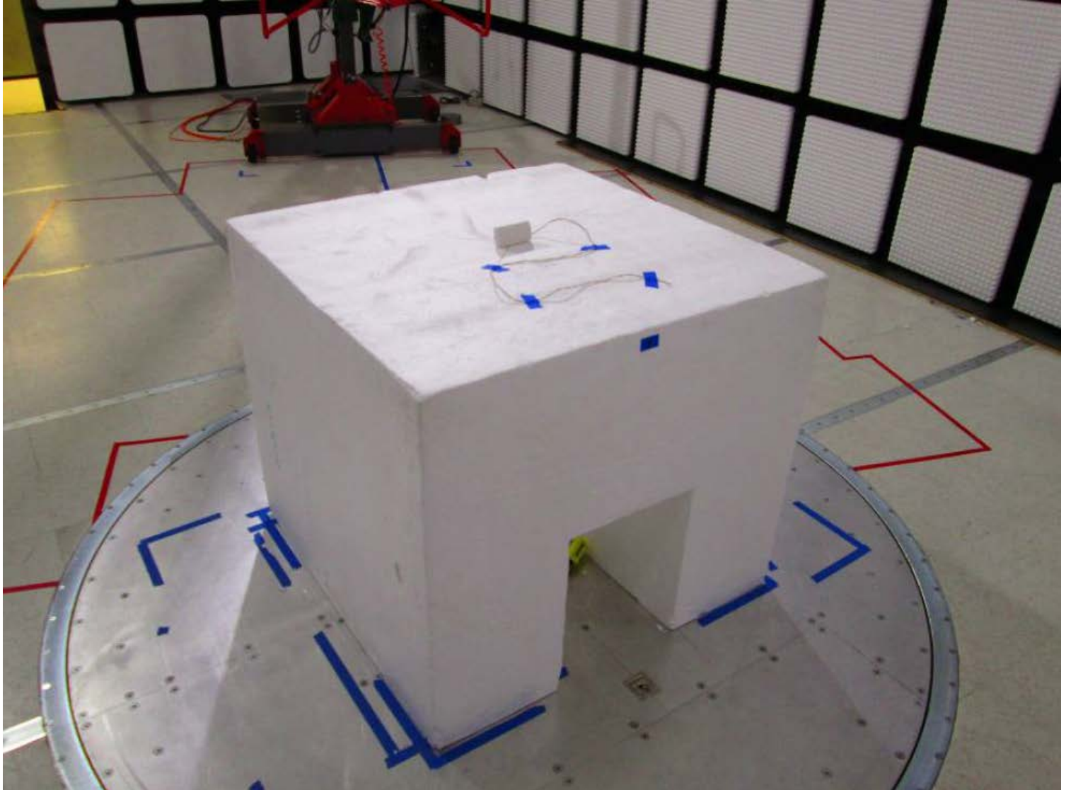
ANT2 Radiated Testing Below 1GHz - Back View
