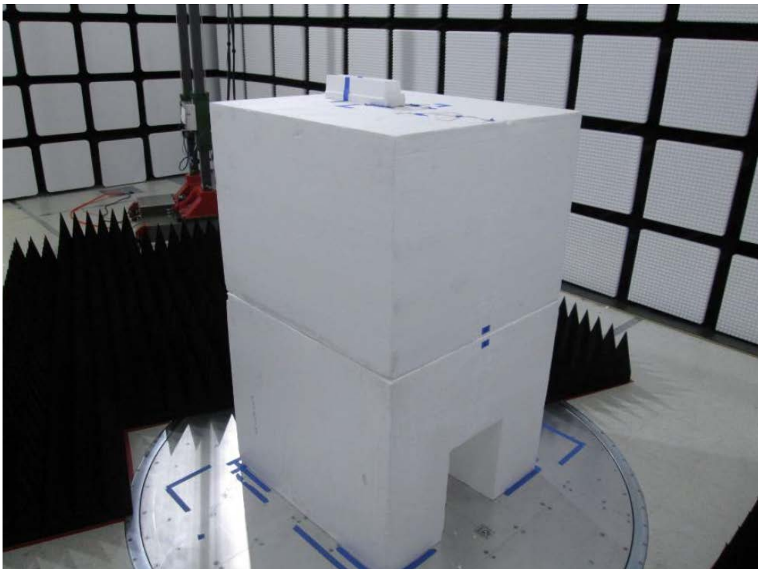
ANT2 Radiated Testing Above 1GHz - Back View
