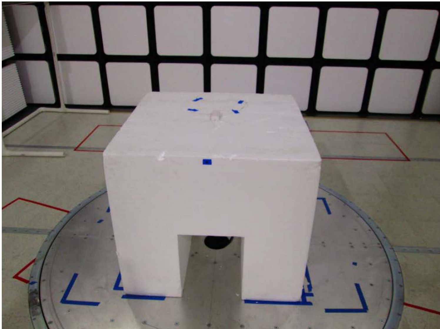
ANT1 Radiated Testing Below 1GHz - Front View
