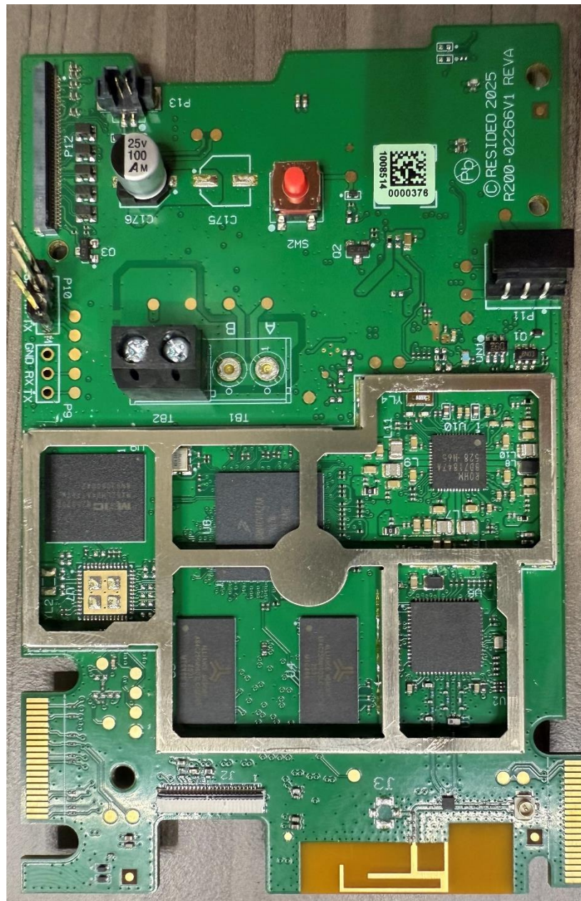
Figure 2 PCB top view without metal shield
