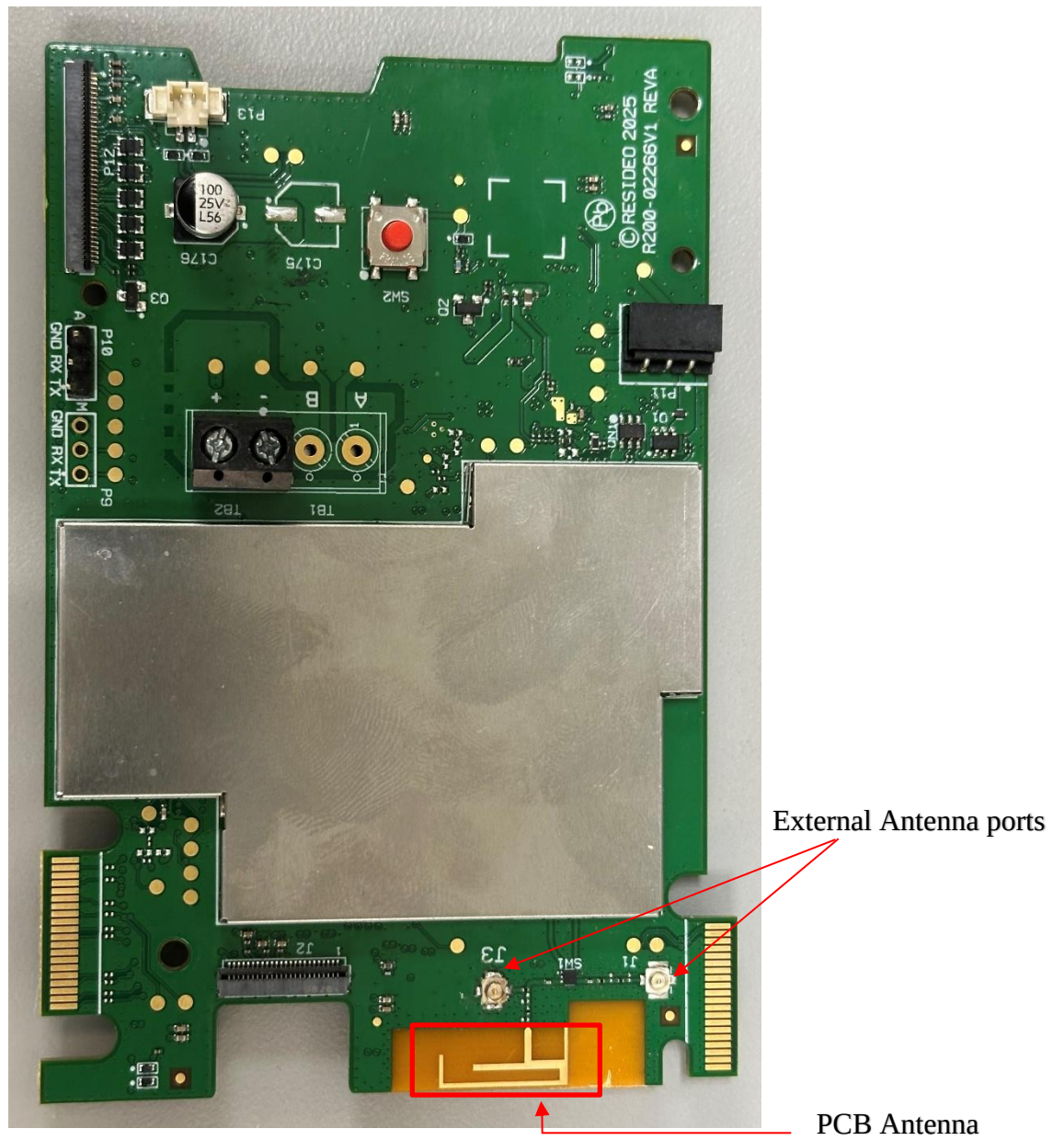
Figure 1 Top view
