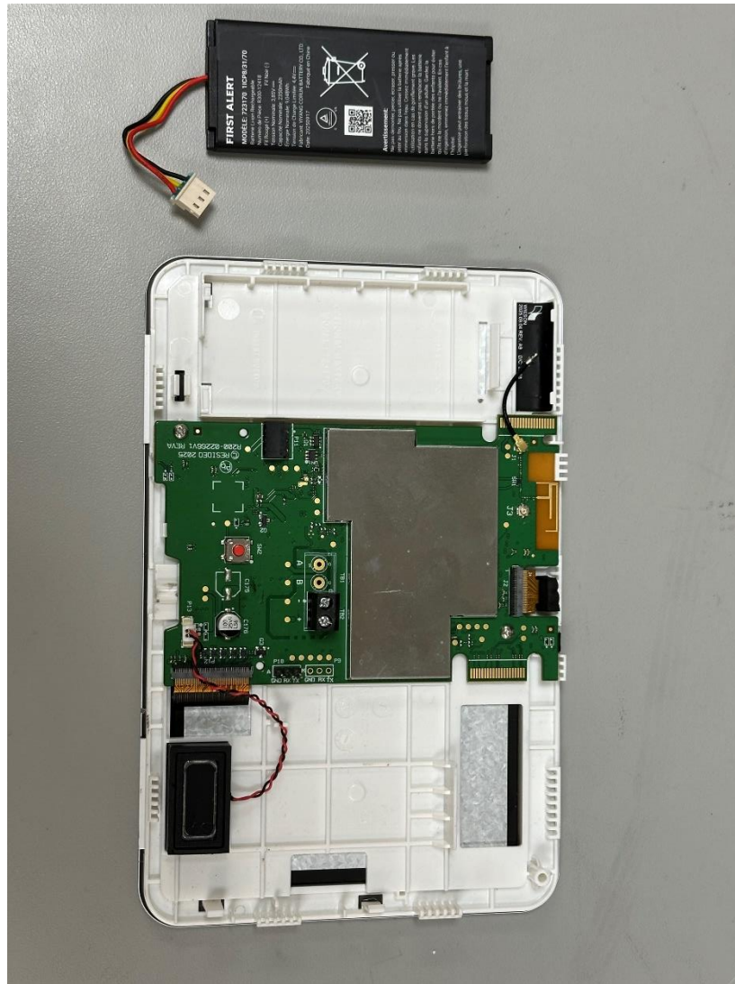
Figure 7 PCB inside cover without battery
