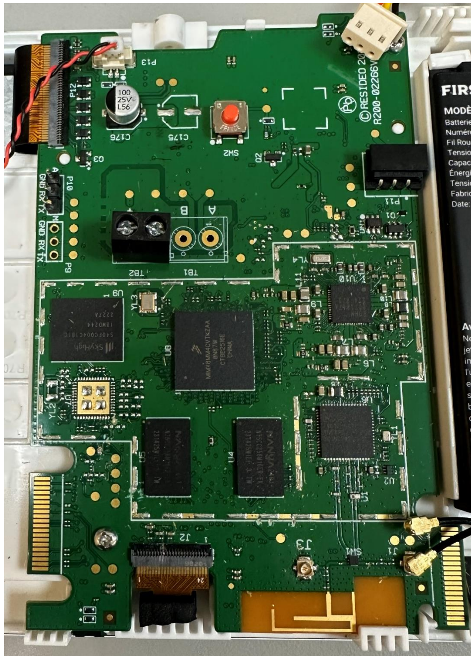
Figure 3 PCB top view without the cross bars
