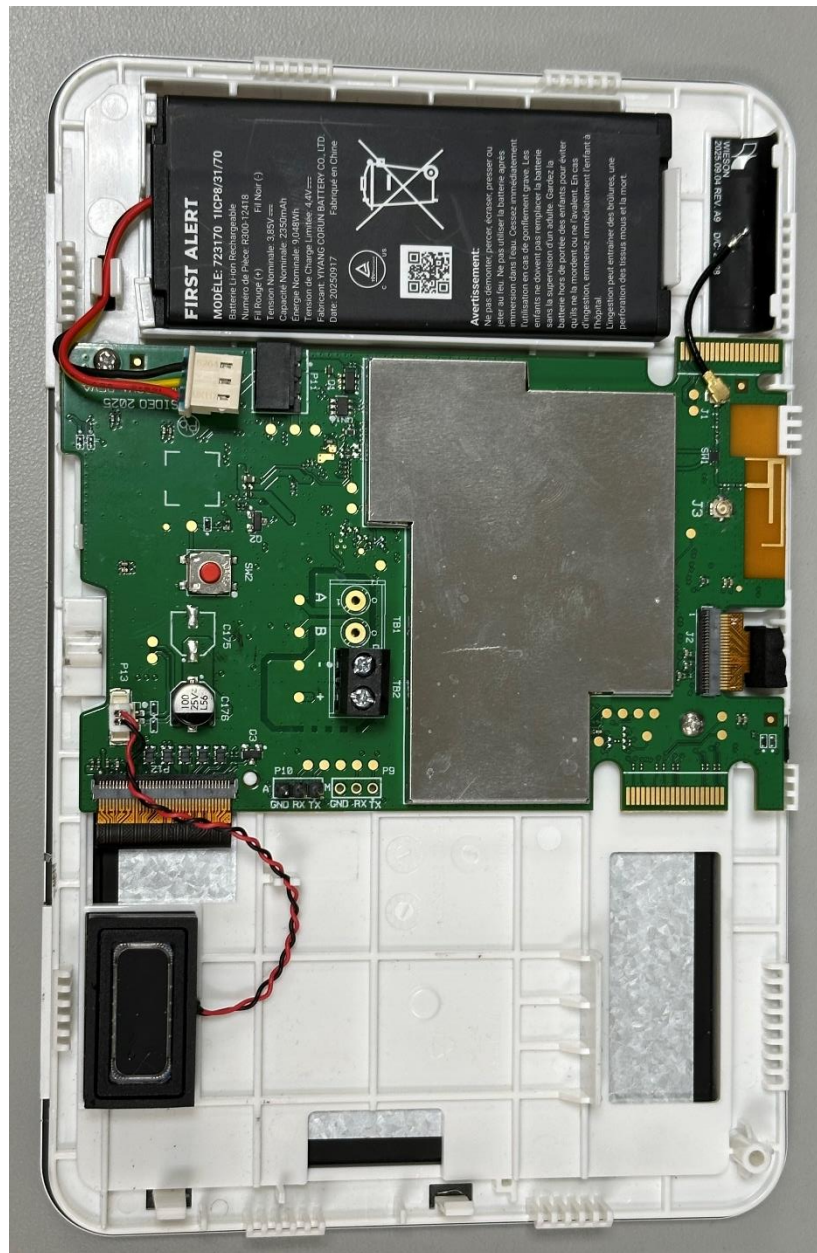
Figure 6 PCB inside cover with battery
