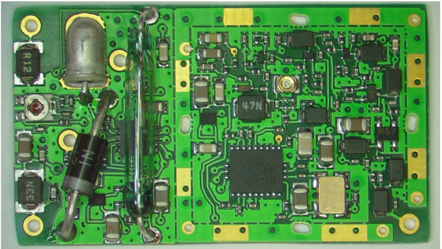
Printed Circuit Board Front photo without shield
