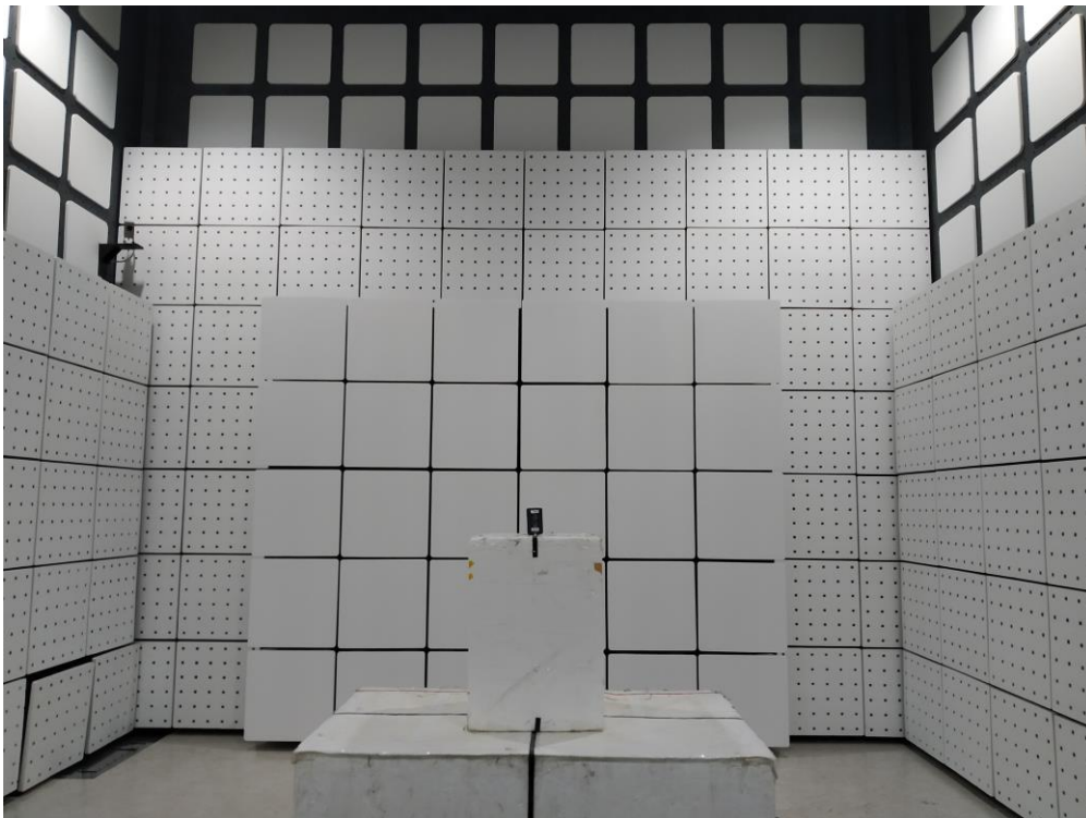
Photograph 2: Set-up for Radiated Emissions (Front View 2)
