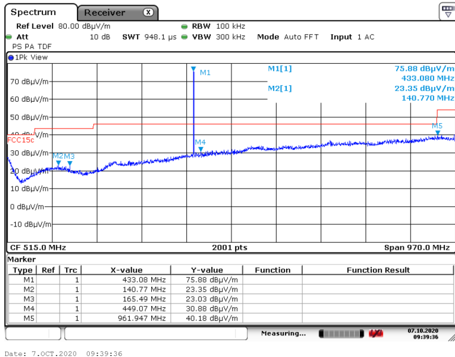
Pre-scan Plot of the emissions in the range 30 – 1000 MHz, Antenna Vertical, EUT @ 433.3 MHz
