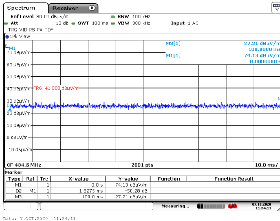
Plot 4: RF On Time for data transfer (position info) in a 100ms period, as measured on a spectrum analyzer.
