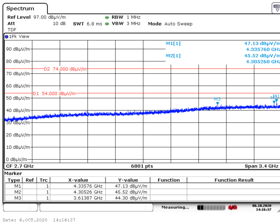
Plot of the emissions in the range 1G – 4.5 GHz, Antenna Vertical, EUT @ 433.3 MHz
