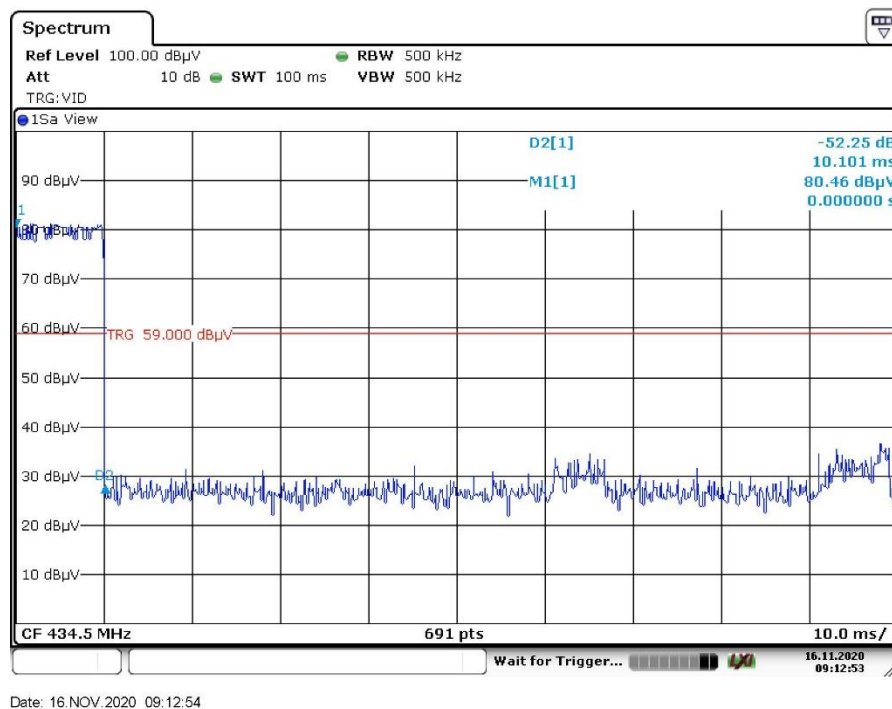
Plot 5: RF On Time for Activity communication in a 100ms period, as measured on a spectrum analyzer.
