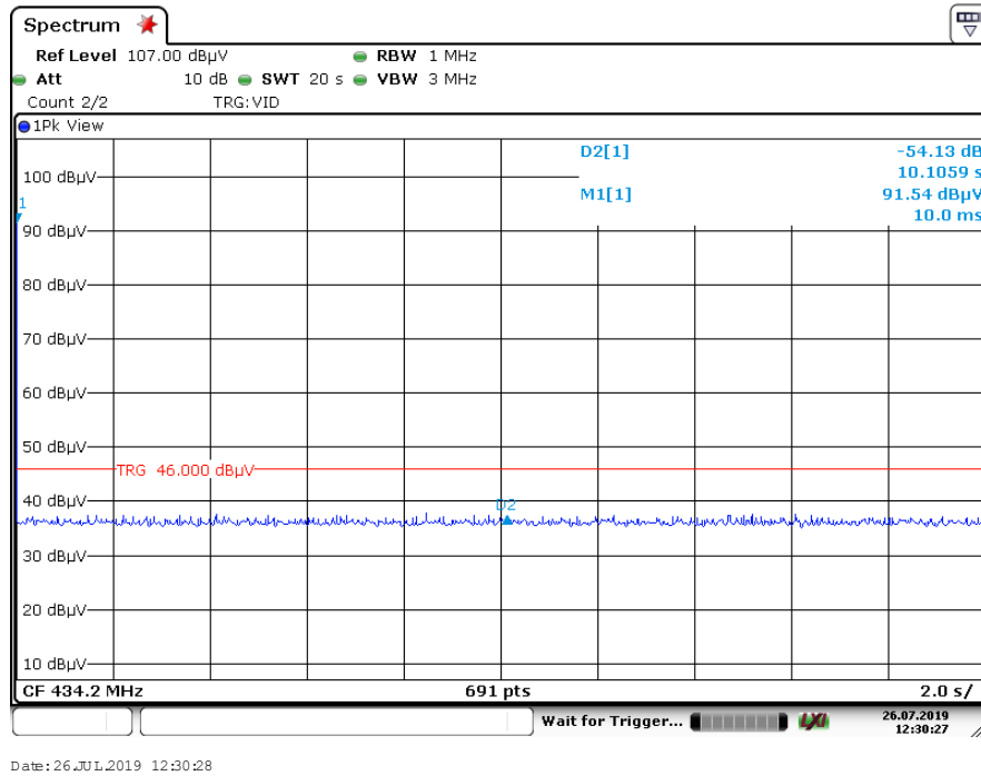
Plot 6: RF Off Time as measured on a spectrum analyzer
