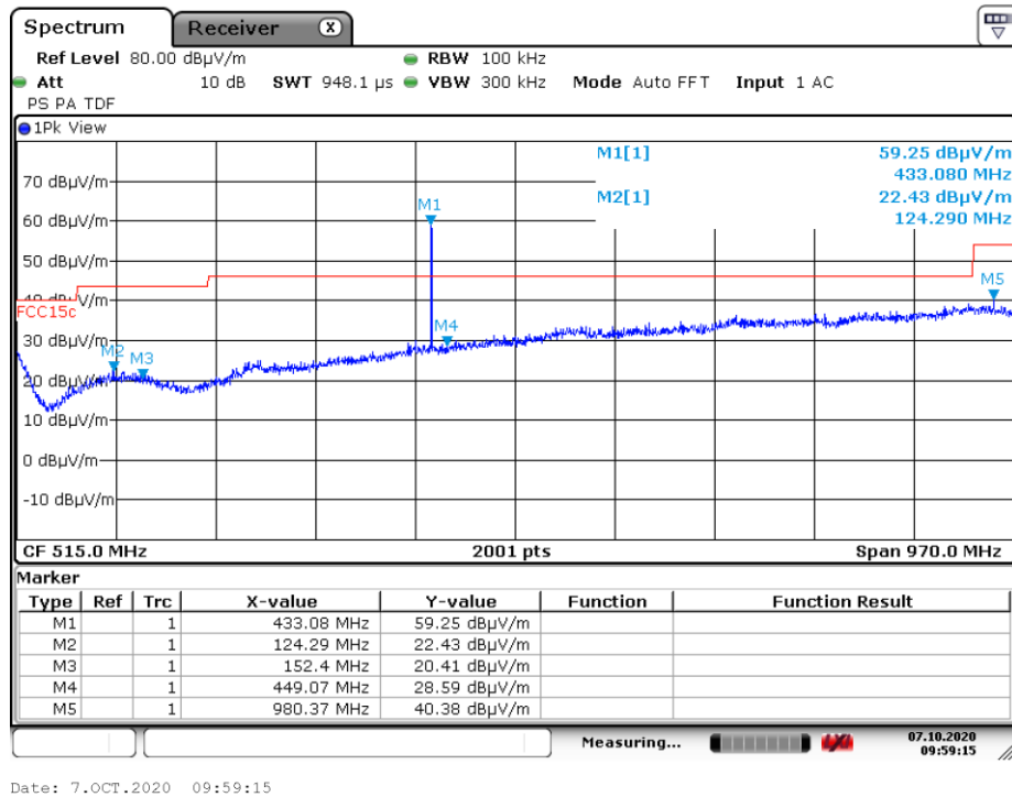
Pre-scan Plot of the emissions in the range 30 – 1000 MHz, Antenna Vertical, EUT Z pos @ 434.0 MHz
